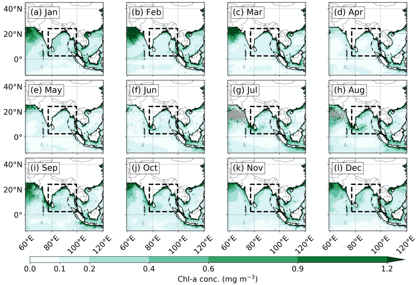
Figure 3: Monthly chlorophyll- a concentration climatology measured from MODIS-Aqua at 4 km horizontal resolution from January to December. The BoB domain is outlined by a black dashed box (77–99.5° E, 2.5–24° N), which shows the location of the imposed annual cycle of chlorophyll concentration for the perturbation simulation. Missing data is shown in grey.
