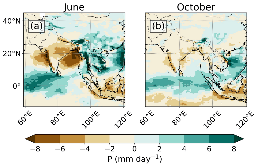
Figure 13: Model bias of precipitation rate for: (a) June; (b) October. Bias calculated as the monthly 29-year average precipitation rate from the control run minus the monthly climatological precipitation rate observed from TRMM satellite.
