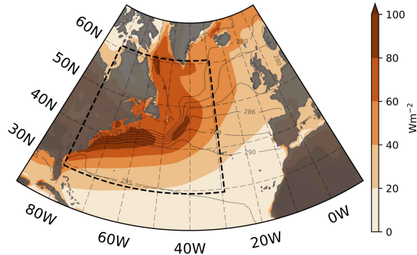
Figure 1. Temporal standard deviation of F (shading) and SST winter climatology (contours, every 2K from 280K to 290K, every 5K otherwise). The area within the dashed box ( 30\text{--}60^\circ\text{N} , 30\text{--}79.5^\circ\text{W} ) corresponds to the region of the N. Atlantic considered in the next sections for the computation of spatial averages.
