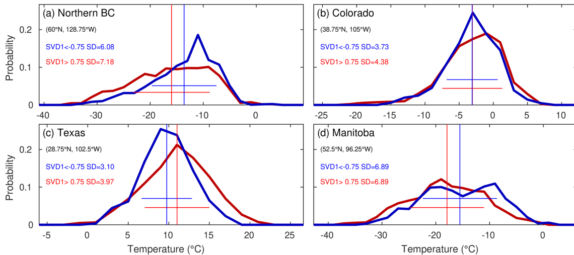
Figure 11. Probability density of temperature at four reference locations (indicated with letters in Fig. 10). Statistics are reported separately for SVD1 SST > 0.75 (red) and SVD1 SST < -0.75 (blue). The standard deviation (SD) is reported in each panel and illustrated with horizontal lines as intervals of 2 SD. The means of the distributions are indicated with vertical lines.
