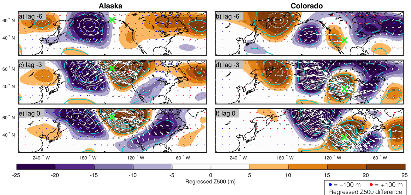
Figure 9. One-point regression maps of Z500 anomalies (color shading) with respect to reference SAT time series over (a, c, e) Alaska (61° N, 150° W) and (b, d, f) Colorado (39° N, 105° W). The corresponding correlation is superimposed with cyan contours (increments of 0.2). The regression is performed separately for years when SVD1_{SST} \geq 0.75 and SVD1_{SST} \leq -0.75 (indicated with blue crosses and circles in Fig. 1, respectively), and the average of the two patterns is shown in this figure. The reference SAT time series for the positive and negative phases are normalized independently before carrying out the regression. Differences between the SVD1_{SST} \geq 0.75 and SVD1_{SST} \leq -0.75 patterns that are significant at the \alpha_{FDR} = 0.1 significance level are shown with blue dots for negative differences and red dots for positive differences. The dots are scaled according to the magnitude of the difference. For reference, the dots illustrated in the legend represent a difference of 100 m. The wave-activity flux (Takaya and Nakamura, 2001) evaluated with the regressed Z500 anomalies is shown with white arrows with a distance of 1° corresponding to a flux of 2/3 \text{ m}^2 \text{ s}^{-2} .
