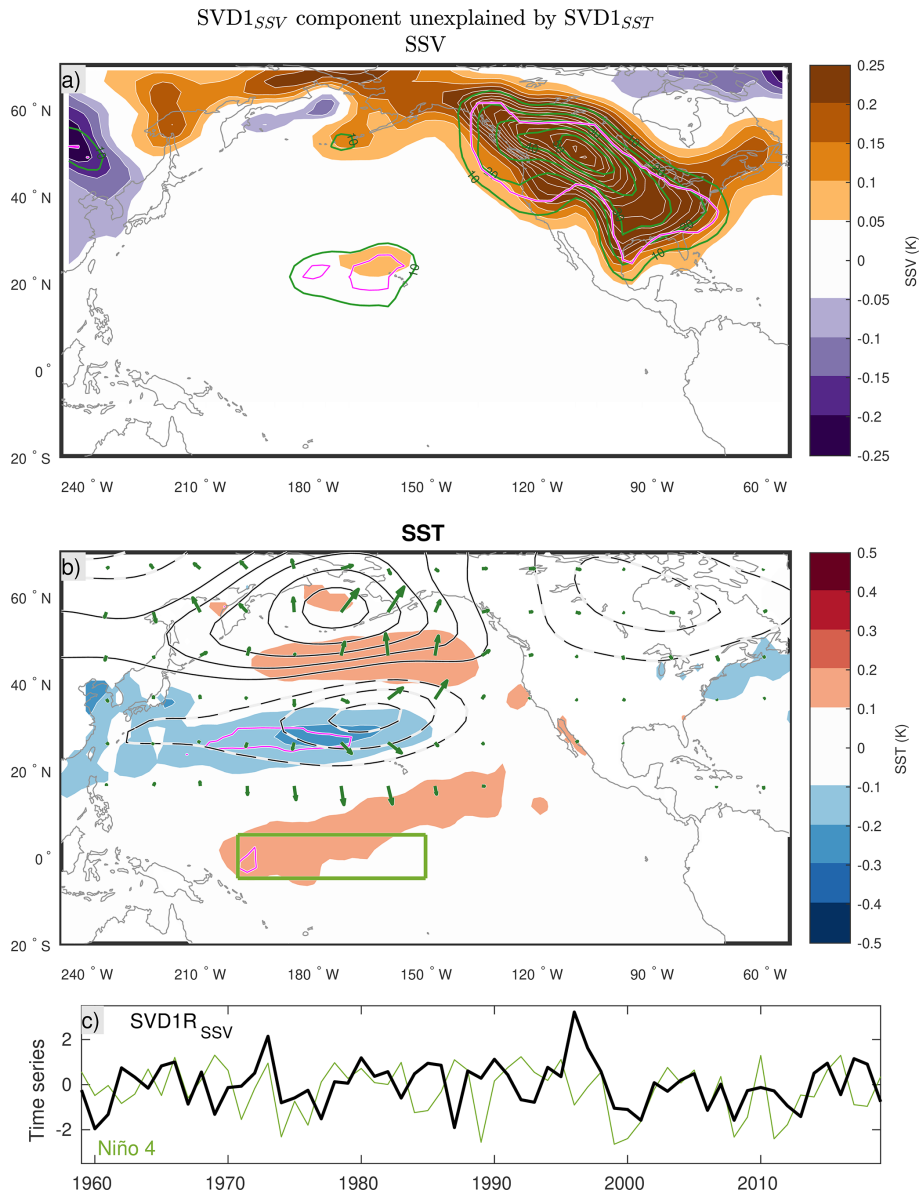
Figure 12. Subseasonal (10–60 d) SAT variability (SSV) (a) and SST (b) are regressed on the component of SVD1 SSV that is not correlated with SVD1 SST (SVD1 RSSV ). Regions that are statistically significant at the \alpha_{FDR} = 0.1 significance level are contoured in magenta. The green contours superimposed on panel (a) indicate the fraction of interannual SSV variability explained by this mode with 10% contour intervals (solid and dashed contours are used for positive and negative values, respectively; the 0 line is omitted). The regression of Z500 (contours, 5 m intervals with solid and dashed black contours for positive and negative anomalies) is also shown in panel (b) . The corresponding wave-activity fluxes (Takaya and Nakamura, 2001) are shown with green arrows. A distance of 1° corresponds to a flux of 0.125 m 2 s -2 . The SVD1 RSSV time series, as well as the Niño 4 index, are shown in panel (c) and the region used to compute this index is illustrated over the SST pattern in panel (b) .
