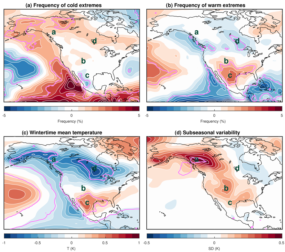
Figure 10. Regression of (a) frequency of cold extremes, (b) frequency of warm extremes, (c) winter-mean SAT, and (d) subseasonal SAT variability onto the SVD1 SST index. Values that are statistically significant at the \alpha_{FDR} = 0.1 significance level are contoured in magenta.
