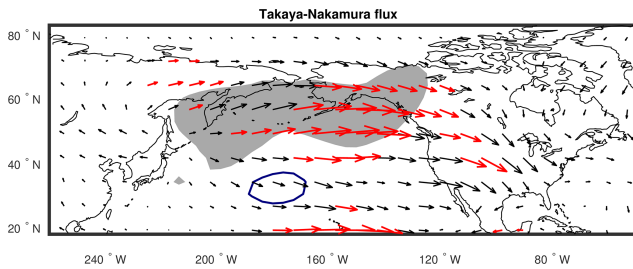
Figure 7. The wave-activity flux (Takaya and Nakamura, 2001) of 10–60 d band-pass-filtered eddies at 300 hPa regressed onto the SVD1_{SSV} time series. The anomalous flux whose meridional or vertical component is significant at the \alpha_{FDR} = 0.1 significance level, assessed with a t test on the correlation coefficients, is shown in red. A distance of 1^\circ corresponds to a flux of 0.67 \text{ m}^2 \text{ s}^{-2} . Regions where CP and CK are larger than 3 \times 10^4 \text{ J m}^{-2} \text{ d}^{-1} are denoted with gray shading and a blue contour, respectively (see Fig. 2c–d).
