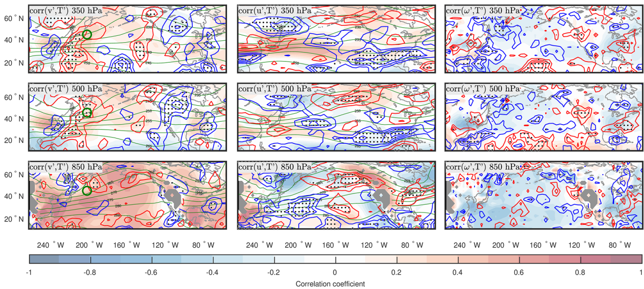
Figure 6. Maps of climatological correlation coefficients (color shading) between v' and T' (left), between u' and T' (center), and between \omega' and T' (right). The respective composite differences between winters of SVD1_{SSV} > 0.75 and SVD1_{SSV} < -0.75 are superimposed with blue and red contours with an interval of 0.1 for negative and positive differences, respectively. For reference, the temperature climatology is shown with green lines. Composite differences that are significant at the \alpha_{FDR} = 0.1 significance level are dotted. The green circle in the left panels indicates the reference location for Fig. 8.
