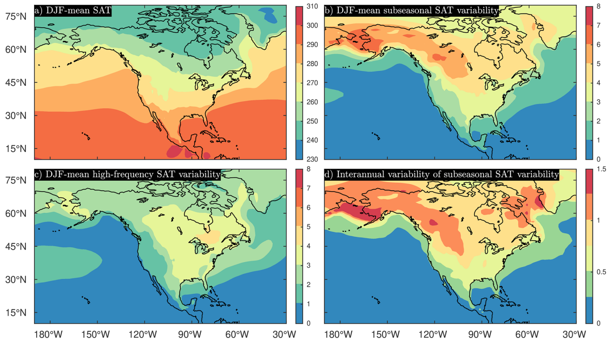
Figure 1. Climatological features of SAT variability (1958–2019). The (a) DJF-mean SAT, (b) DJF-mean subseasonal (10–60 d) SAT variability, or SSV, (c) DJF-mean high-frequency (2–8 d) SAT variability, and (d) interannual modulations of subseasonal SAT variability are shown with color shadings. All variables are in units of K. Variability is illustrated with the standard deviation.
