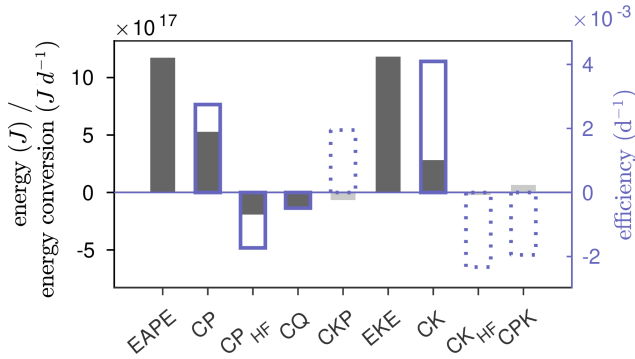
Figure 4. The energetics of subseasonal eddies are integrated over the North Pacific (10–87.5° N, 120° E–55° W) and regressed onto SVD1 SSST . Raw changes in energy and sources/sinks are shown with solid bars. Significant values are shown with a darker shade of gray. Blue boxes indicate changes in the efficiency with significant changes indicated with solid borders. Quantities shown include eddy available potential energy (EAPE), baroclinic energy conversion (CP), high-frequency eddy baroclinic feedback (CP HF ), diabatic feedback (CQ), transfers from EKE to EAPE (CKP), eddy kinetic energy (EKE), barotropic energy conversion (CK), high-frequency barotropic feedback (CK HF ), and transfers from EAPE to EKE (CPK).
