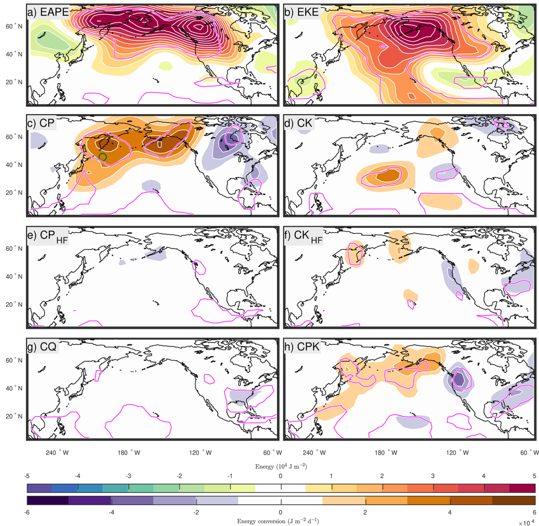
Figure 3. (a) Eddy available potential energy (EAPE), (b) eddy kinetic energy (EKE) of subseasonal eddies and energy sources/sinks (c–h), all regressed onto the SVD1_{SST} index. (c) CP and (d) CK are the baroclinic and barotropic energy conversions, respectively. (e) CP_{HF} and (f) CK_{HF} represent the baroclinic and barotropic high-frequency eddy feedbacks. (g) CQ is the diabatic feedback. (h) CPK represents transfers from EAPE to EKE. Correlations that are statistically significant at the \alpha_{FDR} = 0.1 significance level are contoured in magenta. The green circle in panel (c) indicates the reference location for Fig. 8.
