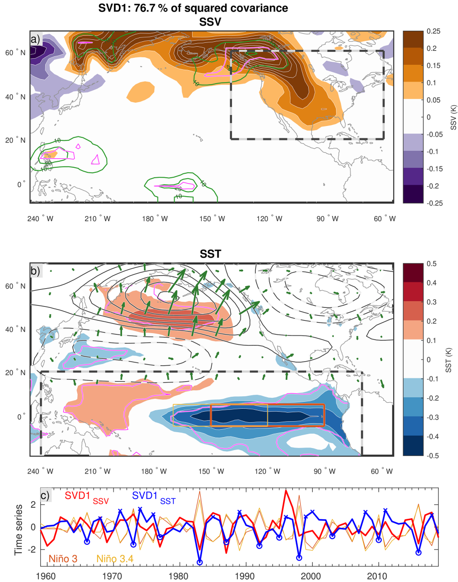
Figure 2. Wintertime anomaly patterns of (a) subseasonal SAT variability (SSV; 10–60 d) and (b) winter-mean SST associated with the dominant mode of covariability (SVD1, corresponding to La Niña) between the two variables (color shadings; anomalies statistically significant at the \alpha_{FDR} = 0.1 significance level are contoured in magenta). The sectors used for the SVD analysis are bounded by bold dashed lines. The green contours superimposed on (a) indicate the fraction of interannual SSV variability explained by this mode with 10% contour intervals (solid and dashed contours are used for positive and negative values, respectively; the 0 line is omitted). Z500 anomalies regressed onto SVD1 SST are superimposed on (b) with black contours (increment of 5 m, solid and dashed for positive and negative anomalies, respectively). The corresponding wave-activity fluxes (Takaya and Nakamura, 2001) are shown with green arrows. A distance of 1^\circ corresponds to a flux of 0.125 \text{ m}^2 \text{ s}^{-2} . (c) Anomaly time series of SSV (SVD1 SSV , red) and SST (SVD1 SST , blue) associated with SVD1. Two Niño indices are superimposed (domains used to compute these indices are illustrated over the SST pattern in panel b).
