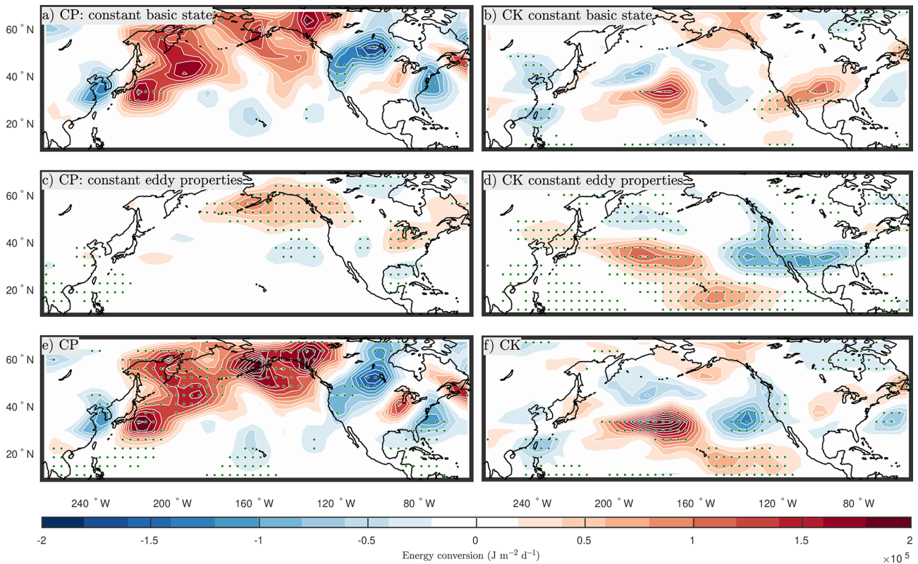
Figure 5. Baroclinic energy conversion (CP; a , c , e ) and barotropic energy conversion (CK; b , d , f ) composite differences between the positive ( \text{SVD1}_{\text{SST}} > 0.75 ) and negative ( \text{SVD1}_{\text{SST}} < -0.75 ) phases of SVD1 (representing La Niña) are calculated by keeping either the background flow properties ( a , b ) or eddy properties ( c , d ) constant every year. For reference, the composite difference when both eddy properties and the basic state can change from year to year is shown in panels ( e ) and ( f ). Composite differences that are significant at the \alpha_{\text{FDR}} = 0.1 significance level are dotted.
