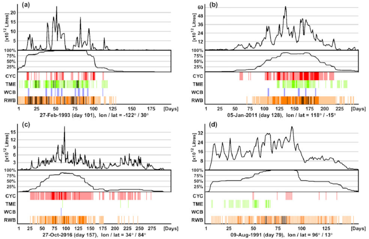
Figure 7 Each of the four panels depicts an exemplary patch, labelled by the respective panel's letter in Fig. 6. Time periods on the abscissa span from the earliest (day 1) to the latest date (e.g. day 170 in panel A) of all extreme seasons of the grid points that compose each patch. The upper part of each panel shows time series of daily precipitation, accumulated for all grid points that compose the patch. Given that the patch period on the abscissa is composed by non-identical extreme seasons per grid point, the time series in the middle of each panel shows the fraction of the extreme season patch that includes the respective day. The lower part of the panel marks each day by a vertical line if a weather system overlapped with the patch (see text): red for cyclones, blue for WCBs, green for TMEs and brown for RWB. Central date and average latitude/longitude of each of the four patch is shown under the panels.
