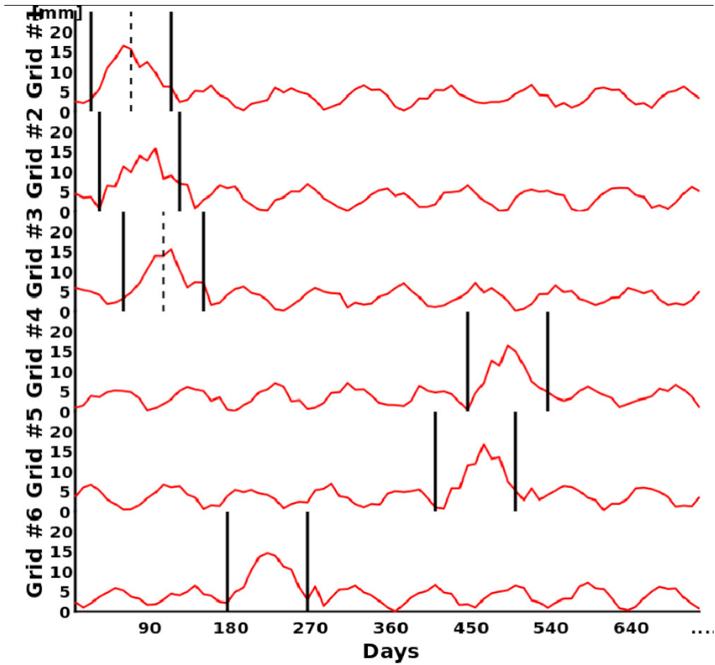
825 Figure 1 Methodological approach in an idealized one-dimensional grid to identify spatial coherences of extreme seasons. Red lines show precipitation time series per grid point, vertical black lines delineate the identified extreme season per grid point and vertical dotted lines depict their central date (only for two seasons, to be used as an example in text).
