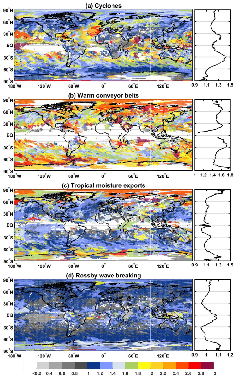
995 Figure 11 All extreme wet season patches are coloured according to their overlapping frequency ratios with specific weather systems (relative to the climatology). Panels in the right column show the latitudinal distribution of the overlapping ratios, as zonal averages within \pm 7.5^\circ latitude. Patches may overlap between each other; to allow higher visibility for patches with highest ratios, the overlay of the patches in all panels started from the patch with the lowest ratio.
