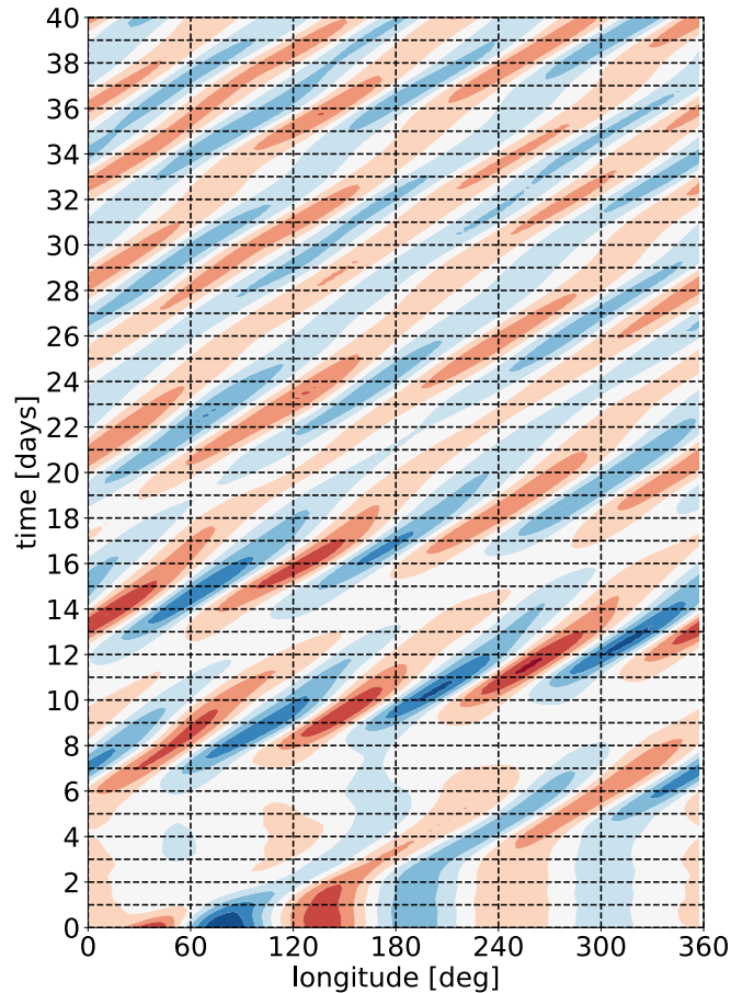
Figure 1. Development of a barotropically unstable initial state for a model set-up with a strong narrow jet at 45^{\circ}\text{N} . The plot shows a Hovmoeller diagram of the meridional wind component of the transient part of the flow, v' = v - \bar{v} , averaged over 30 - 60^{\circ}\text{N} .
