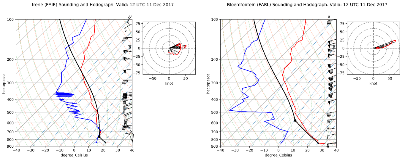
Figure 8: Irene (FAIR) upper-air sounding at 1200 UTC on 11 December 2017. This is used to approximate atmospheric conditions over VAM. The Bram Fischer International Airport (FABL) upper-air sounding at 1200 UTC is also included and indicates upstream mid-level winds of about 45 knots. Hodographs are included for each sounding, indicating wind shear between the surface and 10 km above ground level.
