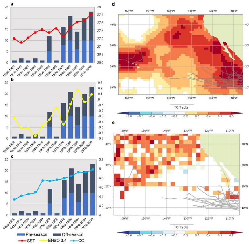
326 Figure 3. Decadal TC counts for the EP off-seasons and decadal average SSTs (a), decadal TC counts for 327 the EP off-seasons and decadal average ENSO 3.4 (b), decadal TC counts for the EP off-seasons and 328 decadal average Correlation between Time and Dec-May averaged CC (c), correlation between Time and 329 Dec-May averaged SST (C°) and the off-season TC tracks for the 1900-2019 period (d) and correlation 330 between Time and Dec-May averaged CC (oktas) and the off-season TC tracks for the 1900-2019 period.
