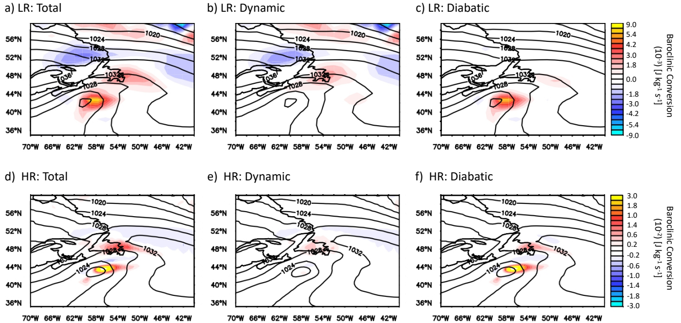
Figure 4. Vertically-averaged baroclinic conversion between 850 hPa and 300 hPa (shaded) and mean sea level pressure (contoured) at 18 UTC 29 September 2016 (T + 18 h from hindcast initiation at 00 UTC 29 September 2016) for ARPEGE hindcasts. a–c) ARPEGE-LR hindcast and d–f) ARPEGE-HR hindcast. a,d) total (dynamic + diabatic) baroclinic conversion; b,e) baroclinic conversion from dynamical processes; c,f) baroclinic conversion from diabatic processes. The colour scales refer to each row.
