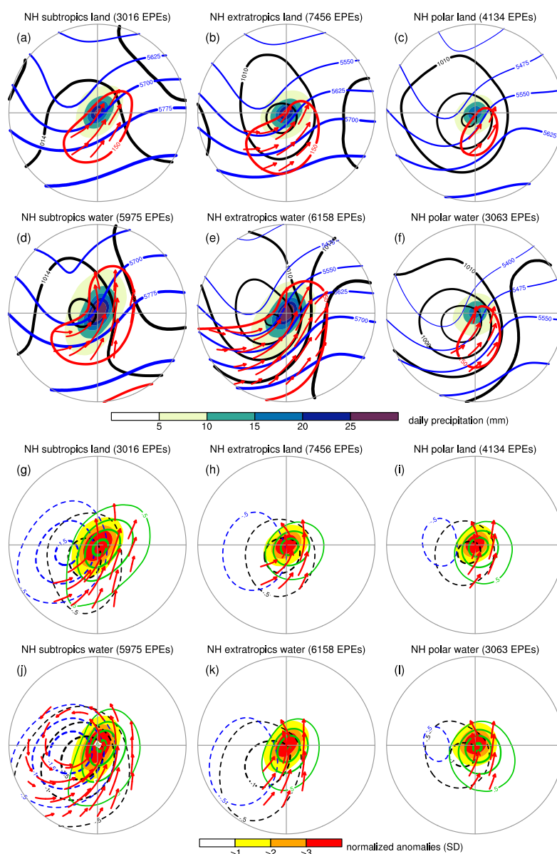
Figure 9. Composites of the tropospheric circulation for EPEs linked to combined Rossby wave breaking and intense moisture transport with (a-f) daily means and (g-l) normalized anomalies. The composites have a radius of 2000 km and are centred on the mass-weighted centres of the EPEs for subtropical (20°–40° N), extratropical (40°–60° N), and polar (60°–80° N) regions in the Northern Hemisphere over (first and third row) land and (second and fourth row) water during the period of 1979–2018. Shading in (a)–(f) shows daily precipitation (mm) and in (g)–(l) their normalized anomalies (SD). The contour lines in (a)–(f) show daily means of the 500-hPa geopotential height (gpm, in blue), mean sea level pressure (hPa; in black), and the IVT magnitude (150 kg m −1 s −1 contour in red) with IVT vectors where the IVT magnitude exceeds 150 kg m −1 s −1 . The contour lines in (g)–(l) show normalized anomalies, in colours as in (a)–(f), in standard deviation (SD) for intervals of \pm 0.5 SD starting at \pm 0.5 SD, with only contours for negative values of 500-hPa geopotential height and mean sea level pressure, and for positive values of total column water (in green). Also, in (g)–(l), IVT vectors constructed from their zonal and meridional components, and only displayed where their vector length exceeds 1 SD.
