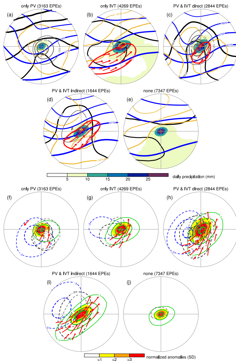
Figure 10. Composites, as in Fig. 9, but for EPEs over subtropical land, for the period of 1979-2016, and for five exclusive categories of EPEs that match (a,f) only PV structures, (b,g) only IVT structures, (c,h) combined PV and IVT structures with a direct PV influence, (d,i) combined PV and IVT structures with only an indirect PV influence, and (e,j) neither PV structures nor IVT structures, as detailed in the text and Table 1. The composites also include in (a)-(e) daily mean contours of QG ascent ( \text{Pa s}^{-1} , in grey) and static stability ( \text{K m}^2 \text{kg}^{-1} , in orange), and in (f)-(j) their normalized anomalies in identical colours, whereby those of static stability are displayed for intervals of -0.25 SD starting at \sim -0.25 SD. Different from Fig. 9, the IVT contours in (a)-(e) correspond to a 200 \text{ kg m}^{-1} \text{s}^{-1} value with IVT vectors shown where the IVT magnitude exceeds 200 \text{ kg m}^{-1} \text{s}^{-1} .
