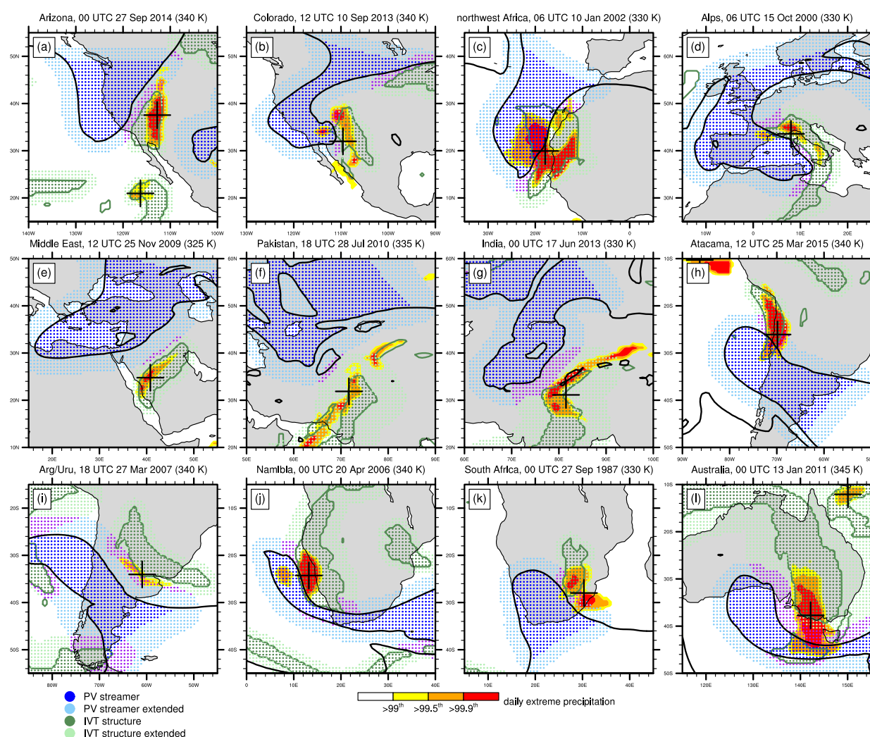
Figure 4. Illustrative cases of extreme precipitation and flooding accompanied by stratospheric PV streamers and IVT structures in (a) Arizona, USA, 00 UTC 27 September 2014, (b) Colorado, USA, 12 UTC 10 September 2013, (c) northwest Africa, 06 UTC 10 January 2002, (d) the Alpine region, 06 UTC 15 October 2000, (e) the Middle East, Jeddah, 12 UTC 25 November 2009, (f) Pakistan, 18 UTC 28 July 2010, (g) India, 00 UTC 17 June 2013, (h) the Atacama Desert in Chile, 12 UTC 25 March 2015, (i) Argentina and Uruguay, 18 UTC 28 March 2007, (j) Namibia, 00 UTC 20 April 2006, (k) South Africa, 00 UTC 27 September 1987, and (l) Australia, 00 UTC 13 January 2011. All meteorological variables and identified objects correspond to those as in Fig. 3b with the exception of extreme precipitation for which only the objects instead of all percentile-exceeding grid points are shown.
