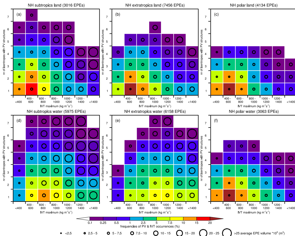
Figure 8. Characteristics of PV and IVT structures, for clusters defined by the number of isentropes with PV structures and the IVT maxima ( \text{kg m}^{-1} \text{s}^{-1} ), with the corresponding average precipitation volumes of the EPEs in the circles as denoted by the legend. As in Fig. 7, the plot is based on EPEs, linked to combined wave breaking and intense moisture transport, for identical regions. The colours of the squares reflect the frequencies (%) of the PV and IVT structures that fall in the corresponding clusters and are relative to the total number of 6-hourly time instances during all EPEs that are linked to combined wave breaking and intense moisture transport.
