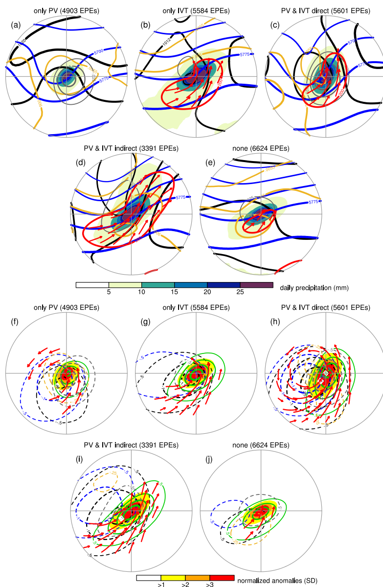
Figure 11. As Figure 10, but for EPEs over subtropical water.
