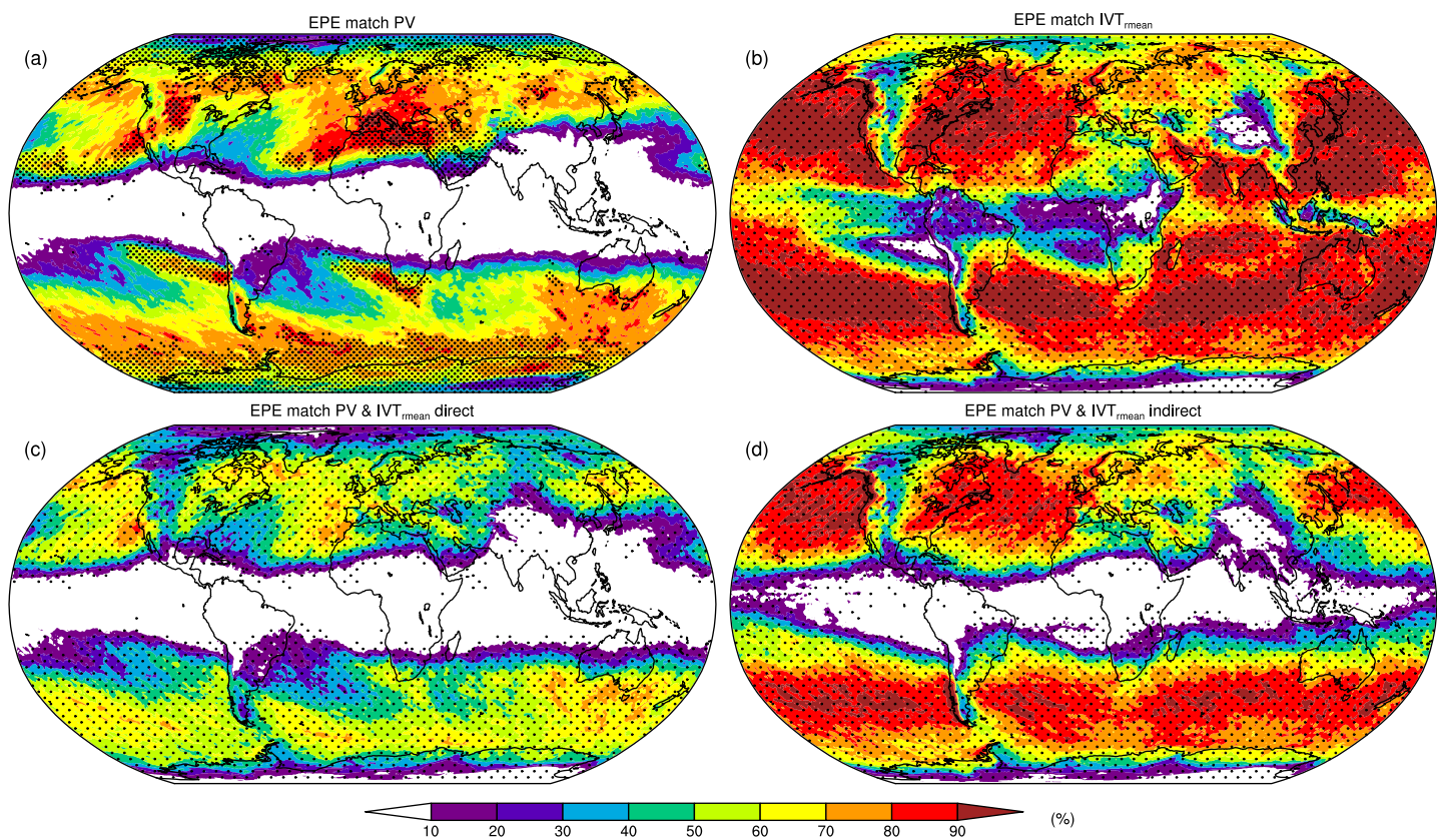
Figure S1. As Fig. 6, but for the IVTfilt form.
