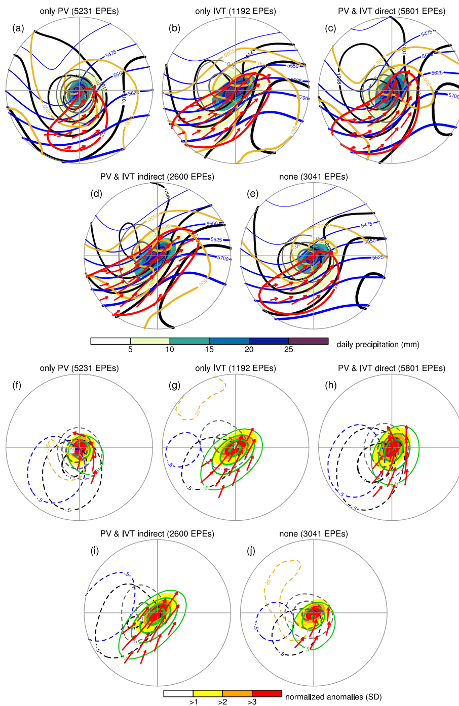
Figure S3. As Fig. 10, but for EPEs over extratropical water.
