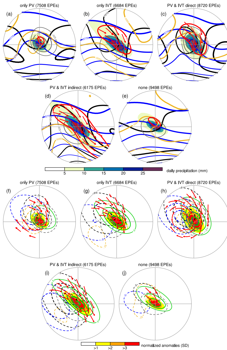
Figure S4. As Fig. 10, but for EPEs in the Southern Hemisphere over subtropical water.
