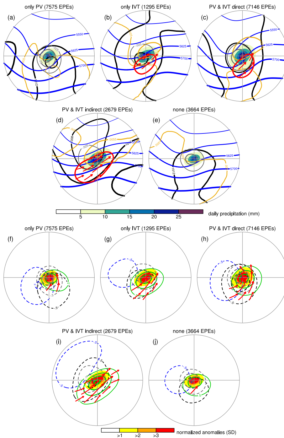
Figure S2. As Fig. 10, but for EPEs over extratropical land.
