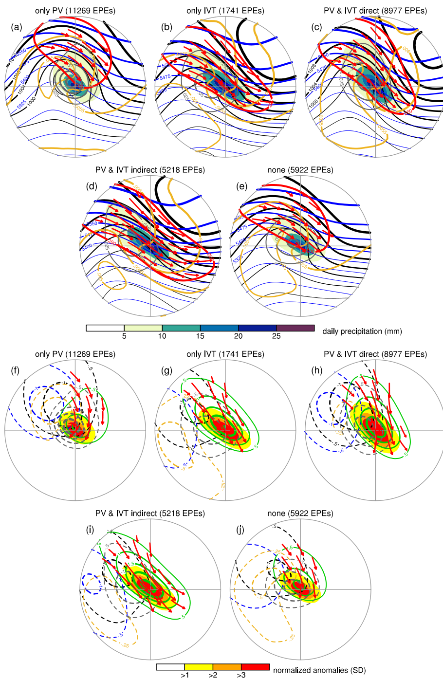
Figure S5. As Fig. 10, but for EPEs in the Southern Hemisphere over extratropical water.
