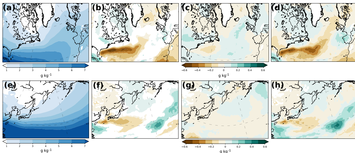
Figure 9. (a) Climatological specific humidity at 850 hPa (shading, \text{g kg}^{-1} ) for the North Atlantic for CNTL. (b) Difference-Statistically significant (>95%) difference of climatological specific humidity between SMTHG and CNTL ( SMTHG-CNTL ). (c,d) As (b) but only considering the dates with separated for specific humidity within (c) or without and outside (d) cyclones being present in the Gulf Stream region a radius of 750 km around a cyclone centre. (e-h) As (a-d), but for the Kuroshio region . The Gulf Stream and Kuroshio regions are marked with a black box, respectively. Panels (c,d,g,h) are scaled such that their sum yields panels (b) and (f), respectively North Pacific .
