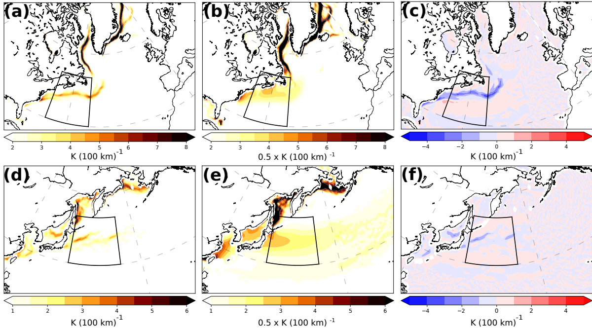
Figure 2. (a) Climatological SST gradient in-for DJF for (a) CNTL [ K (100 \text{ km})^{-1} ], (b) SMTHG [ 0.5 K (100 \text{ km})^{-1} ], and (c) the-difference between-SMTHG and-CNTL- SMTHG-CNTL [K (100 \text{ km})^{-1}] . (d-f) as-As (a-c), but for the North Pacific. The Gulf Stream and Kuroshio regions are marked with a black box, respectively.
