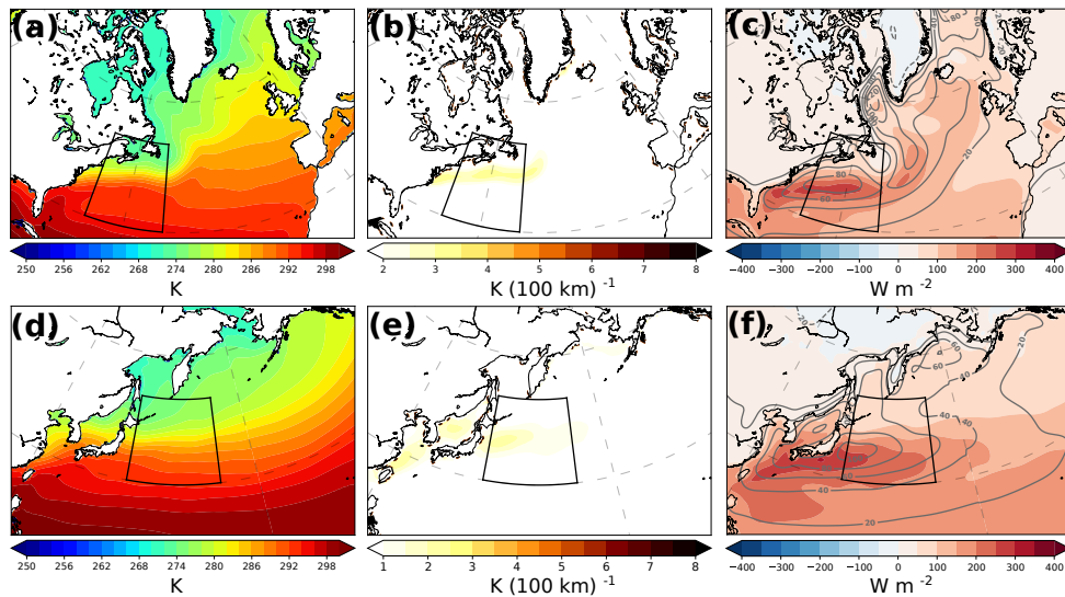
Figure A1. (a) DJF climatology over ERA-Interim period 1982-2000 for (a) the SSTs (K), (b) the SST gradient ( K (100 km)^{-1} ), (c) the latent (shading, W m^{-2} ) and sensible heat fluxes (contours, W m^{-2} ) for the North Atlantic. (d-f) As (a-c), but for the North Pacific. The Gulf Stream and Kuroshio regions are marked with a black box, respectively.
