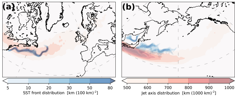
Figure 3. (a) SST front distributions-distribution (blue shading, \text{km of line } (100 \text{ km})^{-2} ) and jet axis distributions-distribution (orange-pale red shading, \text{km of jet axis line } (1000 \text{ km})^{-2} ) for the North Atlantic. (b) as-As (a), but for the North Pacific
