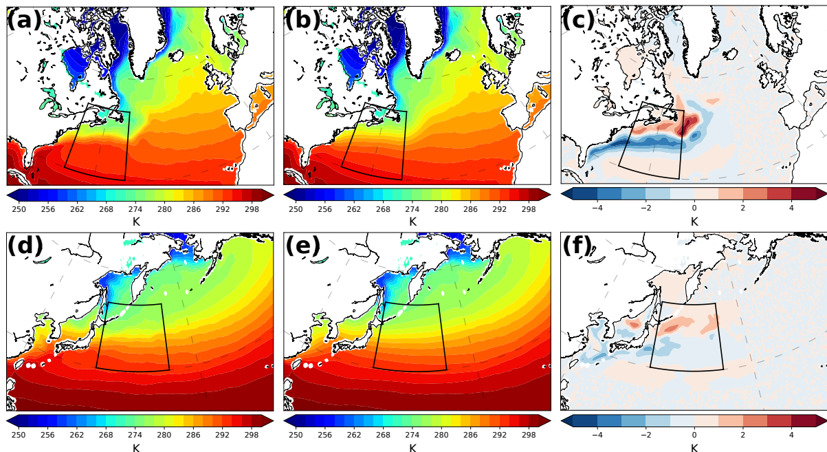
Figure 1. (a) Climatological SSTs in SST for DJF for (a) CNTL, (b) SMTHG, and (c) the difference between SMTHG and CNTL ( \text{SMTHG}-\text{CNTL} [K]). (d-f) as As (a-c), but for the North Pacific. The Gulf Stream and Kuroshio regions are marked with a black box, respectively.
