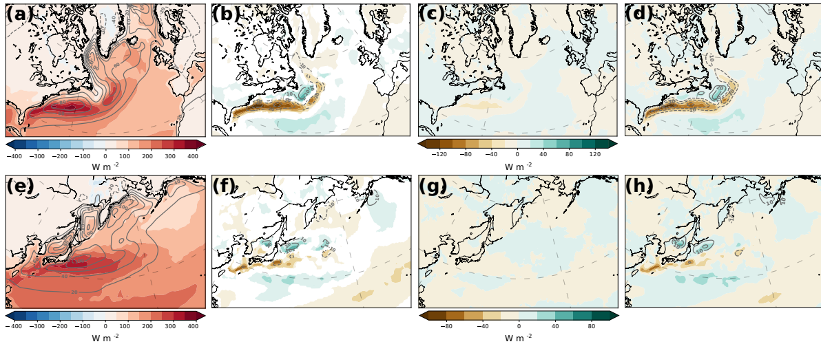
Figure 7. (a) Climatological latent (shading, \text{W m}^{-2} ) and sensible heat fluxes (contours, \text{W m}^{-2} ) for the North Atlantic for CNTL. (b) Difference-Statistically significant (>95%) difference of the heat fluxes-flux climatologies between SMTHG and CNTL ( SMTHG-CNTL ) for latent (shading) and sensible heat fluxes (grey contours, interval: 10 \text{ W m}^{-2} , zero contour omitted). (c,d) As (b) , but only considering the dates with separated for fluxes within (c) or without and outside (d) cyclones present in the Gulf Stream region a radius of 750 km around a cyclone centre. (e-h) As (a-d), but for the Kuroshio region. The Gulf Stream and Kuroshio regions are marked with a black box, respectively. Panels (c,d,g,h) are scaled such that their sum yields panels (b) and (f), respectively North Pacific.
