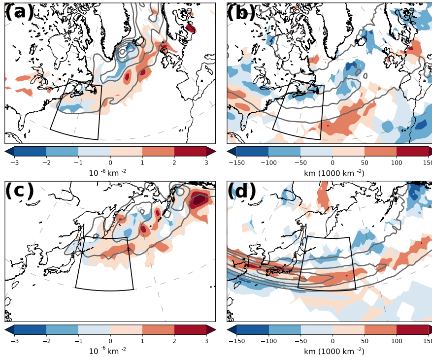
Figure 4. (a) Difference-Statistically significant (>95%, based on the chi-square test) difference in climatological cyclone density (SMTHG-CNTL, shading, 10^{-6} \text{ km}^{-2} ) and climatological cyclone density for CNTL (contours, first contour: 6 \cdot 10^{-6} \text{ km}^{-2} , interval 3 \cdot 10^{-6} \text{ km}^{-2} ). (b) Difference-Statistically significant (>95%, based on the chi-square test) difference in climatological jet stream density (SMTHG-CNTL, shading, km of jet axis line (1000 \text{ km})^{-2} ) and climatological jet stream density for CNTL (contours, first contour: 400 km of jet axis line (1000 \text{ km})^{-2} , interval: 200 km of jet axis line (1000 \text{ km})^{-2} ). (c,d) As (a,b), but for the North Pacific.
