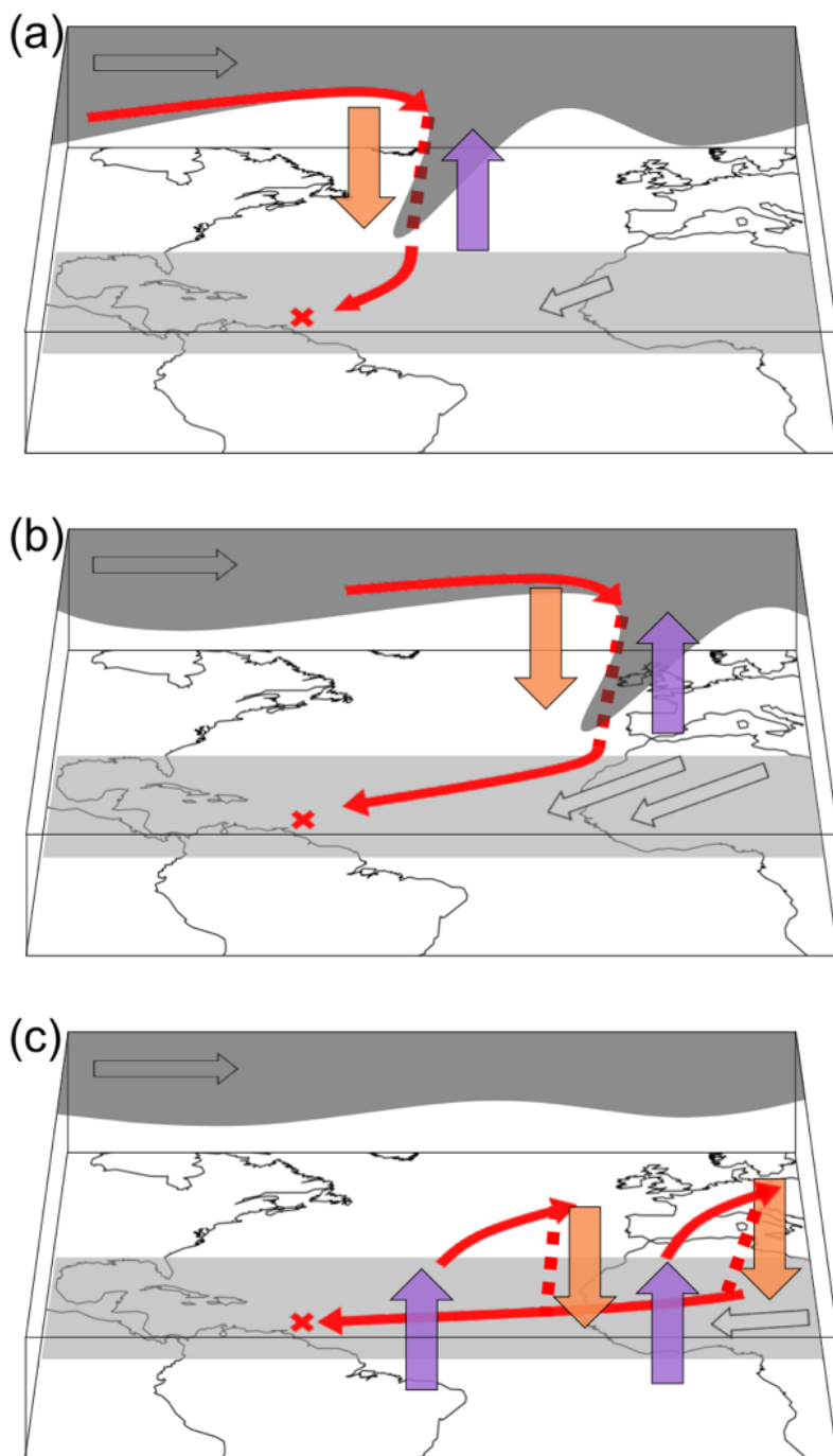
Figure 2: Three-dimensional schematic of the three flow regimes for air parcels arriving in the sub-cloud layer ( p \geq 940 hPa) in Barbados. The extratropical dry intrusion regime is shown in (a), the extratropical trade wind regime in (b), and the tropical regime in (c). The upper-level westerly flow (e.g. on the 310 K isentrope) is indicated with the dark grey surface, the low-level trade wind flow (900-1000 hPa) with the light grey surface, strong descending motion is shown by orange arrows, strong ascending motion is shown by violet arrows, the red line indicates the air parcels' typical trajectory in each regime with dashed red representing rapid descent.
