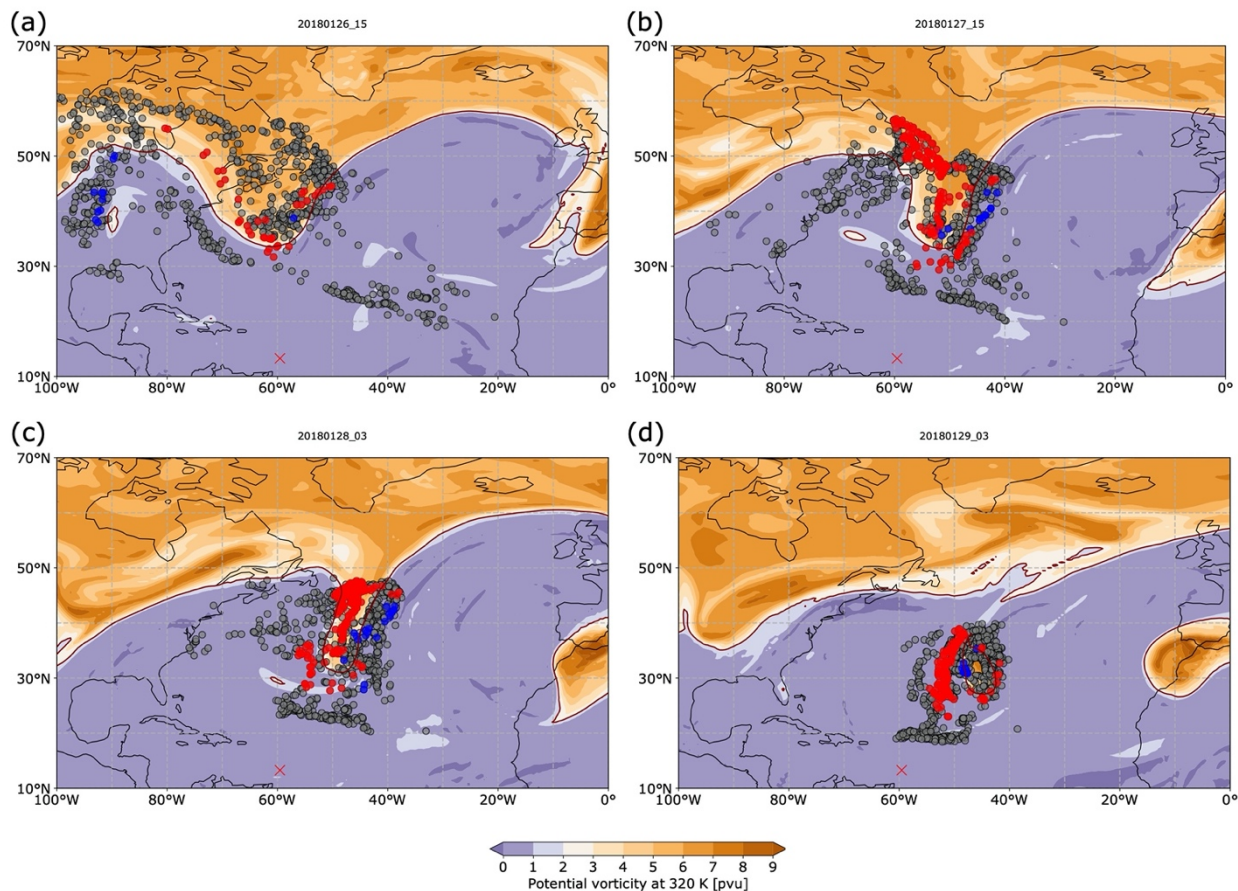
990 Figure 13: The same as Fig. 12 but from 26-29 January 2018, and with air parcels that reach Barbados between 1-4 February. The air parcels that experience rapid ascent ( <-300 \text{ hPa}(2\text{d})^{-1} ) or descent ( >300 \text{ hPa}(2\text{d})^{-1} ) centred at the time shown in the figure are highlighted in blue respectively red. An animation illustrating the 3 hourly evolution of the large-scale flow fields in the period 26 January to 4 February 2018 is provided as Supplementary material S3.
