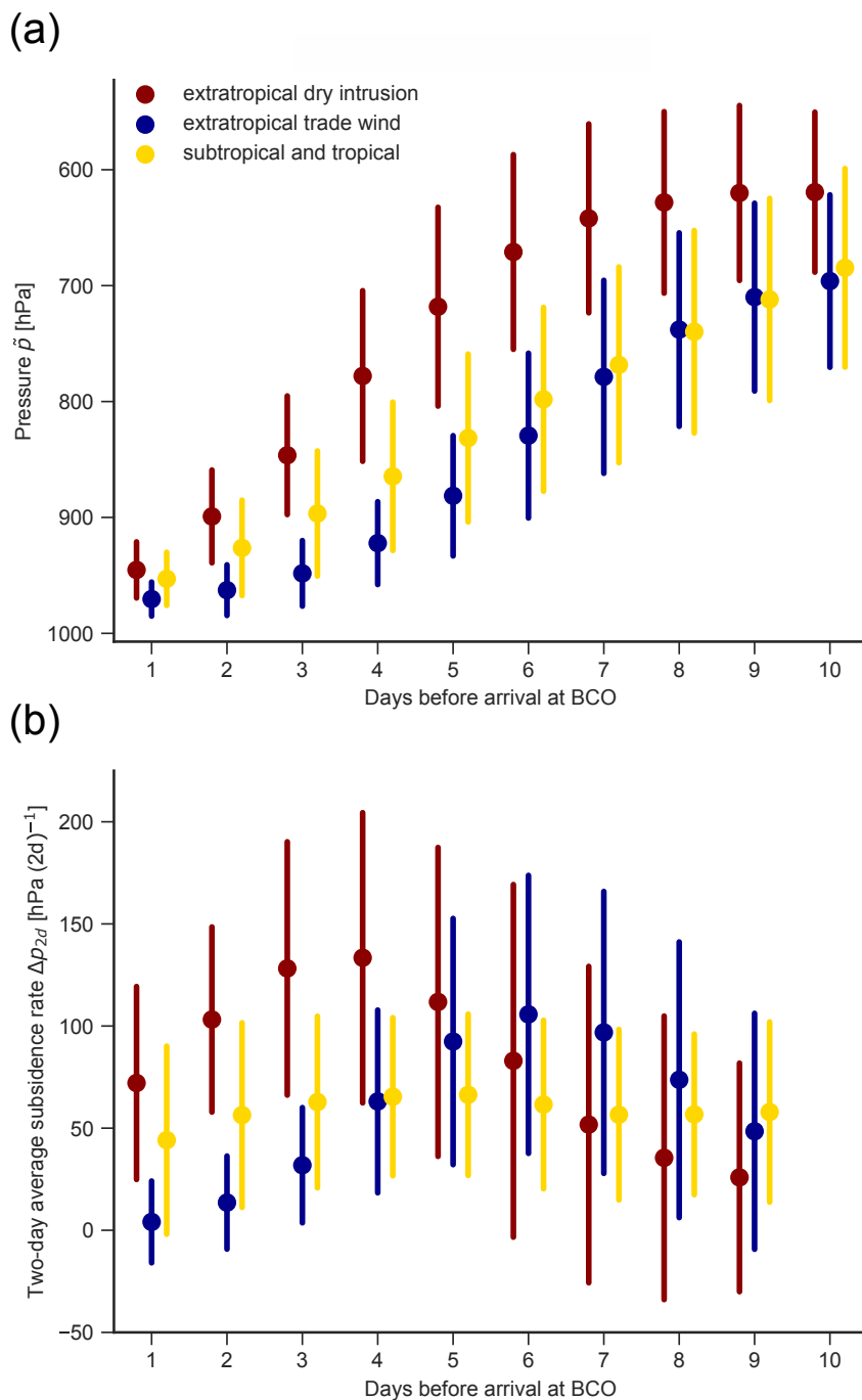
Figure 4: Climatological mean and standard deviation (bar) showing the pressure (a) and two-day subsidence rate (b) of the 40 sub-cloud layer air parcels within 1 to 10 days prior to their arrival above Barbados in January-February 2009-2018, classified into regimes with different transport pathways. The extratropical dry intrusion regime (27% occurrence frequency) is shown in dark red, the extratropical trade wind regime (28%) in blue, and the tropical regime (44%) in yellow.
