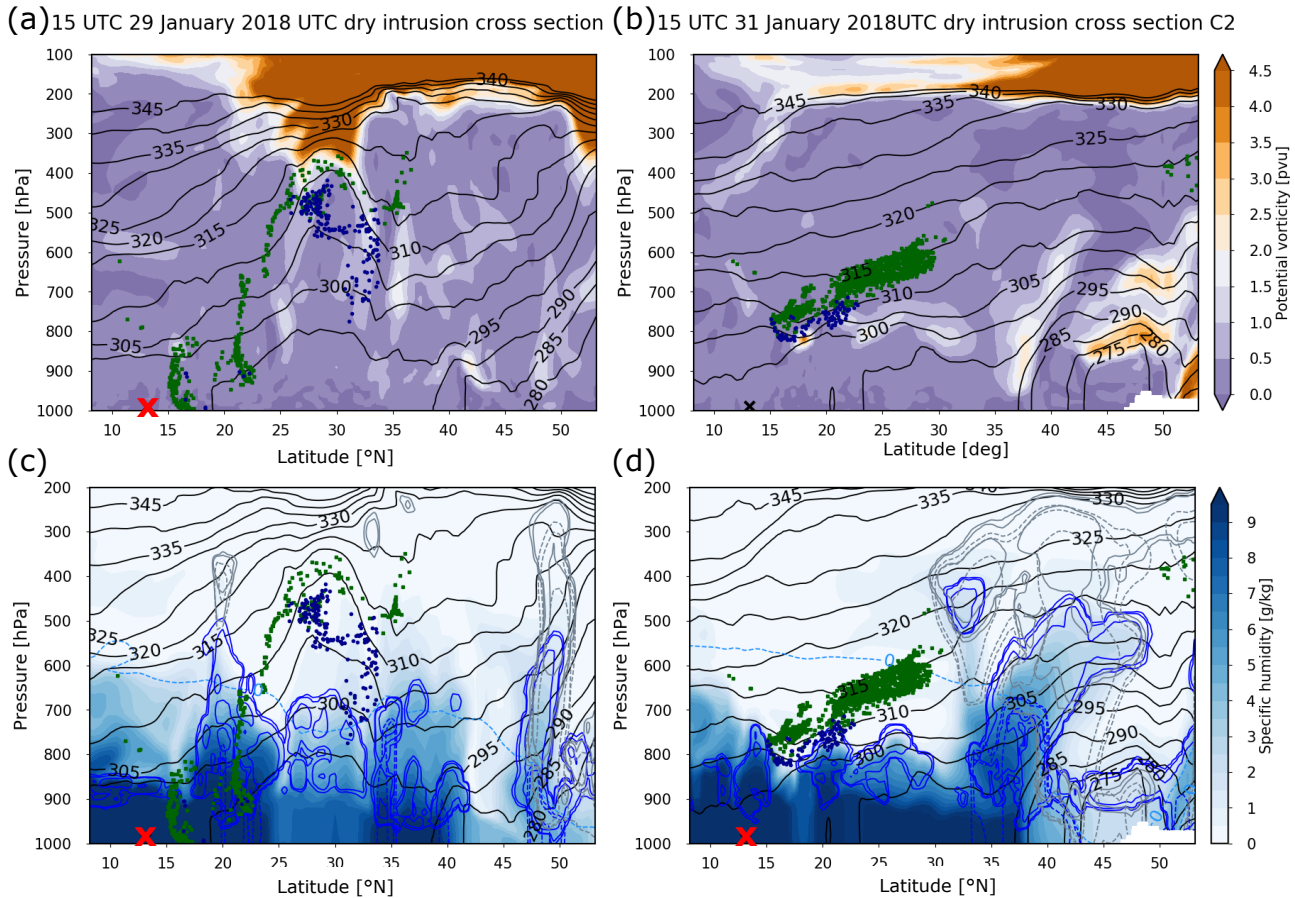
Figure 14: Meridional cross sections along the lines C1 and C2 in Fig. 11b at 15 UTC 29 January 2018 through the upper-level cutoff (C1, a,c) and at 15 UTC 31 January 2018 showing the strongly descending air parcels west of the cutoff (C2, b,d). Filled contours show (a,b) potential vorticity and (c,d) specific humidity. Isentropes are shown by black contours, every 5 K. In (c,d) cloud liquid water is shown by solid blue contours, rain water by dashed blue, ice water content by grey, and snow water content by dashed grey contours. All hydrometeor contour lines correspond to 5, 10 and 50 \text{mg kg}^{-1} . The green and blue points correspond to the positions of air parcels within \pm 1^\circ longitude of the cross section. The green air parcels form together the cloud layer (940-700 hPa) and the blue air parcels form the sub-cloud layer (surface to 940hPa) above Barbados during the period of the extratropical dry intrusion between 1-4 February 2018. The latitude of Barbados is highlighted by the red cross at the surface.
