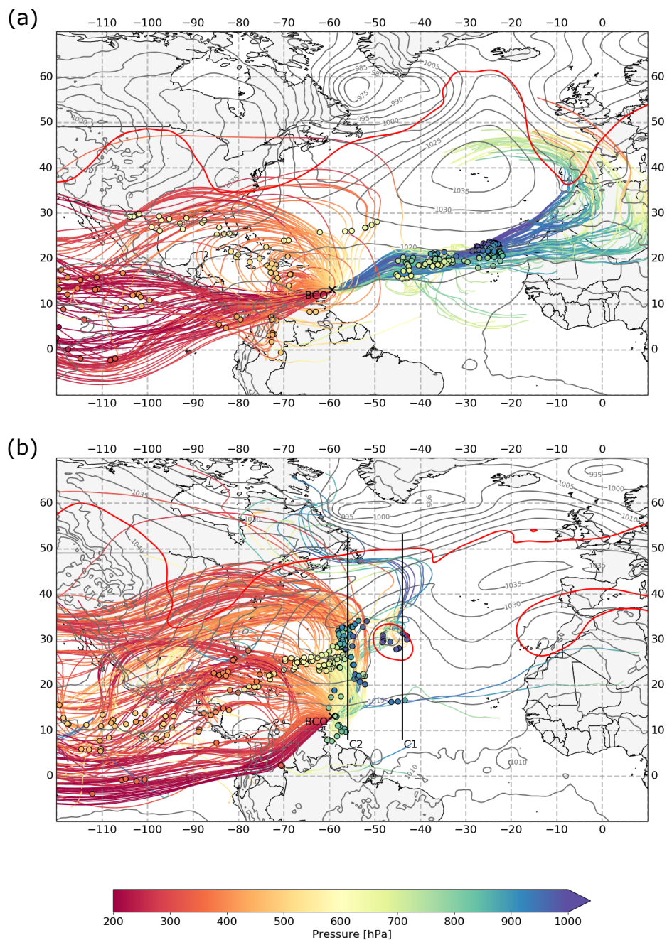
975 Figure 11: Back-trajectories from the BCO started at (a) 15 UTC 29 January 2018 (extratropical trade wind regime) and (b) 15 UTC 02 February 2018 (extratropical dry intrusion regime). The trajectories are coloured according to their pressure. The position 4 days before arrival above Barbados is indicated by a dot coloured with their arrival pressure at the BCO (blue in the sub-cloud layer, green in the cloud layer, orange in the free troposphere and red in the upper troposphere). The black cross indicates the location of Barbados (BCO). The grey contours show the sea level pressure and the red contour denotes 2 pvu on 320 K, 4 days before arrival.
