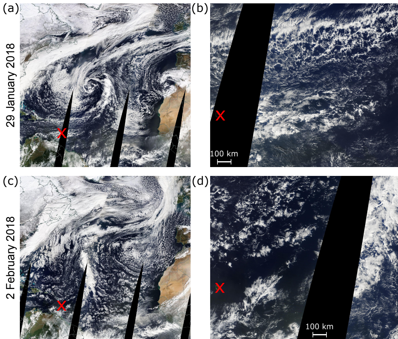
970 Figure 10: Cloud patterns (a,c) over the North Atlantic and (b,d, 48–60°W, 10–20°N) around Barbados at 1430 UTC 29 January 2018 (a,b) and 1430 UTC 02 February 2018 (c,d) as seen from the MODIS instrument on TERRA. Images from NASA Worldview Snapshots ( https://wvs.earthdata.nasa.gov ). In (a) the cyclone is visible that is associated with the extratropical dry intrusion reaching Barbados a few days later on 1–4 February 2018.
