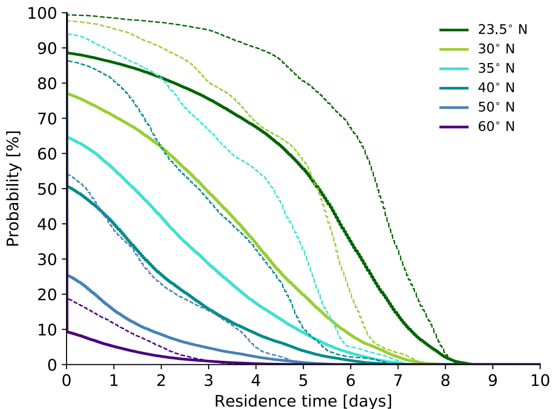
905 Figure 3: Exceedance probabilities of the residence time in different spherical caps (north of 23.5°N, 30°N, 35°N, 40°N, 50°N, and 60°N) of air parcels arriving in the sub-cloud layer ( p \geq 940 hPa) in Barbados, based on a climatology of 10-day backward trajectories from Barbados calculated with ERA5 in January and February 2009 to 2018 (568'320 trajectories, solid lines) and for January and February 2018 (isoTrades campaign; 23'040 trajectories, dashed lines).
