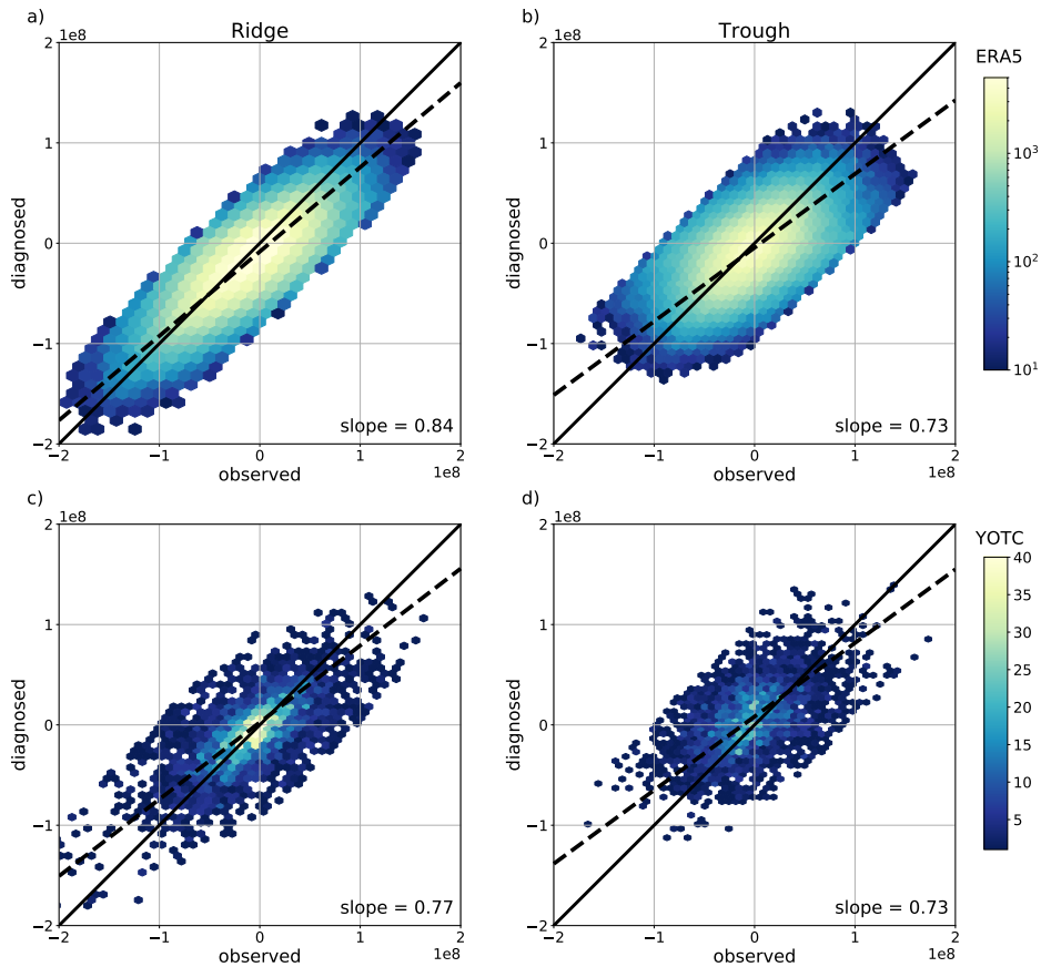
Figure 2. Relation between observed and diagnosed amplitude evolution tendencies (in PVU m^2/s ) for both datasets, ERA5 (a,b) and YOTC (c,d), and for ridges (a,c) and troughs (b,d) separately. For a perfect correspondence all scatters should be aligned along the black solid line of slope 1 and cross the origin. The 2d-fit ( total least squares ) is indicated by the black dashed line with slope + (slope lower right corner) . Color shading describes number of values within a certain hexbin (for ERA5 on logarithmic scale). For ERA5 620316 datapoints are included, for YOTC 7692.
