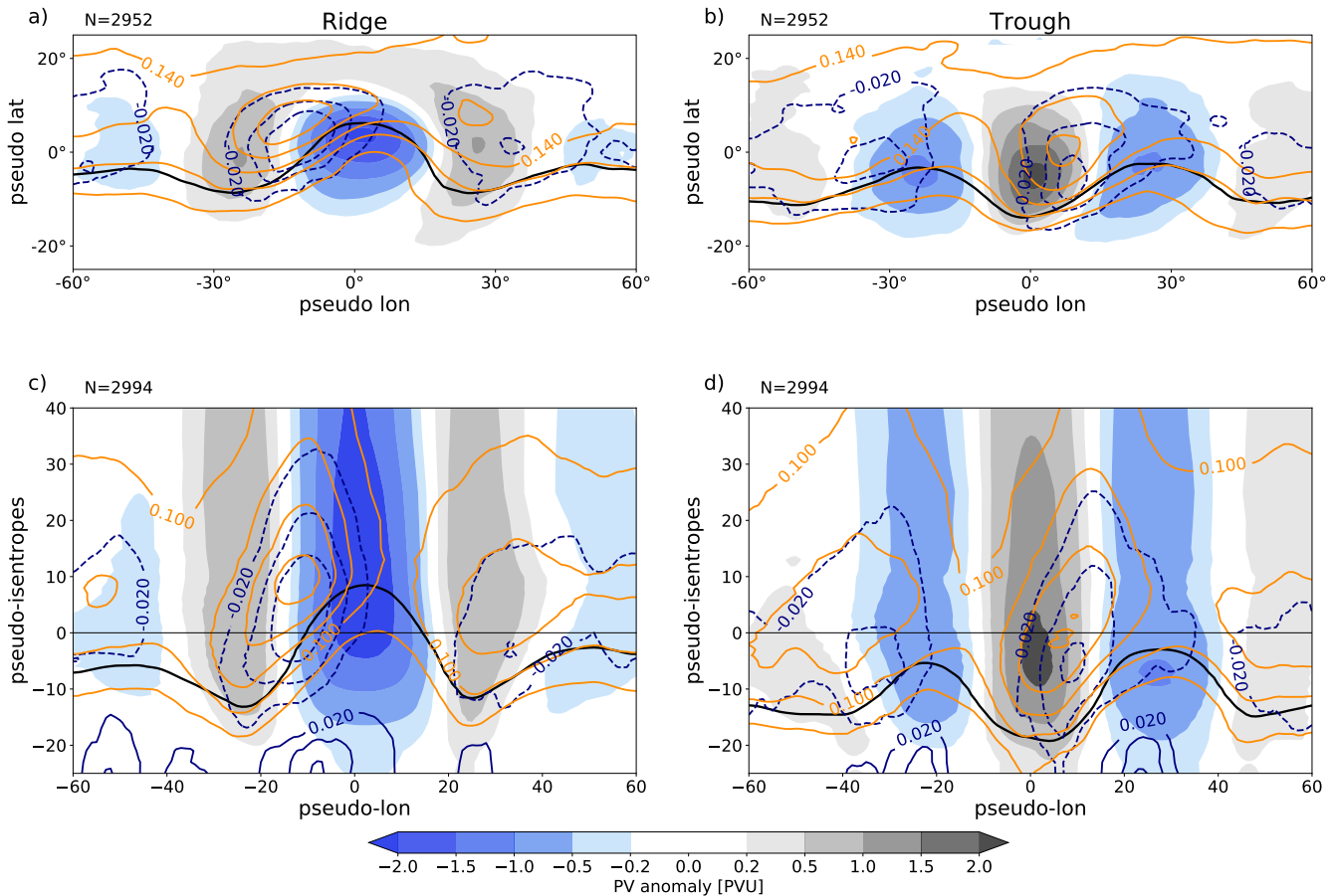
Figure 10. Spatial composites of PV anomalies (shading) and PV tendencies for (a,c) ridges and (b,d) troughs during YOTC-period averaged from 72 h before to 72 h after the maximum of baroclinic growth. The different contours show in blue PV tendencies due to the cloud scheme ( \pm(0.02,0.04,0.06) PVU/day, negative dashed), in orange PV tendencies due to longwave radiation ( \pm(0.06,0.1,0.14,0.18,0.22) PVU/day) and in black the 2-PVU contour depicting the tropopause. The isentropic level in (a,b) follows the seasonal cycle defined in subsection 2.2 and relates to the pseudo-isentropic level 0 in (c,d). Note, only YOTC-data is shown. A box-smoothing of 3 points is applied for visual clarity.
