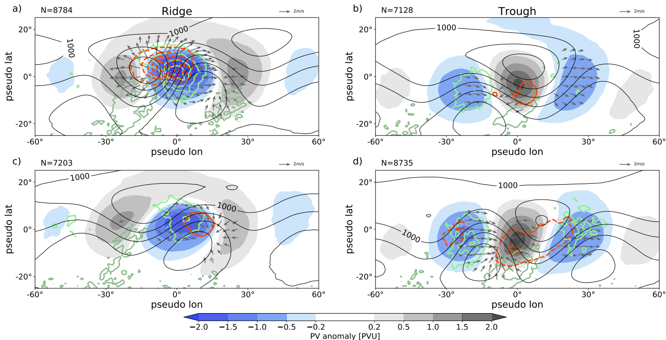
Figure 6. Spatial composites of PV anomalies (shading) and PV' tendencies for the strongest (a,bc) ridges and weakest (cb,d) contribution of troughs at times when the divergent PV tendencies for ridges yield maximum amplification (a,eb) and troughs maximum weakening (bc,d) ; respectively of the respective amplitude. The different contours show in red PV tendencies due to divergent flow ( \pm(0.5, 1, 1.5, 2, 2.5, 3) PVU/day, negative dashed), in light green convergence of IVT as proxy for latent heat release ( \pm(0.02,0.04,0.06,0.08,0.1) kg m -2 day -1 , negative darker divergence of IVT in dark green) and in thin black solid geopotential at 1000 hPa (every 200 m 2 /s 2 , 1000 m 2 /s 2 labeled). The arrows refer to the divergent wind, only shown at grip points with values greater than 1 m/s (reference vector in upper-right corner). The isentropic level for PV anomalies and PV tendencies follows the seasonal cycle.
