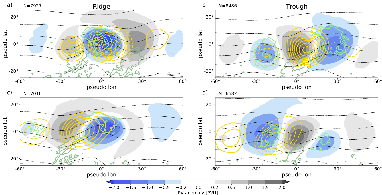
Figure 5. Spatial composites of PV anomalies (shading) and PV' tendencies for the strongest (a,bc) ridges and weakest (c,d) contribution of troughs at times the baroclinic PV tendencies for ridges yield maximum amplification (a,eb) and troughs maximum weakening (bc,d) respectively of the respective amplitude . The different contours show in yellow PV tendencies due to baroclinic interaction ( \pm(0.1, 0.15, 0.2, 0.25, 0.3, 0.35, 0.4, 0.45, 0.5) PVU/day, negative dashed), in light green convergence of IVT as proxy for latent heat release ( \pm(0.02, 0.04, 0.06, 0.08, 0.1) \text{kg m}^{-2} \text{day}^{-1} , negative darker divergence of IVT in dark green ) and in thin black mean temperature between 850 and 800 hPa (every 5 K). Note, the mean temperature indicates the location of warm (northward extension of contour) and cold (southward extension of contour) anomalies at lower levels. The isentropic level for PV anomalies and PV tendencies follows the seasonal cycle.
