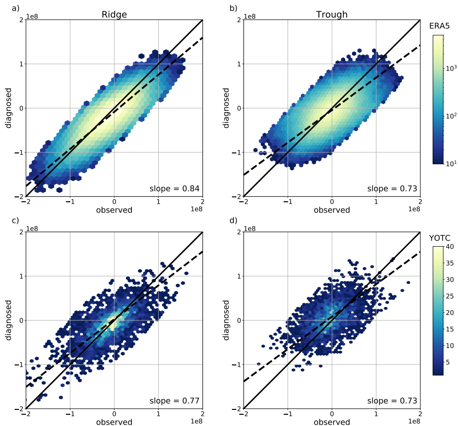
Figure 2. Relation between observed and diagnosed amplitude tendencies (in \text{PVU m}^2/\text{s} ) for both datasets, ERA5 (a,b) and YOTC (c,d), and for ridges (a,c) and troughs (b,d) separately. For a perfect correspondence all scatters should be aligned along the black solid line of slope 1 and cross the origin. The 2d-fit (total least squares) is indicated by the black dashed line (slope lower right corner). Color shading describes number of values within a certain hexbin (for ERA5 on logarithmic scale). For ERA5 620316 datapoints are included, for YOTC 7692.
