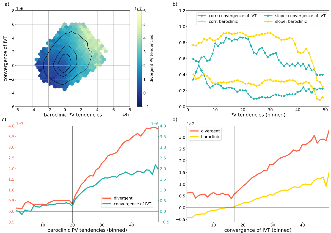
Figure 11. Relation between divergent (DIV) and baroclinic (BC) PV tendencies (in PVU m 2 /s), and convergence of IVT (LHRproxy, in kg day -1 ) within ridges. a) Binned scatter plot of BC (x-axis) and LHRproxy (y-axis) with average DIV shaded. Occurrence distribution shown by black contours (100,500,1000). b) Correlation (dots) and slope (stars) between (green) LHRproxy and DIV in each bin of BC and between (yellow) BC and DIV in each bin of LHRproxy. Values have been normalized by their respective standard deviation before regression. c) DIV (left y-axis) and LHRproxy (right y-axis) as function of BC. The vertical line depicts the bin for that BC turns positive. d) DIV and BC as function of LHRproxy. The vertical line depicts the bin for that LHRproxy turns positive. In b), c) and d) data divided into equally spaced bins from the 0.1% percentile to the 99% percentile, respectively.
