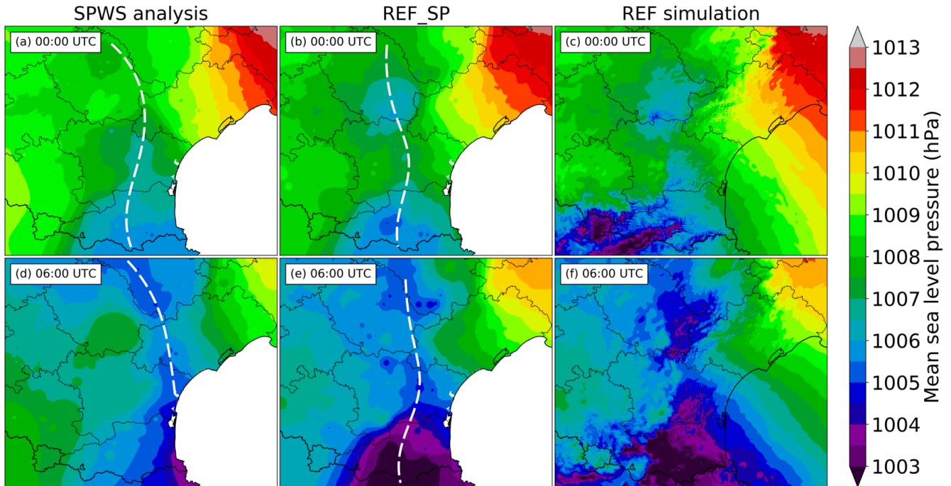
Figure 7. Mean sea level pressure on 15 October at (a,b,c) 00:00 UTC and (d,e,f) 06:00 UTC from (a,d) the SPWS analysis, (b,e) REF_SP and (c,f) the REF simulation. Solid black lines indicate French departments and country borders. Dashed white lines indicate the approximate location of the MSLP trough. Analyses are not computed over the Mediterranean Sea, in white, because of the lack of surface observations over sea.
