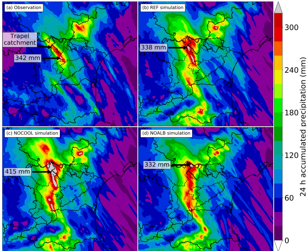
Figure 6. 24 h accumulated precipitation between 12:00 UTC 14 October and 12:00 UTC 15 October from the (a) ANTILOPE analyses, (b) REF, (c) NOCOOL and (d) NOALB simulations. Solid black lines indicate French departments and country borders. Dotted black lines indicate catchment limits of the Aude basin and its tributaries.
