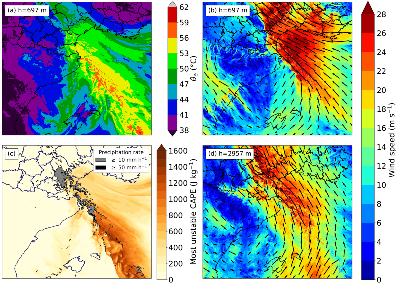
Figure 15. As Fig. 12 at 07:00 UTC 15 October.
