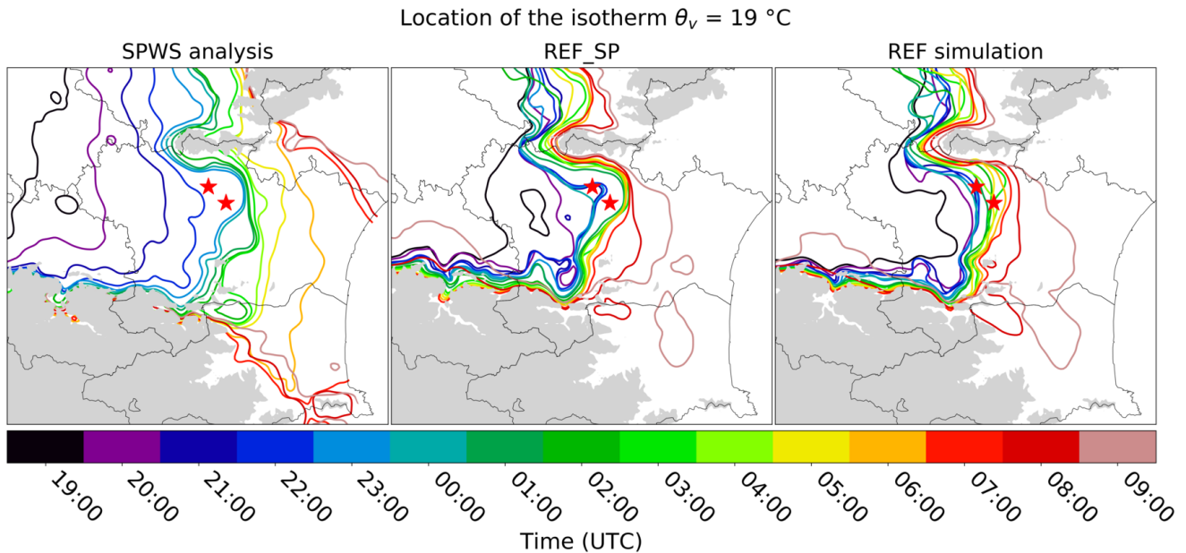
Figure 9. Location of the 19^\circ\text{C} virtual potential temperature ( \theta_v ) isotherm at 2 m height between 19:00 UTC 14 October and 09:00 UTC 15 October from (a) the SPWS analysis, (b) REF_SP and (c) the REF simulation. Terrain elevation over 750 m above sea level (a.s.l.) is shaded in grey. Red stars show the location of Villegailhenc (northern star) and Trèbes (southern star), towns strongly damaged by the HPE.
