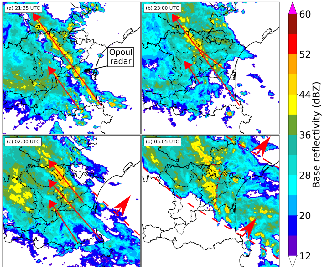
Figure 5. Radar base reflectivity from the French operational mosaic on 14 October at (a) 21:35 UTC, (b) 23:00 UTC and on 15 October at (c) 02:00 UTC and (d) 05:05 UTC. Red arrows with triangle arrowheads show the axes of continuous convective cell renewal and the movement of individual cells shown by radar. Dashed lines and large red arrowheads indicate the northeastwards movement of the convective system ahead of CF2.
