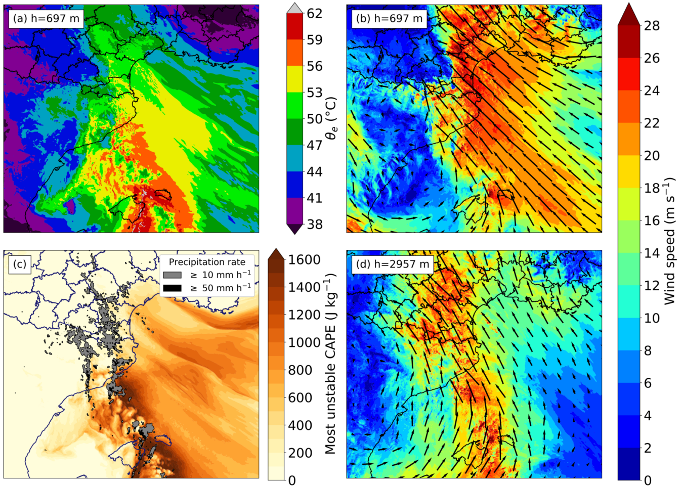
Figure 12. REF simulation at 00:00 UTC 15 October of (a) equivalent potential temperature ( \theta_e ) at 697 m height, (b) wind at 697 m height, (c) most unstable CAPE with instantaneous precipitation rate and (d) wind at 2957 m height.
