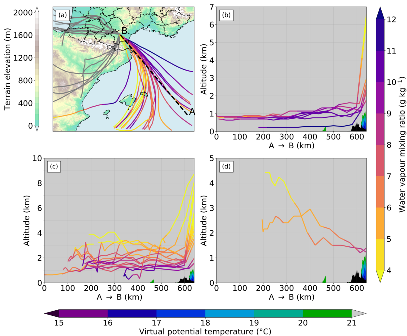
Figure 14. As Fig. 11 for trajectories ending at 07:00 UTC 15 October at 43.26° N, 2.34° E. Air parcels are projected along the same axis A–B but separated depending on their origin and behaviour: (b) ascending parcels from east, (c) ascending parcels from south or west and (d) descending parcels from south.
