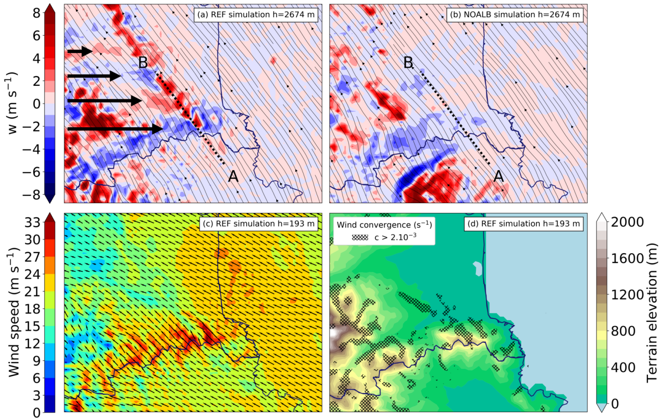
Figure 17. Vertical velocity ( w ) and horizontal wind streamlines at 2674 m height in the (a) REF and (b) NOALB simulations. Horizontal wind (c) speed and direction and (d) convergence > 2 \times 10^{-3} \text{ s}^{-1} at 193 m height in the REF simulation at 05:00 UTC 15 October.
