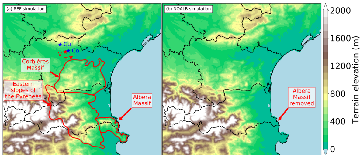
Figure 2. Orography of the south Languedoc-Roussillon including the Aude department in simulations (a) REF and (b) NOALB in which the Albera Massif is removed. Stars indicate towns affected by the HPE and mentioned in the article: "V" is Villegailhenc, "T" is Trèbes, "Cu" is Cuxac-Cabardès and "Co" is Conques-sur-Orbiel. The two red stars are landmarks displayed in other figures of the article. Red contours indicate mountain massifs.
