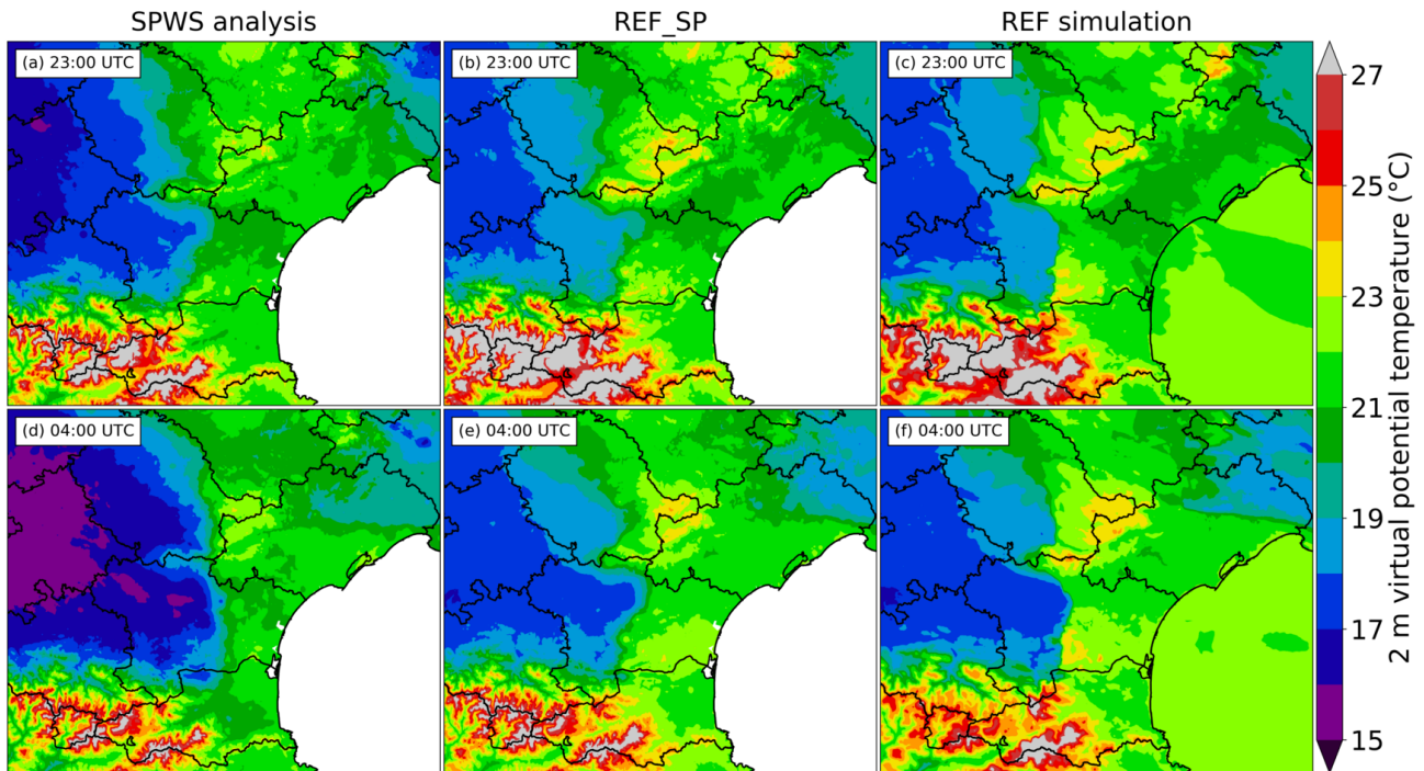
Figure 8. 2 m height virtual potential temperature at (a,b,c) 23:00 UTC 14 October and at (d,e,f) 04:00 UTC 15 October from (a,d) the SPWS analysis, (b,e) REF_SP and (c,f) the REF simulation.
