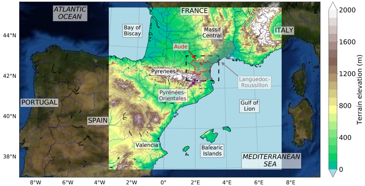
Figure 1. Map of southwestern Europe where locations mentioned in the article are indicated. The bright square and the dashed black line correspond to the two grid-nested domains (parent and child) of the simulation. Inside the bright square, terrain elevation from the parent model is shown; outside, it is the NASA visible blue marble image (from https://visibleearth.nasa.gov ). Solid black lines indicate French departments and country borders. Languedoc-Roussillon, a region including Aude and Pyrénées-Orientales departments is shaded. The two little red stars indicate from north to south the location of Villegailhenc and Trèbes, two towns strongly affected by the HPE.
