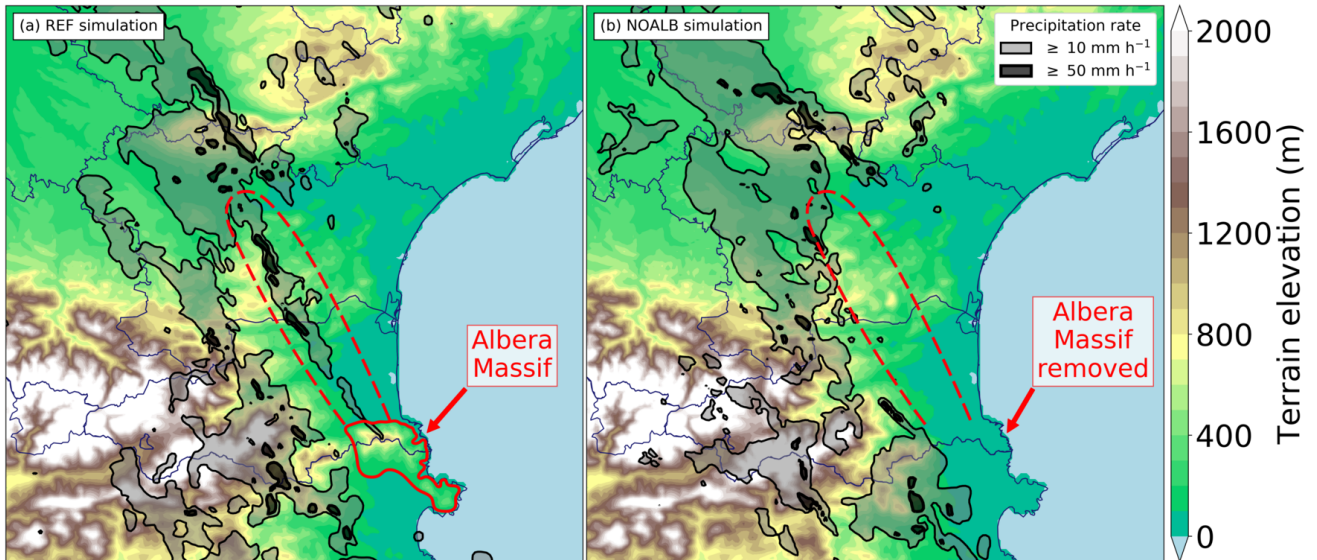
Figure 16. Instantaneous precipitation rate at 05:00 UTC 15 October superimposed on the terrain elevation of (a) REF and (b) NOALB simulations.
