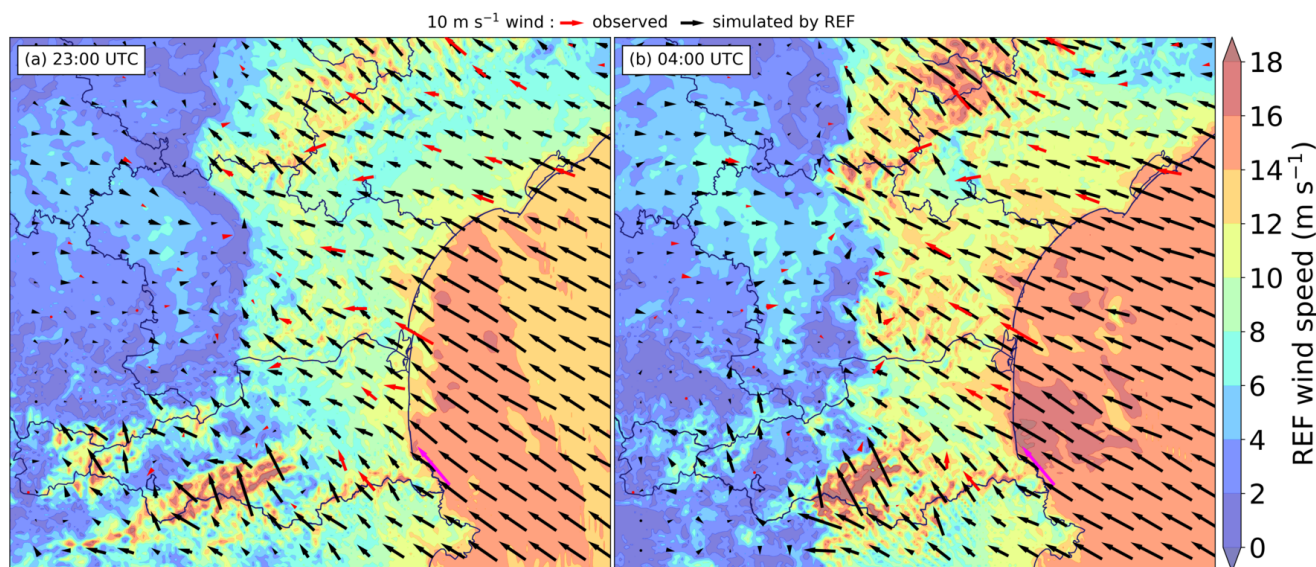
Figure 10. 10 m height instantaneous horizontal wind speed and direction simulated by REF (black arrows, speed also displayed with filled contours) and 10 m height 10 min averaged horizontal wind speed and direction observed (red arrows) at (a) 23:00 UTC 14 October and at (b) 04:00 UTC 15 October. The arrow length is proportional to the wind speed. Purple arrow is the Cap Béar observation measured at an unconventional height of 36 m.
