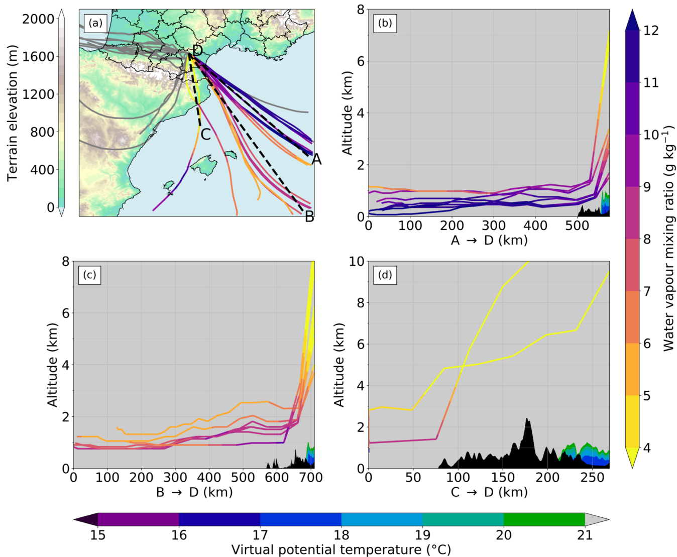
Figure 13. As Fig. 11 for trajectories ending at 04:00 UTC 15 October at 43.31° N, 2.28° E.
