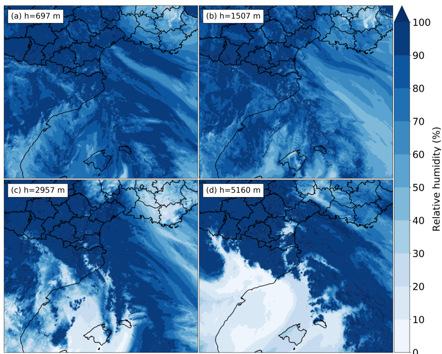
Figure 20. Relative humidity in the REF simulation at 04:00 UTC 15 October at (a) 697 m height (b) 1507 m height (c) 2957 m height (d) 5160 m height.
