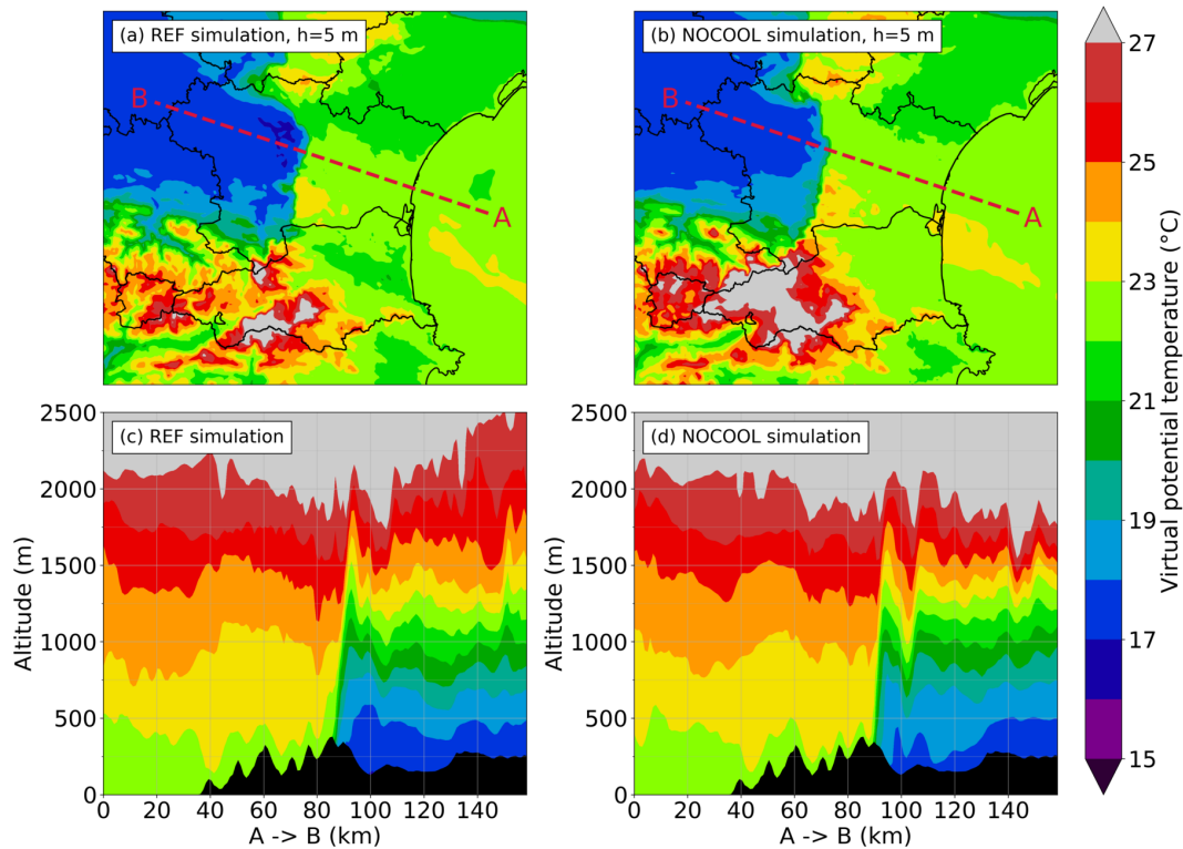
Figure 19. Virtual potential temperature at 5 m height for the (a) REF and (b) NOCOOL simulations at 04:00 UTC 15 October. Vertical cross sections of virtual potential temperature along the A–B axis are drawn for the (c) REF and (d) NOCOOL simulations.
