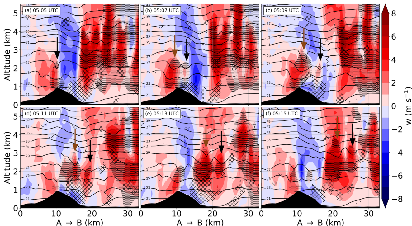
Figure 18. Vertical velocity ( w , \text{m s}^{-1} ), potential temperature (black contours, ^{\circ}\text{C} ), horizontal convergence > 2 \times 10^{-3} \text{ s}^{-1} (black diagonal hatches) and hydrometeor mixing ratio > 1 \text{ g kg}^{-1} (little black dots) between 05:05 and 05:15 UTC 15 October. Terrain is in black.
