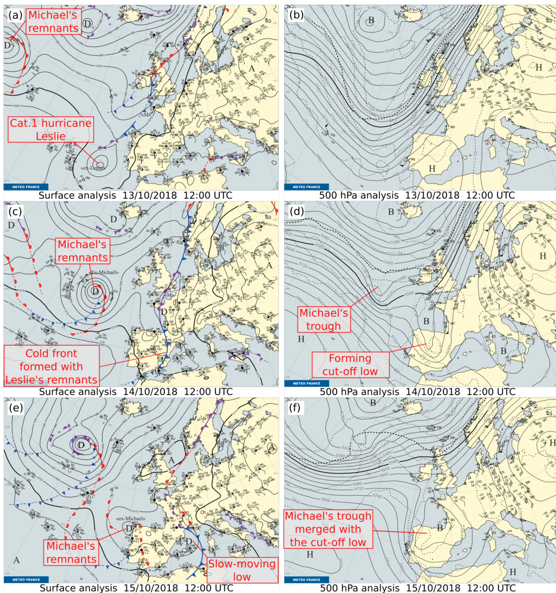
Figure 3. (a,c,e) Surface and (b,d,f) 500 hPa analyses of Météo-France national forecast department (Santurette and Joly, 2002) at (a,b) 12:00 UTC 13 October 2018, (c,d) 12:00 UTC 14 October 2018 and (e,f) 12:00 UTC 15 October 2018. Surface fronts are manually drawn using conventional observations, satellite, radar images and short-term forecasts (instead of analyses due to availability time constraints). Mean sea level pressure (in hPa), 500 hPa geopotential height (in gpm) and temperature (in °C) are from Météo-France operational global model ARPEGE (Courtier et al., 1991) 6 h forecast of the T–6 h run (T: time of the chart). Surface (respectively altitude) low-pressure centres are indicated by "D" (resp. "B") and high-pressure centres by "A" (resp. "H").
