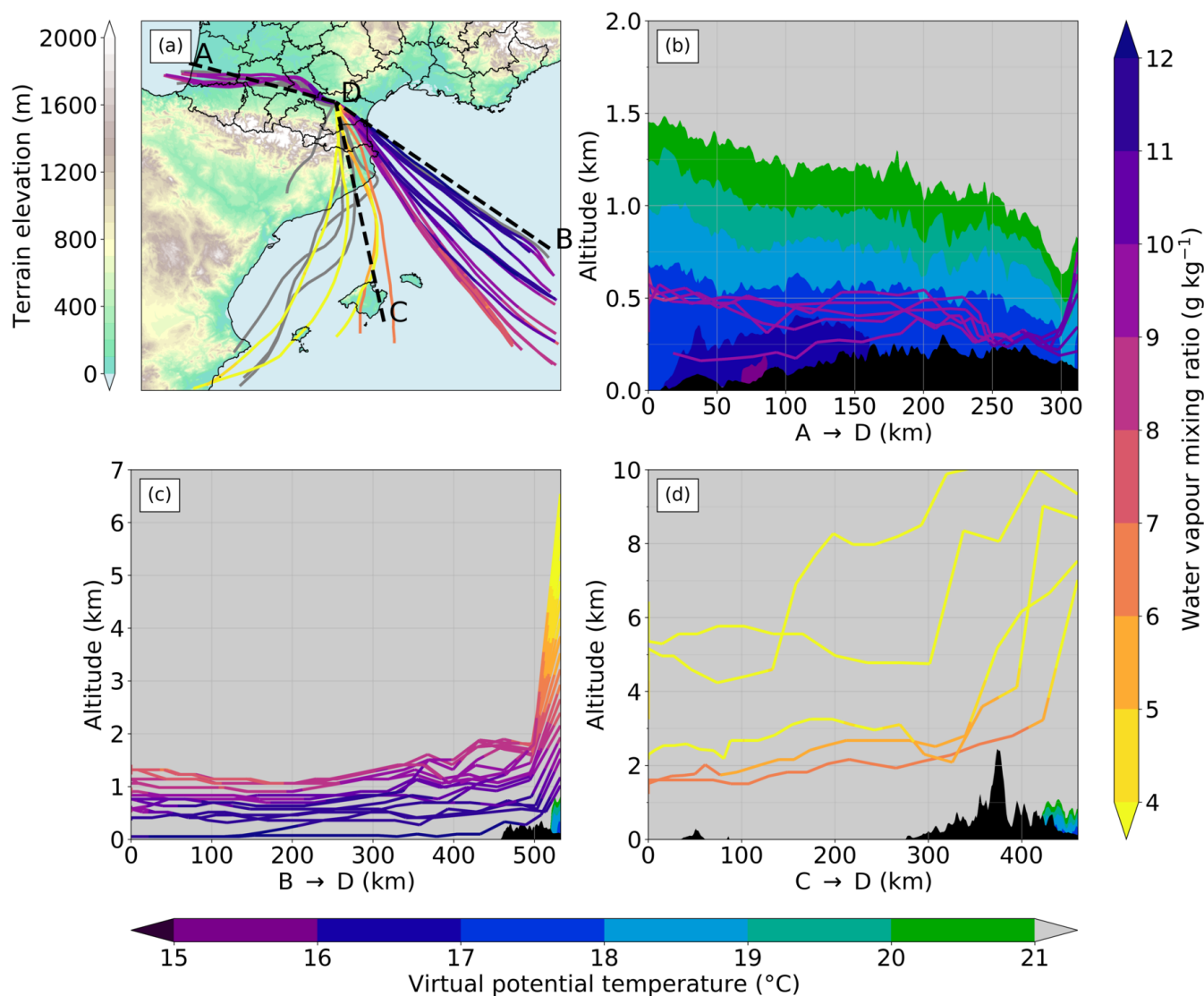
Figure 11. (a) Horizontal projection of the 40 backward trajectories from air parcels taken inside the atmospheric column located in "D" ( 43.25^{\circ} N, 2.25^{\circ} E) at 00:00 UTC 15 October in the REF simulation. Trajectories in colour are the ones projected in (b-d): their colour varies according to the water vapour mixing ratio of the parcels. Other trajectories are in grey. Trajectories are computed until 12:00 UTC 14 October, except for parcels that reach domain boundaries before that time. (b-d) Vertical projections of backward trajectories along the dashed black lines shown in (a) and corresponding cross sections of virtual potential temperature at 00:00 UTC 15 October. Each parcel is projected on the section closest to its trajectory inland. Terrain is in black.
