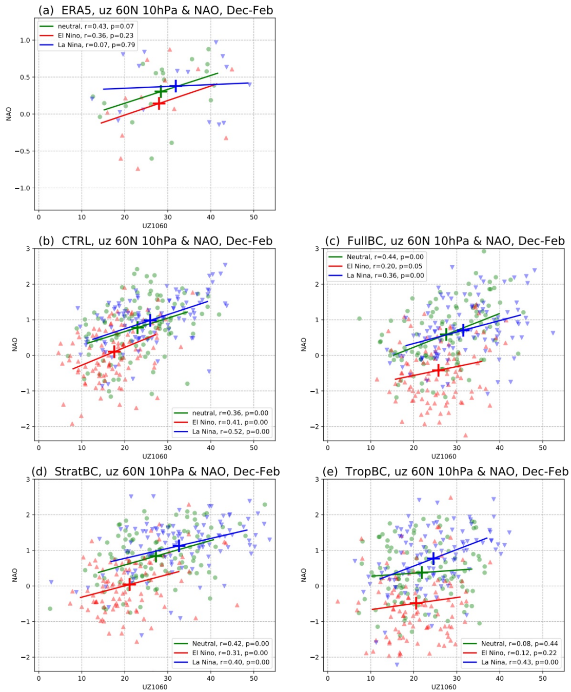
485 Figure 3. Scatterplot with regression line of mean DJF values of uz at 60N 10hPa and the NAO index, for (a) ERA5 (1950-2021), (b) CTRL, (c) FullBC, (d) StratBC and (e) TropBC. Neutral years are green, El Niño years are red, and La Niña years are blue. The large crosses indicate the mean value for each El Niño/La Niña/neutral experiment. Correlation and p-values shown in the legend.
