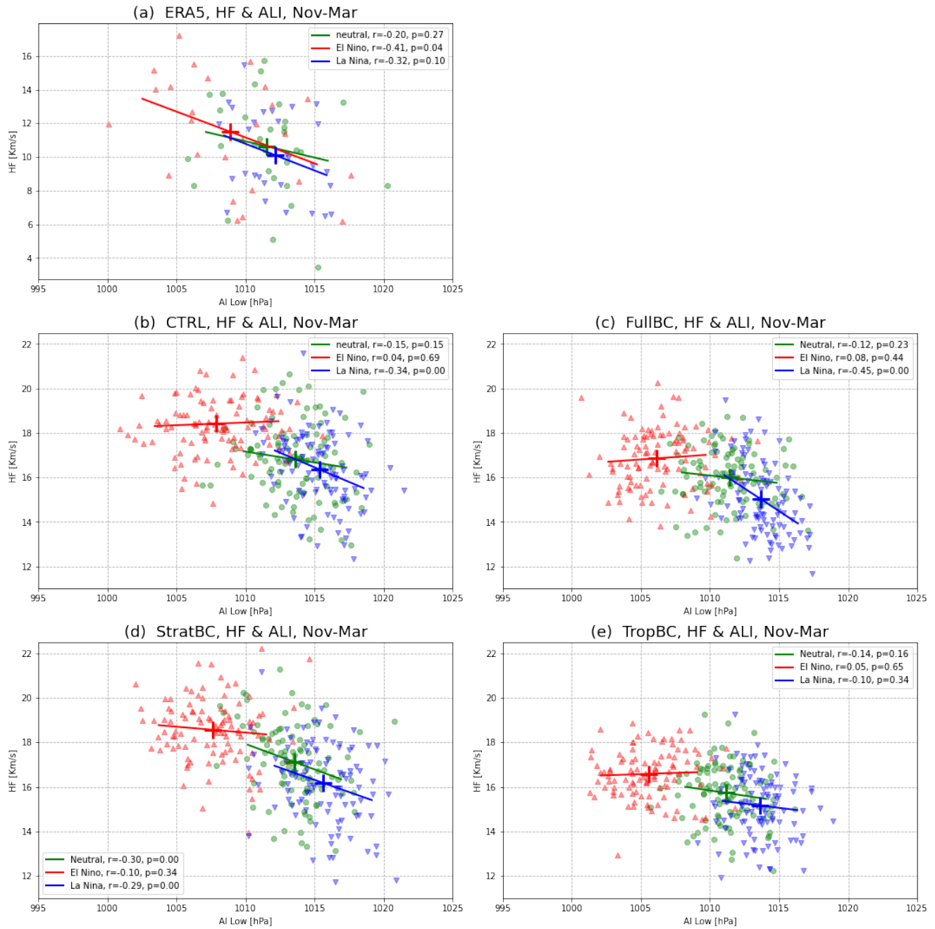
500 Figure 6. Scatterplot with regression line of mean NDJFM values of the Aleutian Low Index and the heat flux between 45N–75N at 100 hPa, for (a) ERA5 (1950–2020), (b) CTRL, (c) FullIBC, (d) StratBC and (e) TropBC. Neutral years are green, El Niño years are red, and La Niña years are blue. Correlation and p-values shown in the legend.
