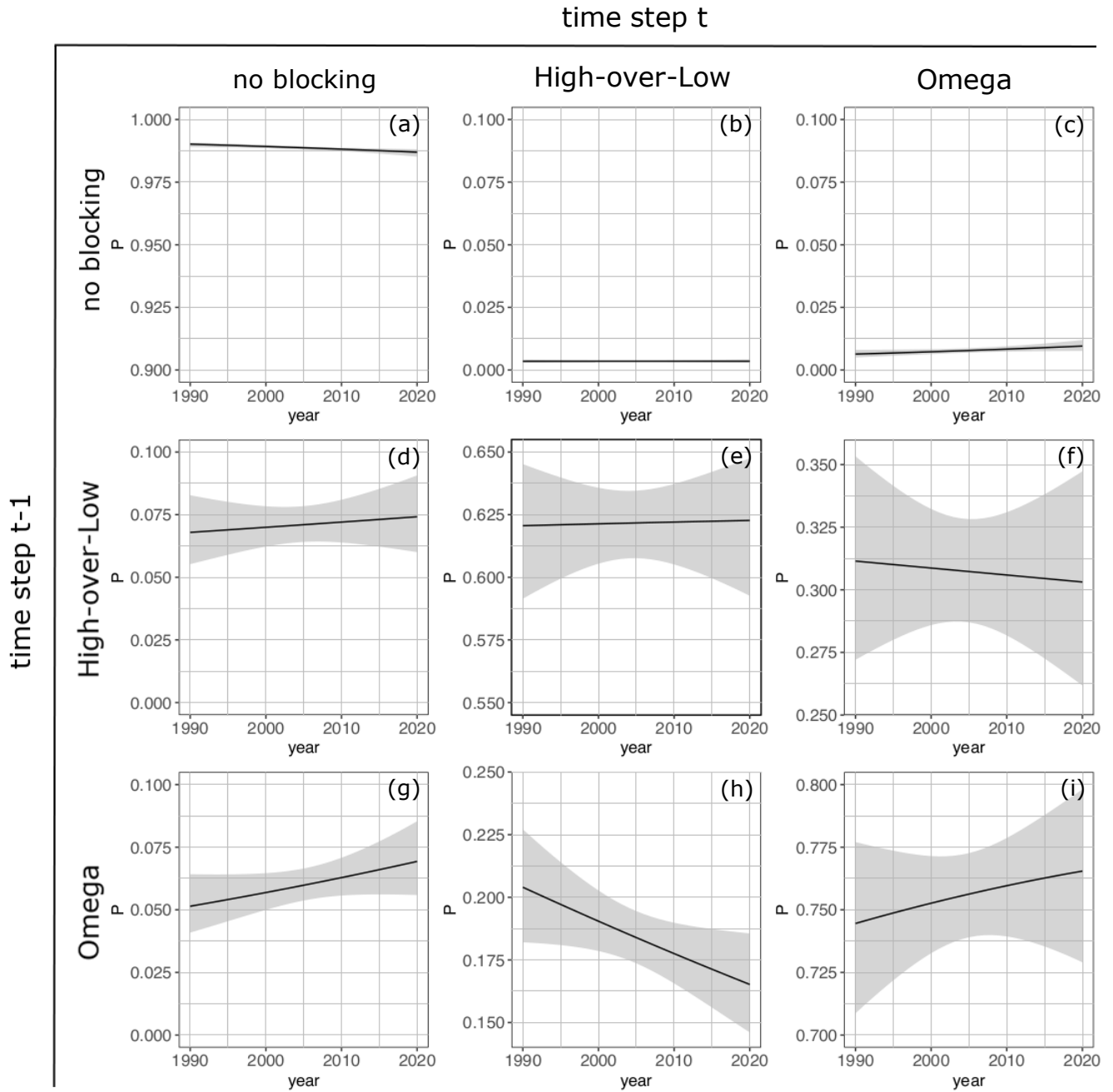
Figure 13. Transition probabilities analogous to the matrix of a three-state Markov process (Eq. 15) as a function of years (Eq. 26) in the Euro-Atlantic region ( 40^\circ W - 30^\circ E ). (a) p_{nB|nB} , (b) p_{HoL|nB} , (c) p_{\Omega|nB} , (d) p_{nB|HoL} , (e) p_{HoL|HoL} , (f) p_{\Omega|HoL} , (g) p_{nB|\Omega} , (h) p_{HoL|\Omega} and (i) p_{\Omega|\Omega} . Shadings show 95 % confidence intervals.
