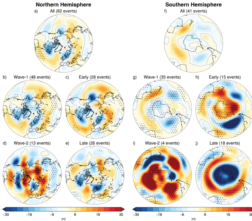
Figure A2. Composite of the linearly detrended 500 hPa geopotential height anomalies [m] from JRA-55 data for (a,f) all FSW events based on the 10 hPa dates, and classified as (b,g) wave-1, (d,i) wave-2, (c,h) early, or (e,j) late averaged over the 7-30 days after the central FSW date (i.e., lags of 7-30 days) for (a-e) the NH and (f-j) the SH extratropics. Stippling in (a,f) indicates regions where the anomaly composites are significantly different from zero at the 95% confidence level, while stippling in other panels shows where composites are significantly different from each other (e.g., wave-1 vs wave-2, early vs late), both according to a 1000-sample bootstrap analysis (with replacement).
