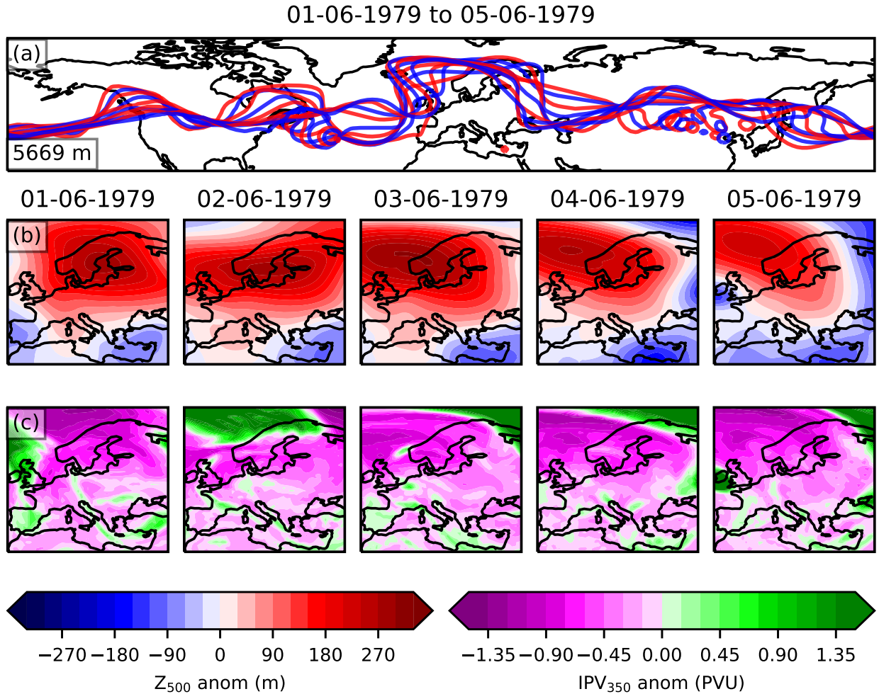
Figure 1. The information used to classify blocks in the ERA5 ground truth dataset (GTD). (a) shows the Z_{500} contour for the averaged value across 30-70^{\circ}\text{N} , indicated in the bottom left of the panel. The red and blue colours highlight the contours at midnight and midday respectively. (b) and (c) show the Z_{500} time detrended anomaly and \text{IPV}_{350} anomaly for each day.
