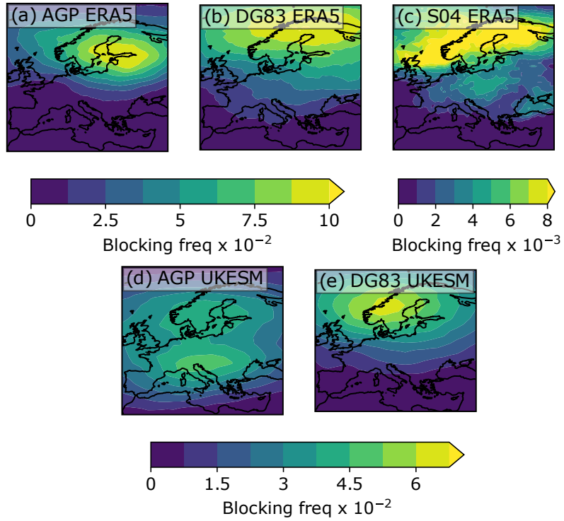
Figure A4. Occurrence of blocking events per grid cell across JJA Europe for three BIs in ERA5 1979-2019 and two BIs in UKESM JJA 1960-2060.
