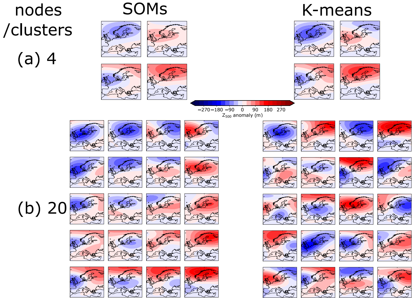
Figure A5. Comparison of the SOM analysis and K-means clustering for (a) 4 and (b) 20 nodes/clusters. Whilst the K-means and SOM analysis produce a similar set of patterns for smaller node numbers, their behaviour diverges for larger node numbers. Since the neighbourhood function ensures that several nodes are updated at once, the SOM produces a continuum of weather patterns. However, since the K-means clustering updates each centroid independently, it will seek to maximise the differences between each cluster. This causes some centroids for high cluster numbers to represent mixed weather regimes that are less realistic than the SOM continuum of weather regimes. The data used for above is ERA5 Z 500 across JJA 1979-2019.
