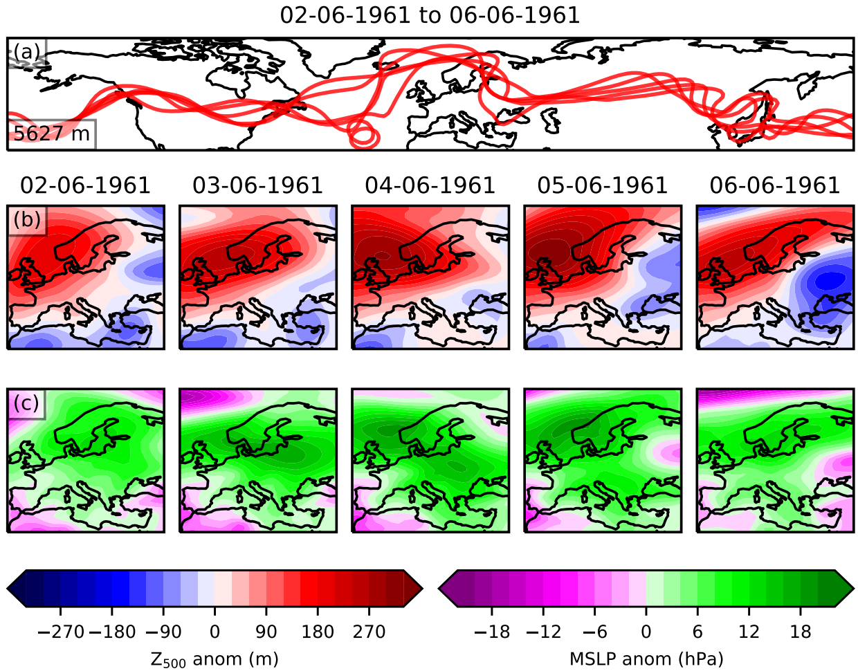
Figure A1. The information used to classify blocks in the UKESM GTD. (a) shows the daily Z_{500} contour for the averaged value across 30-70 °N, indicated in the bottom left of the panel. (b) and (c) show the Z_{500} time detrended anomaly and MSLP anomaly for each day.
