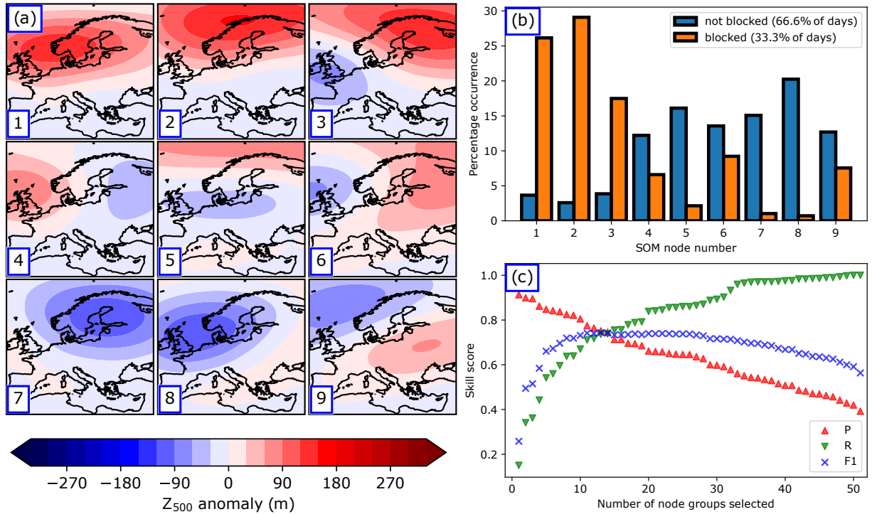
Figure 3. The SOM blocking index (SOM-BI). (a) The trained 3x3 SOM for Z_{500} time-detrended anomaly. (b) Normalised histograms showing the distributions of occurrence of BMUs for the days identified as blocked or non-blocked within the GTD. (c) The SOM-BI optimisation of the set of node groups against three different skill scores (precision (P), recall (R) and F1 score) that are associated with the GTD blocking events.
