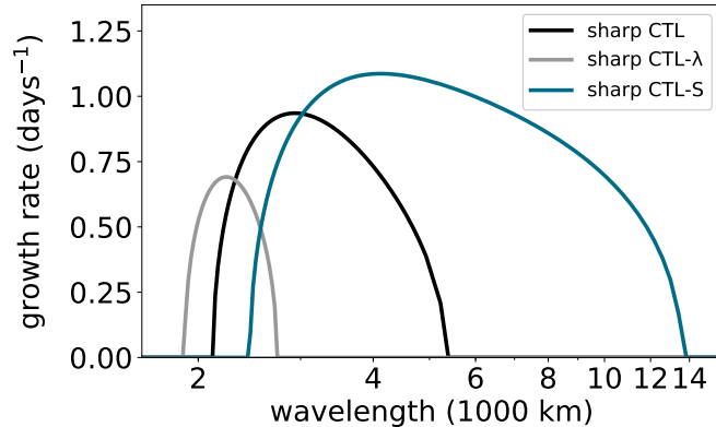
Figure 2. Growth rate vs. wavelength for the sharp CTL (black), CTL- \lambda (grey), and CTL-S (blue) experiments. See text for further details, where either \lambda and S , only \lambda , or only S are discontinuous, respectively.
