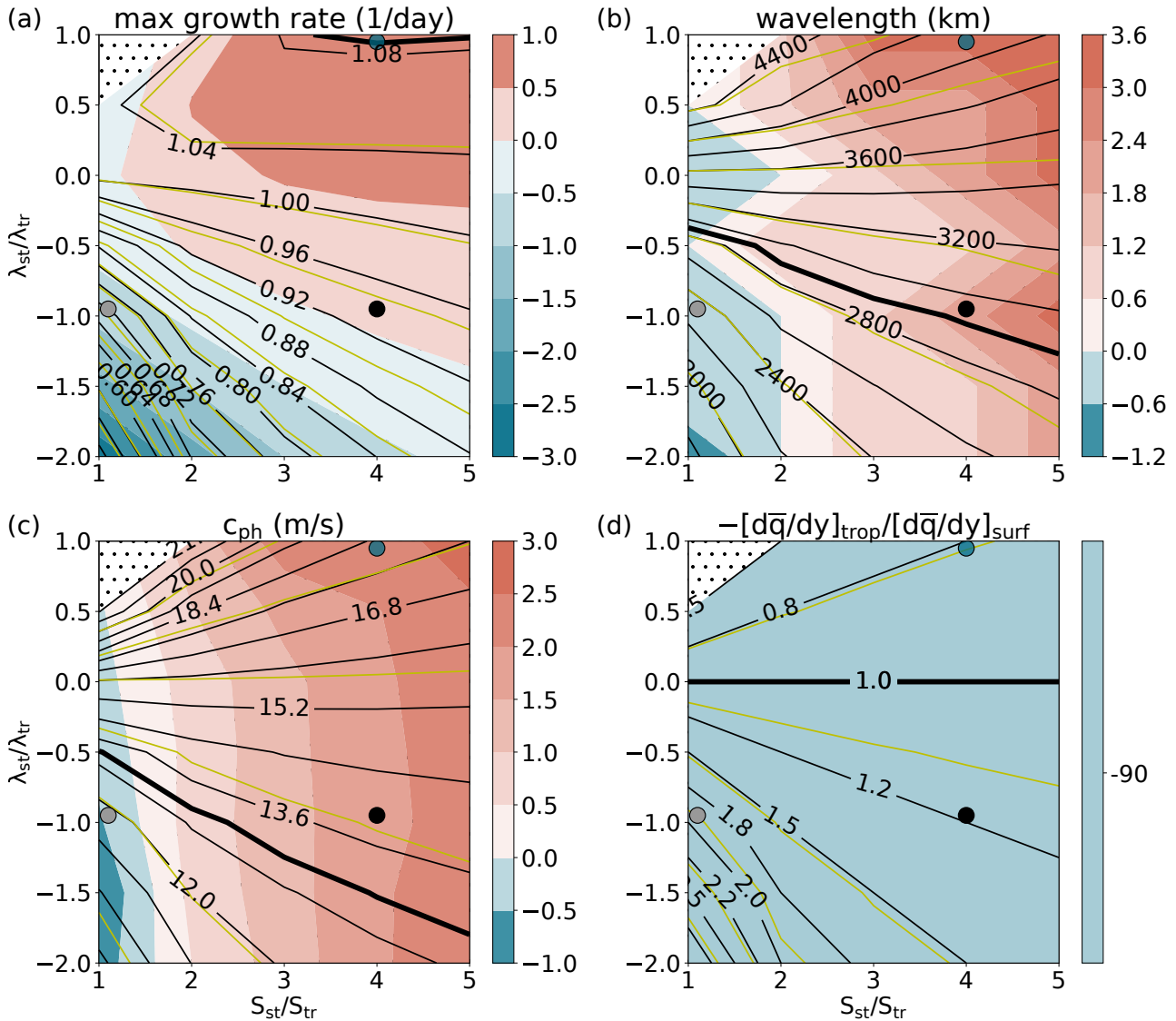
Figure 4. Growth rate, wavelength, and phase speed of the most unstable mode together with absolute value of \partial \bar{q} / \partial y at the tropopause relative to its value at the surface for various \lambda and S in the stratosphere (subscript st) and troposphere (subscript tr). Black (yellow) contours show absolute values of experiments with discontinuous (smooth) profiles, and shading shows relative difference between the discontinuous and smooth experiments in percentage. The values for the most unstable Eady mode with a rigid lid at the tropopause using \lambda_{tr} and S_{tr} are marked by a bold contour. Small black dots indicate regions where no solution is calculated due to the absence of unstable solutions. Big black, grey, and blue dots mark the configurations of \lambda and S used for the sharp CTL, CTL- \lambda , and CTL-S experiments in Fig. 2, respectively.
