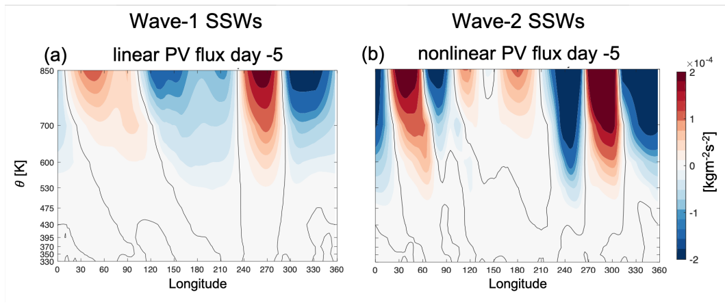
Figure 8. The longitude- \theta cross section of PV flux averaged north of 45^\circ N at day -5. (a) Linear PV flux for wave-1 SSWs and (b) nonlinear PV flux for wave-2 SSWs. Black line indicates the zero value of PV flux.
