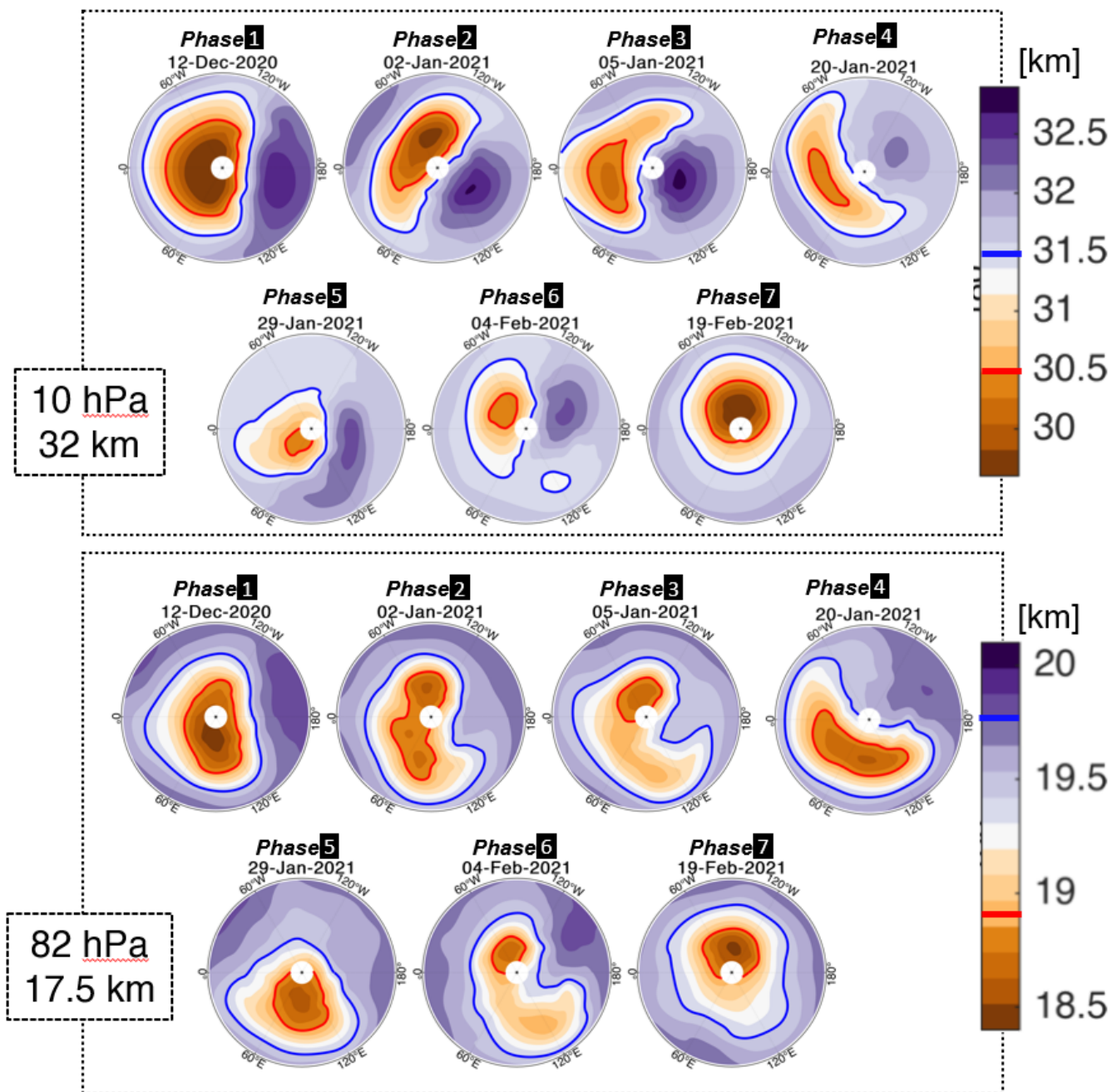
Figure 9. Maps of MLS (top) 10 hPa and (bottom) 82 hPa GPH in km for selected days. Selected contours have been highlighted in blue and red, with their locations indicated on the colour bars.
