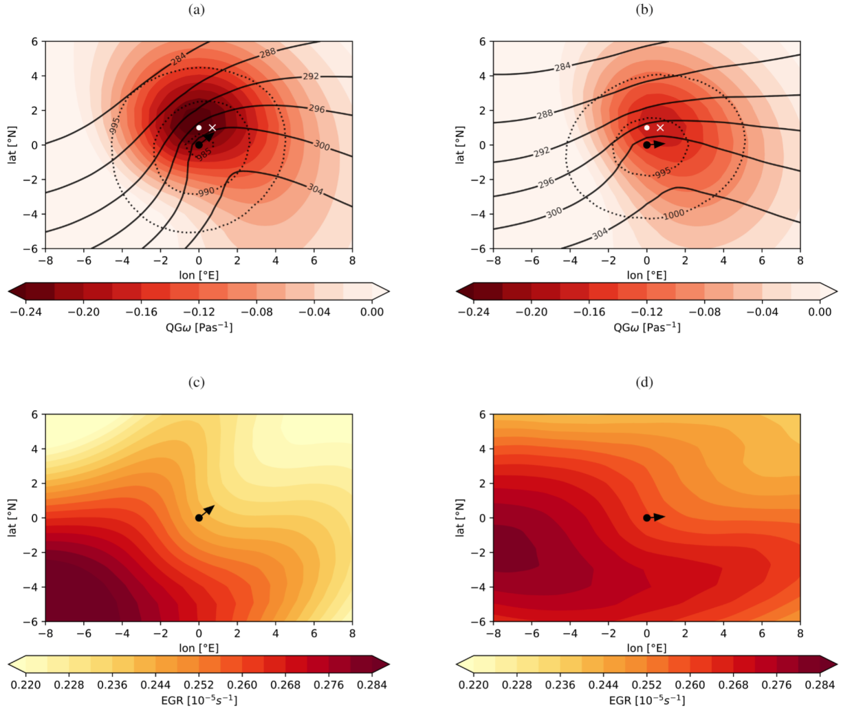
Figure 10. Cyclone-centered composites of \text{QG}\omega (coloured contours in \text{Pas}^{-1} ) for (a) poleward propagating cyclones ( 35^\circ < \alpha < 65^\circ ) and (b) eastward propagating ( -5^\circ < \alpha < 25^\circ ) cyclones, and EGR composites (coloured contours in 10^{-5}\text{s}^{-1} ) for (c) poleward propagating cyclones and (d) eastward propagating cyclones. The black dot represents the cyclone center and the arrow the mean 6-h propagation direction of the cyclone. The white dot in (a) and (b) indicates the maximum of the \text{QG}\omega forcing for poleward propagating cyclones and the white cross the \text{QG}\omega maximum for eastward propagating cyclones, i.e., they mark the exact location of color-shaded \text{QG}\omega fields. The white dot and cross are depicted both in (a) and (b) to highlight the spatial shift between the two forcing maxima. The black contour lines in (a) and (b) show \theta_e (in K) at 850 hPa, the dotted lines SLP (in hPa).
