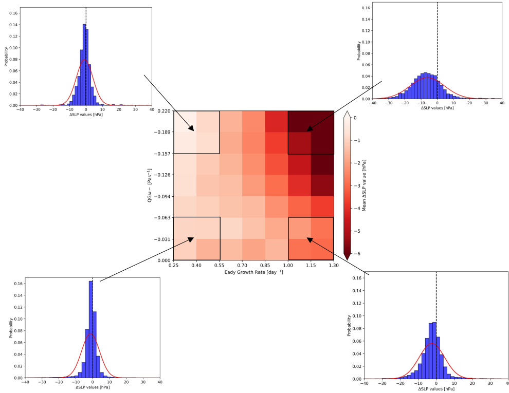
Figure 1. Exemplary 2D forcing histogram with EGR (in \text{day}^{-1} ) on the x-axis and QG\omega (in \text{Pas}^{-1} ) on the y-axis. Colours show the mean \Delta\text{SLP} value for each bin (darker (lighter) red highlights bins containing time intervals with stronger (weaker) mean deepening rates ( \Delta\text{SLP} )). For every corner of the histogram (framed in black, consisting of 2 \times 2 bins), the distribution of \Delta\text{SLP} values is shown. The four boxes are used to define four forcing categories: Q\downarrow E\downarrow , Q\downarrow E\uparrow , Q\uparrow E\downarrow and Q\uparrow E\uparrow (see text for details).
