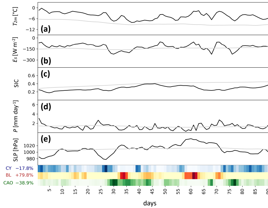
Figure 9. Time series of daily-mean (a) T_{2m} (in ^{\circ}\text{C} ), (b) E_s (in \text{W m}^{-2} ), (c) SIC and, (d) P (in \text{mm day}^{-1} ) and (e) sea-level pressure (SLP, in hPa) averaged in the region of the Kara-Barents Seas Kara and Barents Seas (KBI, KBM, and KBS) in DJF 2011/12 (black lines). The transient climatology is shown by grey lines. Blue, orange, and green heatmaps at the bottom of the figure show the daily-mean coverage of the region by cyclones, blocks, and CAOs, respectively (the darker the color the higher the coverage). Relative frequency anomalies of the three weather systems are given in percentages. The horizontal axis indicates days since the start of the season with day 1 corresponding to 01 December.
