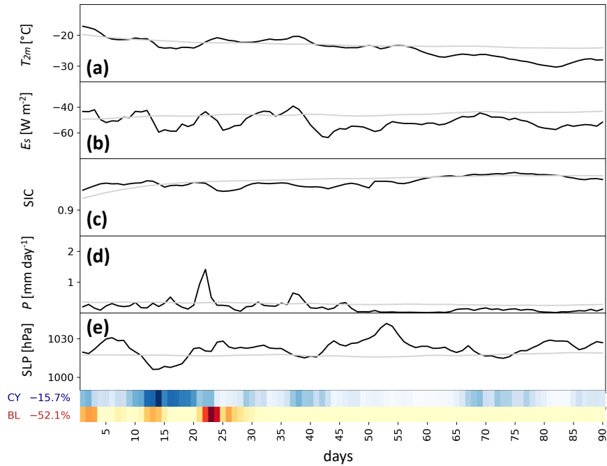
Figure 14. Time series of daily-mean (a) T_{2m} (in ^{\circ}C ), (b) E_S (in W m^{-2} ), (c) SIC, (d) P (in mm day^{-1} ) and (e) sea-level pressure (SLP, in hPa) averaged in the sub-region ARI in DJF 2012/13 (black lines). The transient climatology is shown by grey lines. Blue and orange heatmaps at the bottom of the figure show the daily-mean coverage of the region by cyclones and blocks, respectively (the darker the color the higher the coverage). Relative frequency anomalies of the two weather systems are given in percentages. The horizontal axis indicates days since the start of the season with day 1 corresponding to 01 December.
