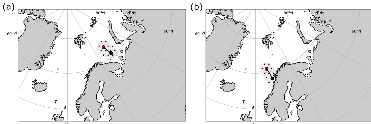
Figure B1. Examples of randomly generated pseudo-events to test performance of diagnostic indices. (a) one of the pseudo-events generated in winter 2003 (b) one of the pseudo-events generated in winter 2007. Pseudo-events are defined at randomly selected times and locations when no PL was observed to test if diagnostic indices are useful for distinguishing occurrence and non-occurrence of PLs.
