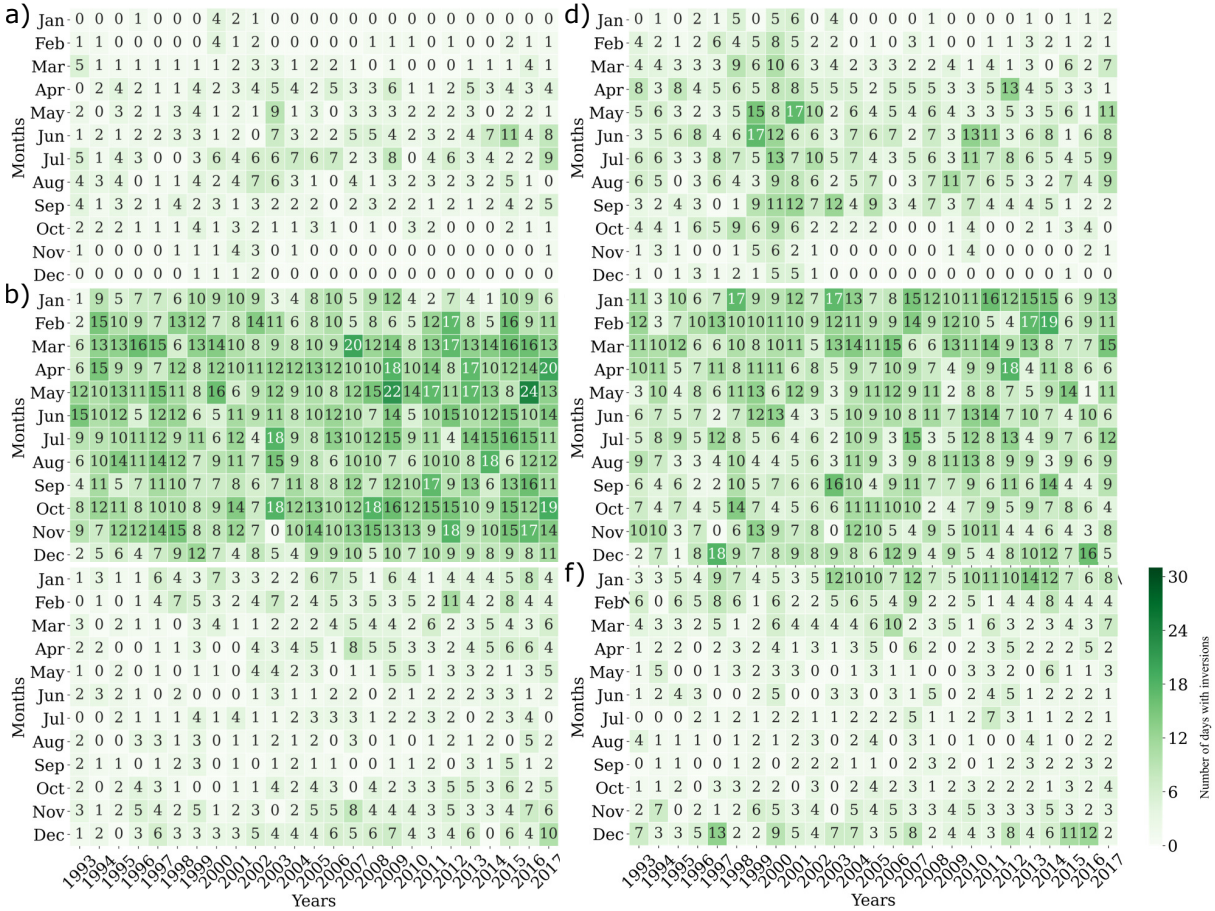
Figure S2. Monthly distribution of days with humidity inversions between 1993-2017 at the three different levels (first level: a and d; second level: b and e; third level: c and f) for cyclonic (a,b,c) and non-cyclonic (d,e,f) conditions
