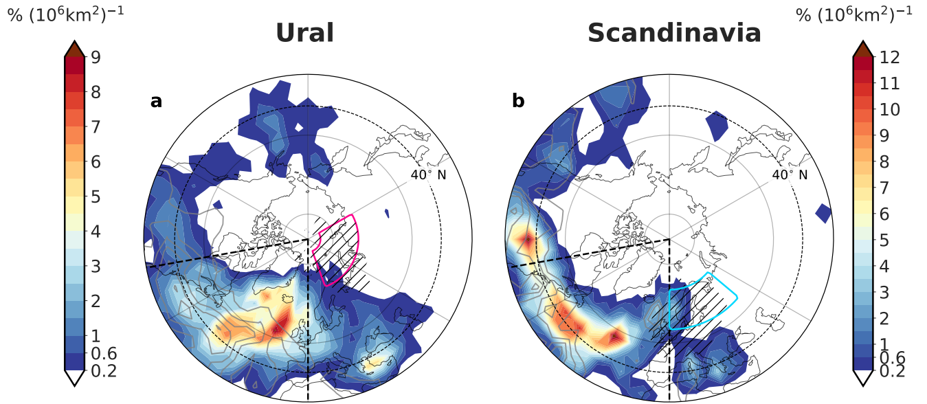
Figure 10. Spatial distribution of the locations of maximum heating for the trajectories within the heating regime initialized from Ural (a) and Scandinavian (b) blocks. Shading shows the density of trajectories at the time of maximum 6-hourly heating, defined as the percentage of the total number of heated trajectories per unit area (here 5^\circ \times 5^\circ ). The gray contours show the locations of the trajectories six days prior to arrival into the blocking region (normalized area-weighted density, shown every 1, starting from 1 \% (10^6 \text{ km}^2)^{-1} ). The magenta box in (a) and the cyan box in (b) show the Ural and Scandinavian sector, respectively, where the hatched regions indicate the main backward trajectory starting locations within the blocks (normalized area-weighted density > 5 \% (10^6 \text{ km}^2)^{-1} ). The main heating domain is denoted by the black dashed lines and the black dashed circle shows the latitude line at 40° N.
