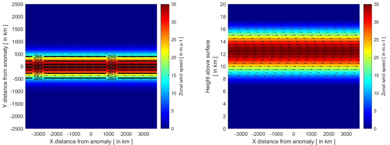
150 Figure 3: The jet stream of the model setup. Left: The zonal wind speed of the jet stream at the height of given model tropopause (12500m AGL). Pressure contours (in hPa) are overlaid together with zonal wind quivers. Right: A cross-sectional view of the zonal wind associated with the jet stream through the centre of the domain overlaid with zonal wind quivers.
