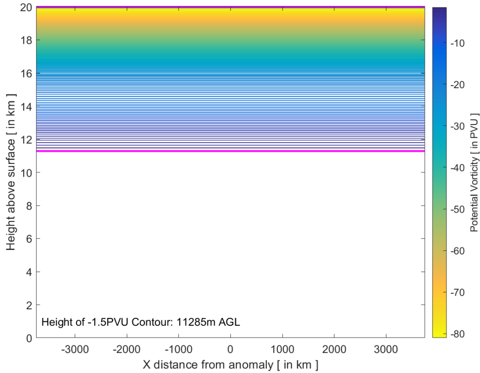
145 Figure 2: PV zonal cross-section through the centre of the domain. The -2 PVU tropopause was specified at a height of 12500m AGL. The -1.5 PVU contour (highlighted in a thick magenta line) was calculated to be 11285m AGL. A contour interval of 0.5 PVU is used.
