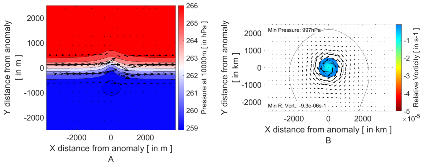
240 Figure 6: A: Upper-level (10000m AGL, 2500m below the experimentally defined dynamical tropopause) pressure field (shaded) together with wind vectors plotted as black arrows. B: Surface pressure isobars (black lines) and surface relative vorticity (shaded) together with surface wind vectors plotted as black arrows.
