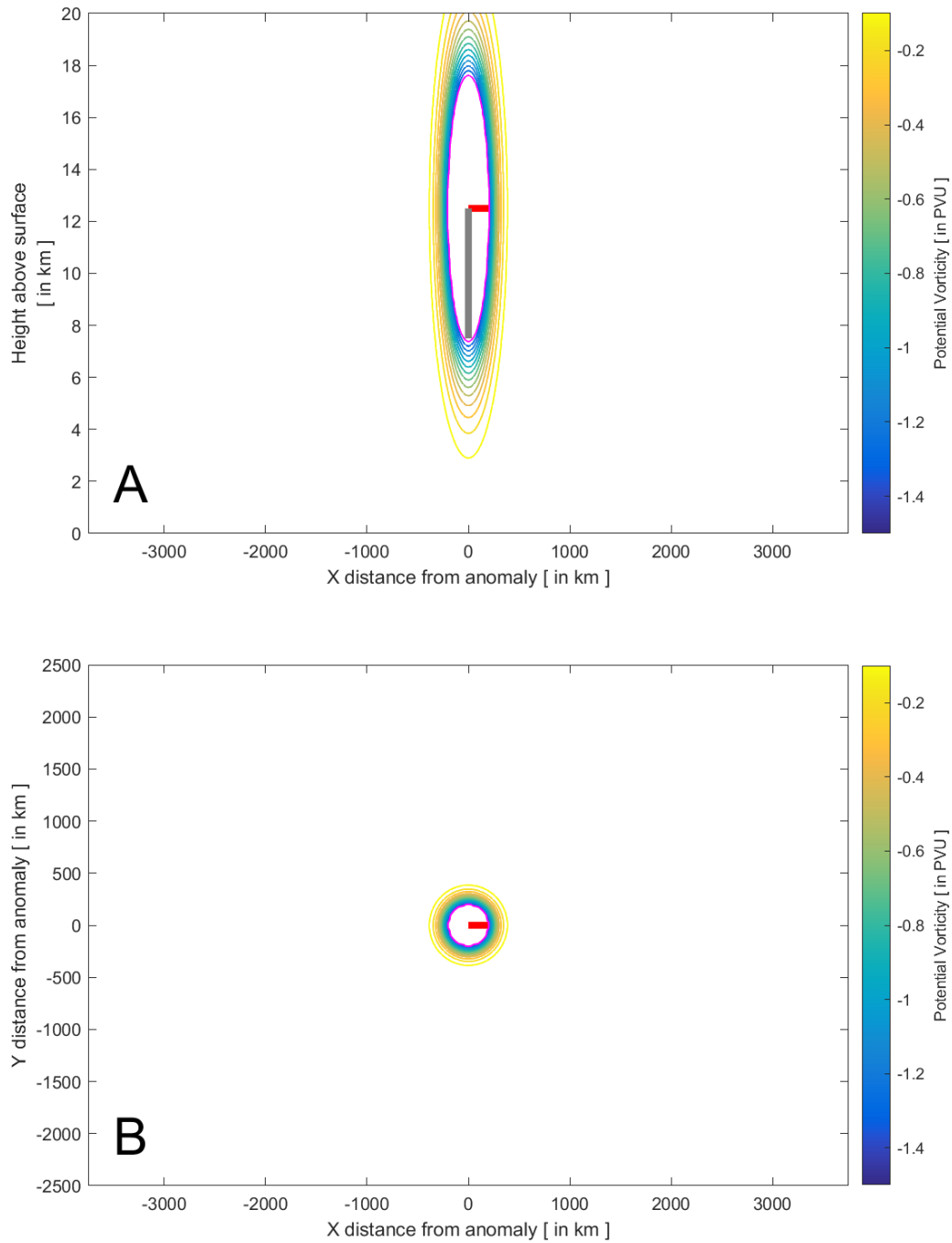
170 Figure 4: Example of a PV anomaly forced into the idealised domain by means of a longitudinal cross section (A) and a horizontal cross-section (B) through the centre of the anomaly. The anomaly has a maximum horizontal width along the minor axis of 400km and a height of 10000m. This excludes the "halo" of decreasing values to zero around it. The red line is defined as the anomaly radial width ( x_{size}, y_{size} ), whilst the grey line is defined as the anomaly radial height ( z_{size} ). The anomaly magnitude (in this case -1.5 PVU) is shown by the magenta contour.
