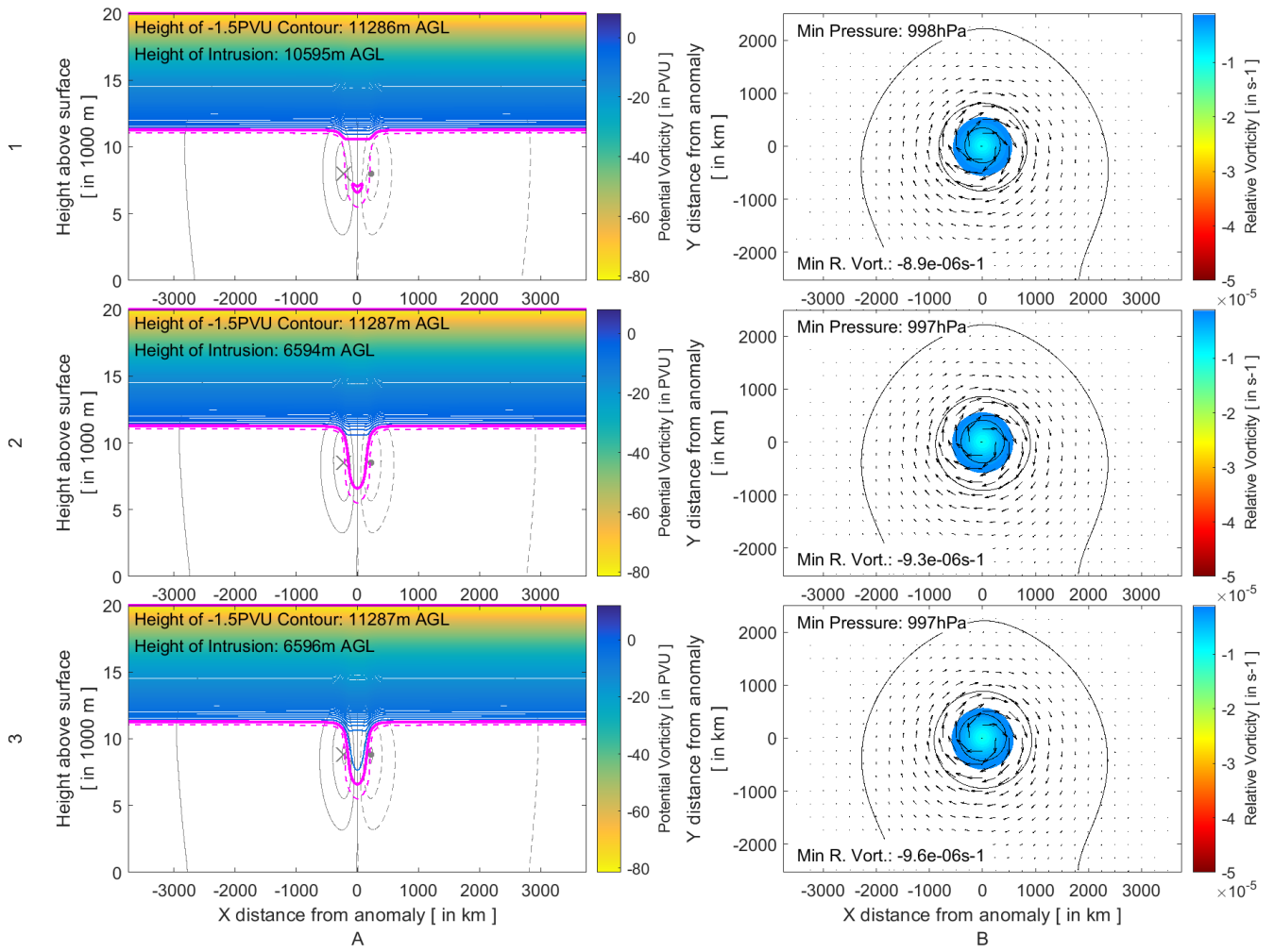
415 Figure 12: Same as in Experiment 0 with varying anomaly magnitudes of -1.0 PVU (row 1) and -2.0 PVU (row 3). Experiment 0 (with an anomaly magnitude of -1.5 PVU) is shown in row 2. In addition to the -1.5 PVU contour (thick magenta line), the -1.0 PVU contour is also provided for context by a dashed magenta line.
