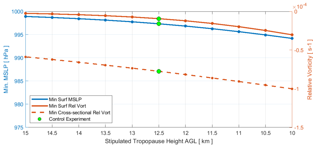
365 Figure 10: Similar to Figure 8 but for Experiment 2 (varying tropopause height experiments) with tropopause height AGL shown on the x-axis
