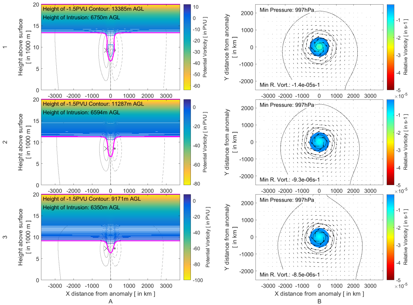
390 Figure 11: Same as in Figure 7 but with variable anomaly radial heights such that the height of the stratospheric intrusions AGL are similar from varying tropopause heights of 15000m (row 1) and 10000m (row 3). Experiment 0 is given in row 2 for ease of reference.
