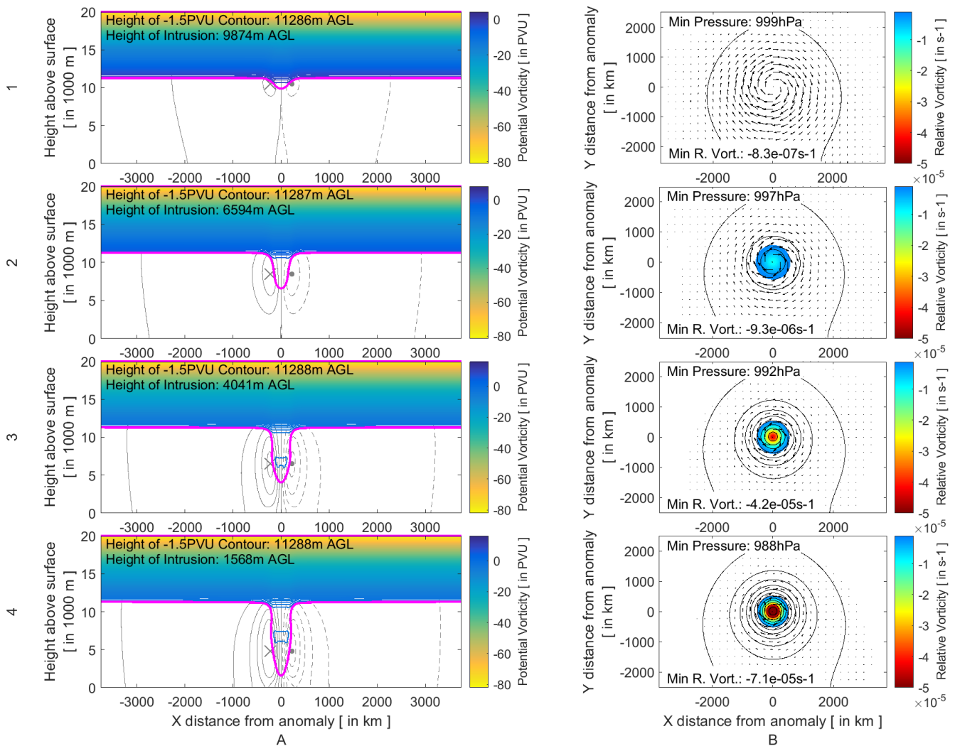
290 Figure 7: A: Longitudinal PV cross-sections through the centre of the forced anomaly. The -1.5 PVU contour (our definition of the dynamical tropopause for this study) is highlighted in by a thick magenta line. Meridional wind velocities are given in 4m.s^{-1} intervals shown by grey contours. Positive velocities (into the page) are represented by solid contours whilst negative velocities are represented by dashed contours (out of the page). B: The effect of the intrusion on the surface pressure and relative vorticity are shown in the right panels. Pressure isobars at a 1hPa contour interval are shown by black lines, whilst relative vorticity is shown by the shading. The panels in rows 1-4 represent different varying stratospheric depths introduced into the domain. For this experiment (Experiment 1), radial anomaly depths given to the system are 2500m (row 1), 5000m (row 2), 7500m (row 3) and 10000m (row 4). 295 By convention, in-text figure references refer to the column letter and the row number of the panel referenced (ie B2 refers to the panel in column B and row 2)
