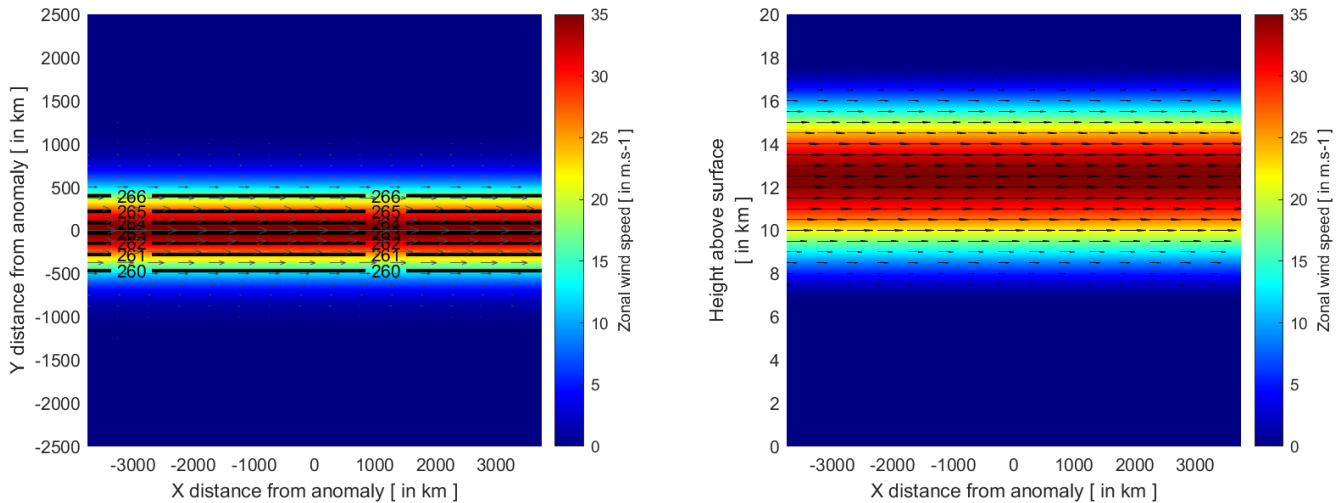
Figure 3: The jet stream of the model setup. Left: The zonal wind speed of the jet stream at the height of given model tropopause (12500m AGL). Pressure contours (in hPa) are overlaid together with zonal wind quivers. Right: A cross-sectional view of the zonal wind associated with the jet stream through the centre of the domain overlaid with zonal wind quivers.
