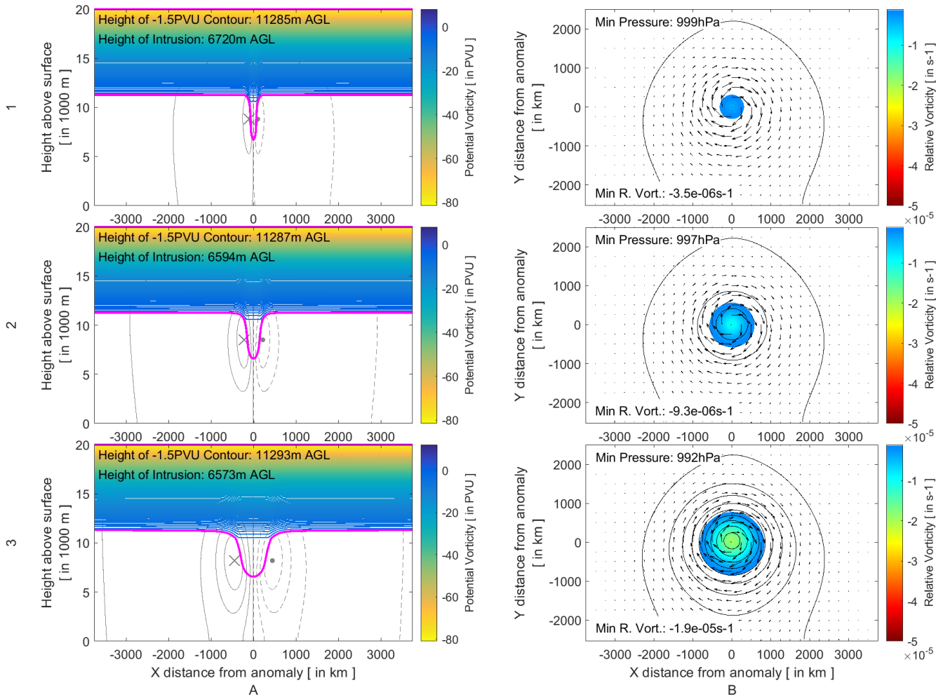
460 Figure 14: Same as in Figure 7 but with variable anomaly radial widths such that the height of the stratospheric intrusions AGL are similar from a constant dynamical tropopause depth of 12500m. The thinner intrusion is created by an anomaly with a 100km radial width (row 1) whilst the broader intrusion is created by a 400km radial width (row 3). Experiment 0 (200km radial width) is provided in row 2 for convenience and comparison.
