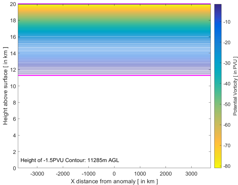
Figure 2: PV zonal cross-section through the centre of the domain. The -2 PVU tropopause was specified at a height of 12500m AGL. The -1.5 PVU contour (highlighted in a thick magenta line) was calculated to be 11285m AGL. A contour interval of 0.5 PVU is used.
