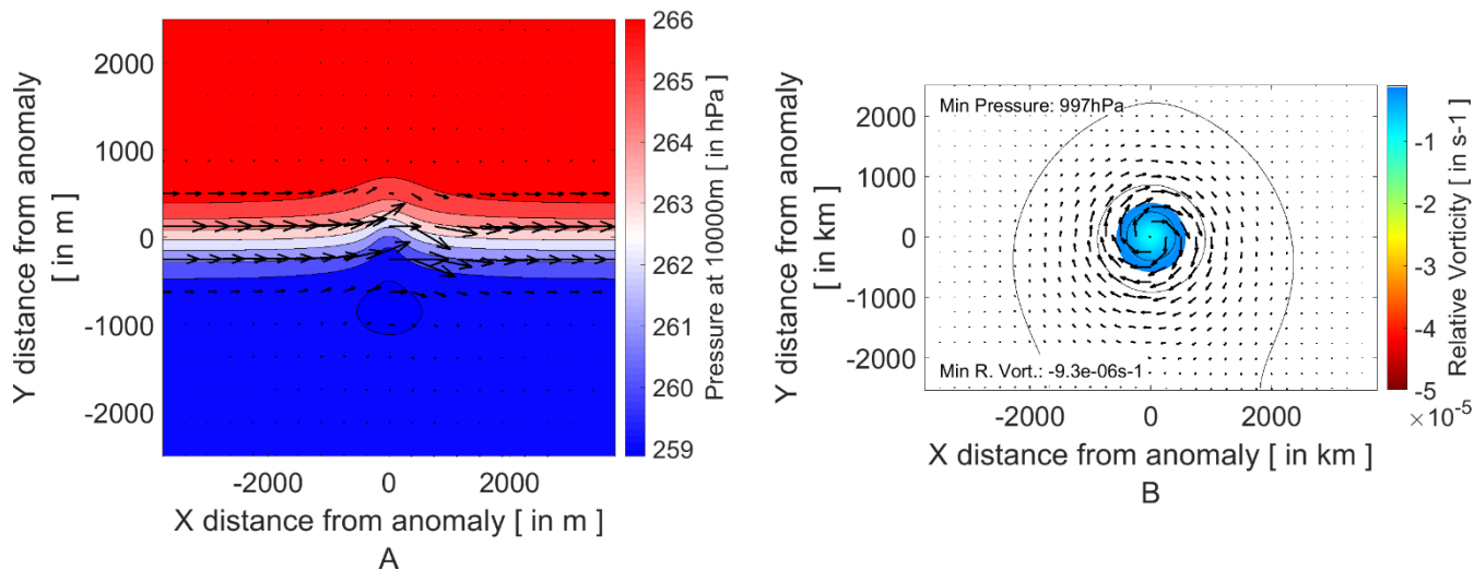
Figure 6: A: Upper-level (10000m AGL, 2500m below the experimentally defined dynamical tropopause) pressure field (shaded) together with wind vectors plotted as black arrows.
