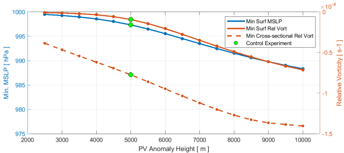
300 Figure 8: Changes to surface parameters (solid lines) as a function of anomaly radial height (depth of intrusion). The minimum MSLP (blue) and relative vorticity (orange) on the surface pressure level are recorded and plotted. The cross-sectional minimum relative vorticity as a function of anomaly depth is also shown by the dashed line. The results in Experiment 0 are highlighted in green for convenience.
