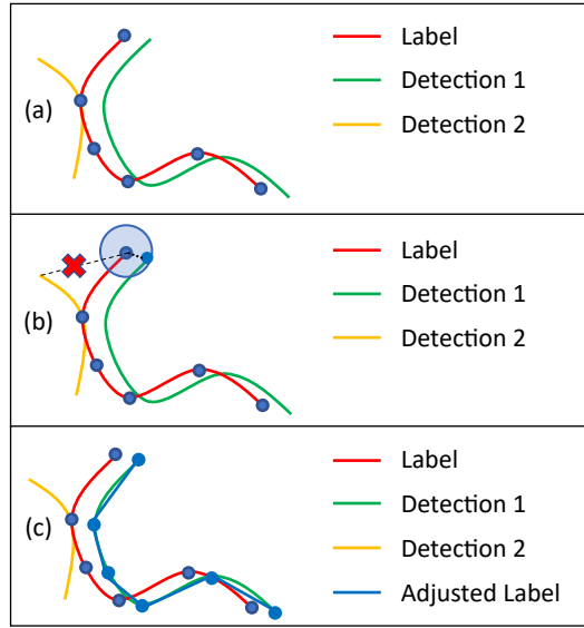
Figure 5. Sketch of our label adjustment method. (a) Initial Weather Service label with poly-line polyline vertices (blue dots) and 2 possible detections. Detection 1 initially scores lower than Detection 2 due to a lower intersection with Label. (b) Display of how a vertex of Label might be adjusted within a search radius for Detection 1. The possibly optimal position for the vertex regarding Detection 2 is not within the search radius of the vertex. Deformation will therefore not be able to create a good intersection of the upper part of Detection 2 and Label. A similar situation occurs for the three vertices at the bottom right of Label. (c) Possible resulting Adjusted Label after each Vertex was adjusted. The Label was deformed onto Detection 1 as it creates the best matching score. Detection 2 is too far from several vertices of Label and cannot score a similar matching score with any deformation of Label. As a result Detection 1 now scores higher than Detection 2.
