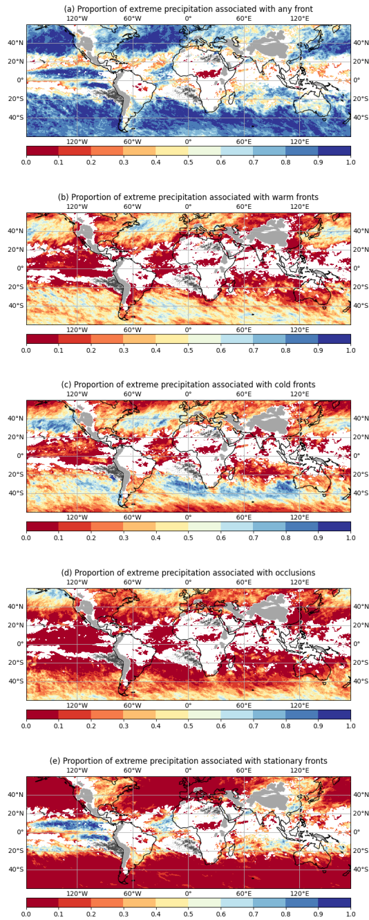
Figure 10. Proportion of extreme precipitation events, which are also associated with a front. High orography is masked as Regions with high topography are shaded in light gray, while areas where no extreme precipitation events occurred in 2016 are masked as shaded in dark gray. Regions where no significant correlation between extreme precipitation and fronts was found are blanked. Results are shown for (a) any front, (b) warm front fronts , (c) cold front fronts , (d) eeclusion occlusions , and (e) stationary front fronts .
