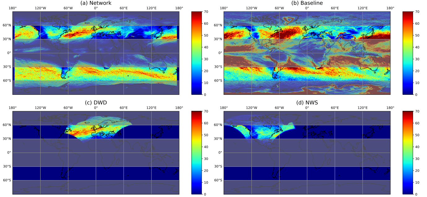
Figure 7. Global frontal climatologies as obtained derived from the ERA5 data set for the year 2016 – and climatologies from the ground truth data sets of the weather service service data-sets . (a) A global Global frontal climatology of from the Network network executed on the 0.25^\circ resolution grid and resampled to 0.5^\circ resolution. The network does not provide a valid prediction for the outer 5^\circ , as the effective output domain is smaller than the input domain. For this reason no fronts are displayed here. (b) A global Global frontal climatology of the baseline algorithm. Note that the algorithm is not designed for application outside the midlatitudes and should only be evaluated outside the gray overlayed shaded regions. (c) Climatology of the provided DWD Front front labels. (d) Climatology of the provided NWS Front front labels. Red denotes more than 70 fronts. The represented front count was clipped at 70 for visual representation, regions with higher front counts are shown in red . Stationary Fronts fronts are explicitly excluded from the climatology of the network generated data and NWS labeled data. The global climatology from the baseline algorithm does not include fronts propagating at less than 3 \text{ m s}^{-1} . The DWD data-set may include stationary fronts, as we were unable to reliably separate them from warm or cold fronts.
