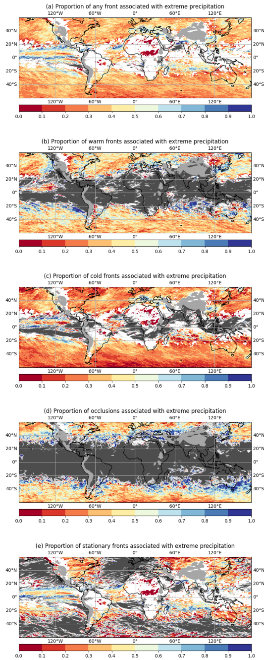
Figure 12. Proportion of fronts, which are associated with an extreme precipitation event. High orography is masked as Regions with high topography are shaded in light gray, while areas where no fronts of the corresponding class were detected in 2016 are masked as shaded in dark gray. Regions where no significant correlation between extreme precipitation and fronts was found are blanked. Results are shown for (a) any front, (b) warm frontfronts , (c) cold frontfronts , (d) occlusion occlusions , and (e) stationary frontfronts .
