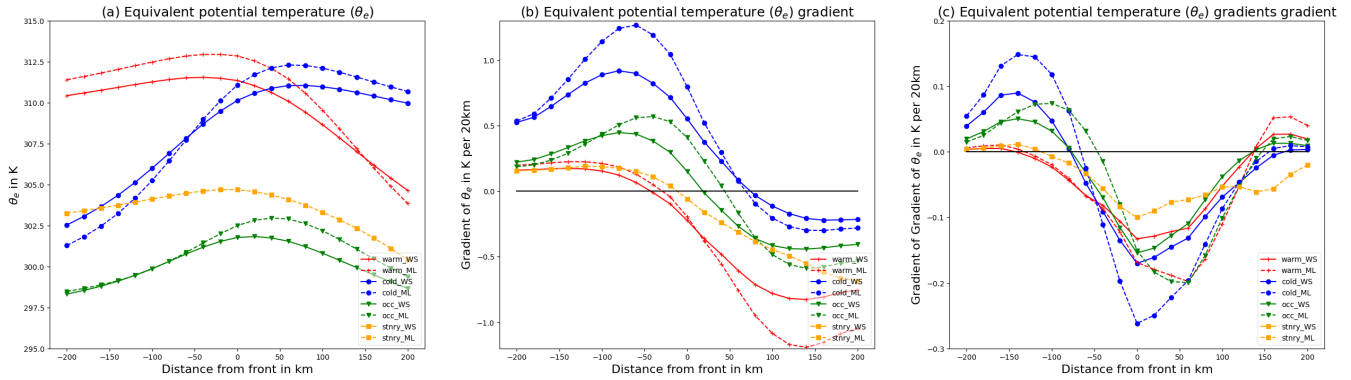
Figure 8. Average value of variables at 850hPa across-front across fronts in direction of wind. Mean of (a) Mean of the equivalent potential temperature ( \theta_e ), (b) \theta_e -gradient and (c) gradient of \theta_e -gradient of provided with front positions determined by DWD manual analysis (solid, WS) and by our network generated (dashed, ML) front labels for the DWD Data . For (b) and (c) we additionally display the 0 level.
