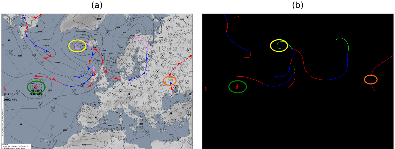
Figure 3. Example of badly extracted fronts (b) from an image as-provided by the DWD (a) (Source: DWD). Green Circle: Object that is not a front, but has the same color coding, is wrongly extracted as a front. Orange Circle: Unrelated symbol is drawn over the front. The front could not be extracted completely. Yellow Circle: Frontal symbol is placed in an area with high curvature. The curvature is not extracted exactly, as the symbol is removed during the procedure and the loose ends are connected with a straight line.
