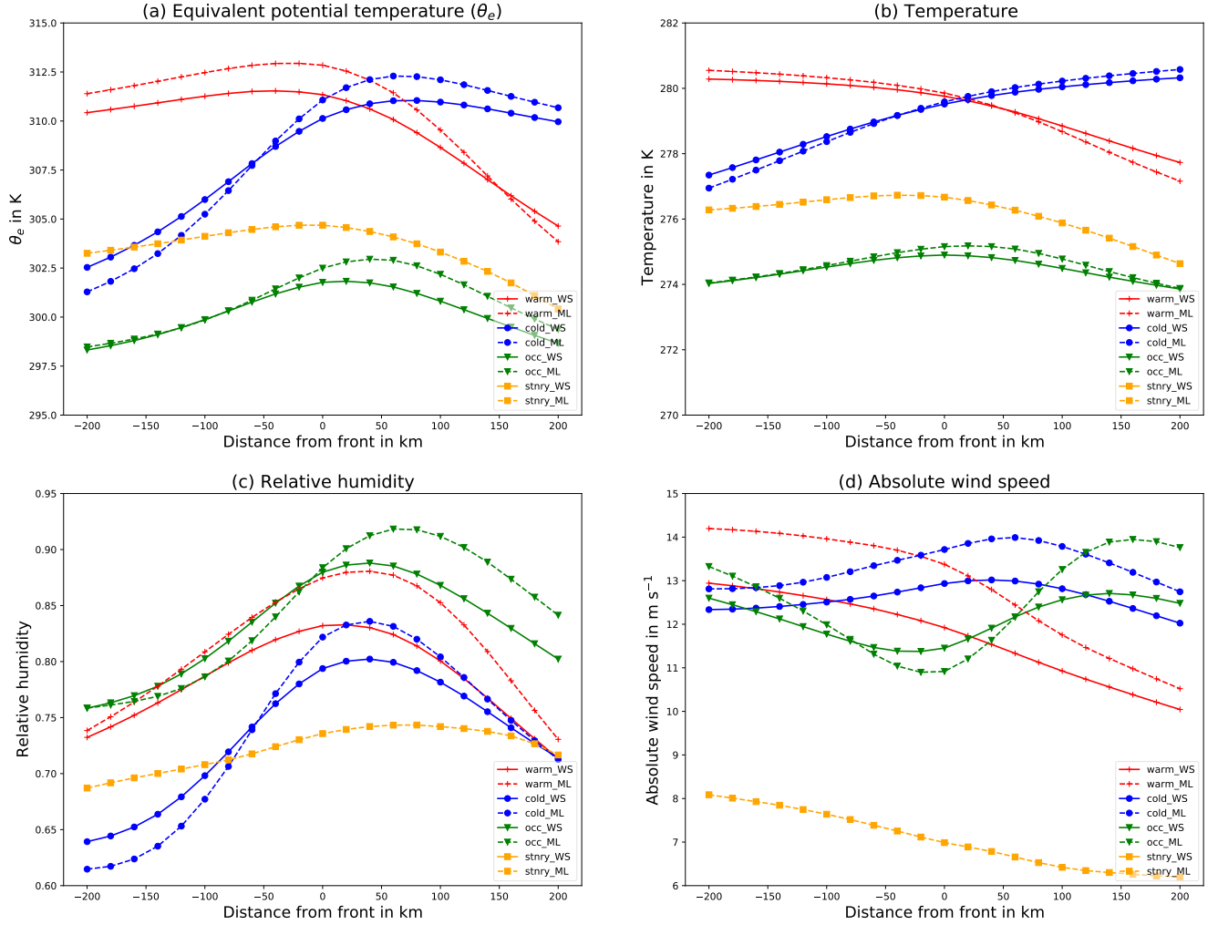
Figure 9. Average value of variables at 850hPa across-across front in direction of wind. (a) Mean of the equivalent potential temperature ( \theta_e ), (b) temperature, (c) relative humidity and (d) absolute wind speed of provided with front positions determined by DWD manual analysis (solid, WS) and by our network generated (dashed, ML) front labels for the DWD Data .
