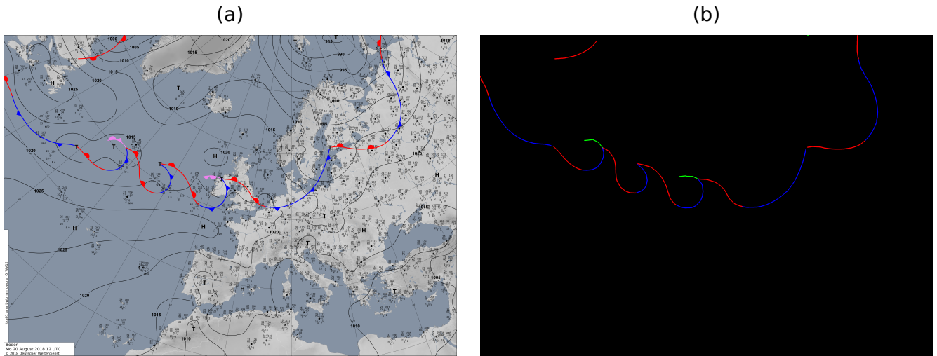
Figure 2. Example of well extracted fronts (b) from an image as-provided by the DWD (a) (Source: DWD). Blue -In panel (b) blue and red lines correspond to cold and warm fronts respectively-as in the original images. Green -image (a), green lines correspond to the occlusions which are pink in the input image. Note that stationary fronts are originally depicted as alternating warm and cold fronts. For this reason we cannot distinguish those from regular cold and warm fronts.
