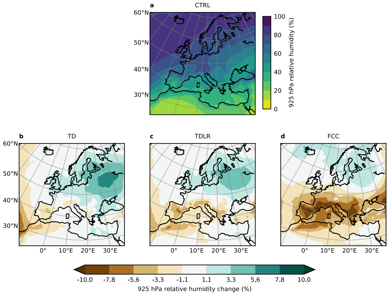
Figure 4. Mean summer relative humidity in the historical CTRL simulation and changes in the idealized simulations. (a) Climatological relative humidity in CTRL for the average summer in the 1971-2000 period. (b) Change in relative humidity in the idealized TD simulation, representing RCP8.5 and the 2070-2099 period. (c) Same as (b) but for TDLR. (d) Same as (b) but for the FCC, which is the GCM-driven transient regional climate simulation.
