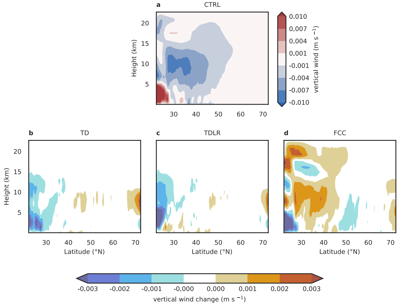
Figure 5. Meridional cross-section of mean summer vertical wind (positive values mean upward motion) in the historical CTRL simulation and changes in the idealized simulations. (a) Vertical velocity in CTRL for the average summer in the 1971-2000 period. (b) Change in vertical in the idealized TD simulation, representing RCP8.5 and the 2070-2099 period. (c) Same as (b) but for TDLR. (d) Same as (b) but for the FCC, which is the GCM-driven transient regional climate simulation. This figure shows only data from the simulations based on the GCM HadGEM2-ES since the necessary three-dimensional model output was only stored for these simulations.
