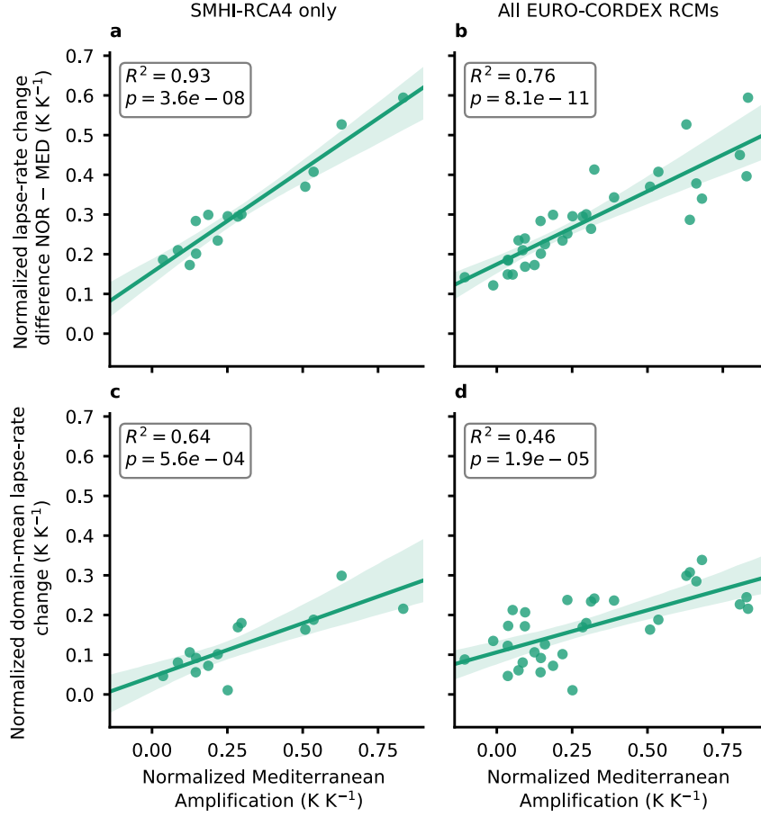
Figure 7. Linear regression linking the enhanced Mediterranean summer 2-m warming to lapse-rate changes in the EURO-CORDEX ensemble. (a,b) Regression linking the Mediterranean amplification and differences in lapse-rate changes between Northern Europe (NOR) and the Mediterranean (MED) over land. (c,d) Regression linking the Mediterranean amplification to the European-scale domain-mean lapse-rate change. (a,c) A subset of the EURO-CORDEX ensemble using one single regional climate model, namely SMHI-RCA4. (b,d) All EURO-CORDEX simulations that were used in this study (Table A1). Each dot represents a simulation with a horizontal resolution of 0.11^\circ or 0.44^\circ . The figure is based on summer-mean (JJA) changes between 1971-2000 and 2070-2099, assuming RCP8.5. We normalized both the Mediterranean amplification and lapse-rate changes with the domain-mean warming, yielding dimensionless values ( K/K ). The lapse-rate changes have been computed as the difference between the 500 hPa warming and the 850 hPa warming. We evaluate the Mediterranean between 30^\circ and 44^\circ N and Northern Europe between 55^\circ N and 70^\circ N. The boxes in the upper left corner of the panels show the statistics of the linear regression fit, while the shadings show the 95% confidence interval of the linear regression estimated by 1000-fold bootstrapping.
