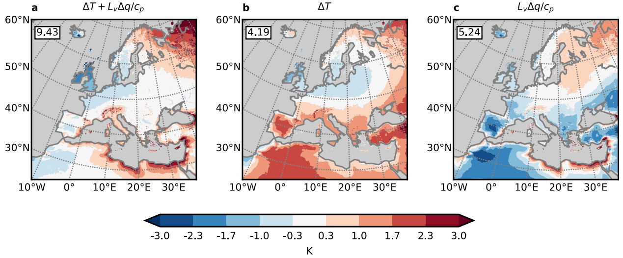
Figure 6. Decomposition of the anomaly of surface moist enthalpy ( H ) changes in the 0.11^\circ EURO-CORDEX ensemble for the summer season over land. (a) Overall anomaly (deviation from the domain mean) of the change in moist enthalpy, normalized by the specific heat of air ( c_p ) to yield the unit Kelvin. Thus, the surface moist enthalpy change has been computed as \Delta H = \Delta T + L_v \Delta q / c_p . The anomalies of the two components of H are shown separately. (b) shows the anomaly of \Delta T , while (c) shows the anomaly of L_v \Delta q / c_p . Gray shading shows ocean areas which are masked to improve the clarity.
