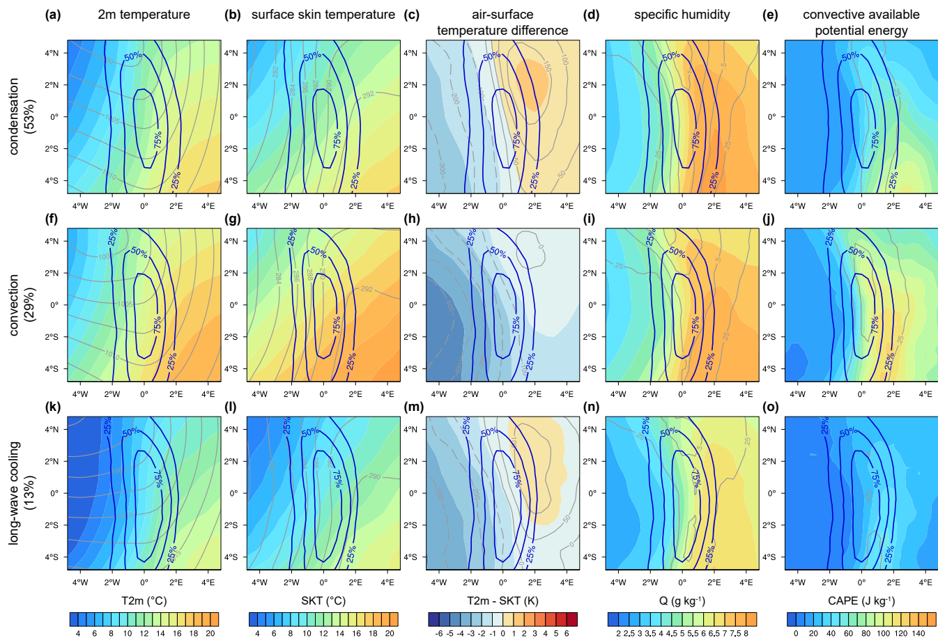
Figure 7. Composites of the environmental conditions along the cold front averaged over the 24 h period of most rapid cyclone intensification for subsets of the 144 extratropical cyclones in of the cold season. Rows represent different cyclone categories based on the primary process that produces the positive PV anomaly along the cold front (Fig. 4a). Depicted are surface fields, except for specific humidity which is shown at 900 hPa. Blue contours indicate average cold front frequency while gray contours show sea level pressure (first column), \theta at 900 hPa (second column), surface sensible heat flux (third column), large-scale precipitation (fourth column), and convective precipitation (last column).
