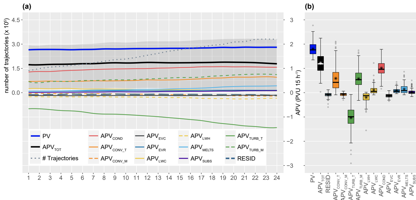
Figure 3. Physical processes that contribute to the positive PV anomaly ( PV \geq 1 PVU) in the cyclone center between the surface and 550550 hPa during the 24 h period of strongest-most rapid cyclone intensification. (a) Time series of APV averaged over the 144 cyclones in-of the cold season and (b) distribution of APV tendencies across-all-in individual cyclones averaged over the 24 h intensification period . The interquartile range is shown by the boxes, the whiskers extend 1-5-1.5 times the interquartile range, the median is shown by the bold horizontal line, the mean by the star, and outliers are shown as open circles.
