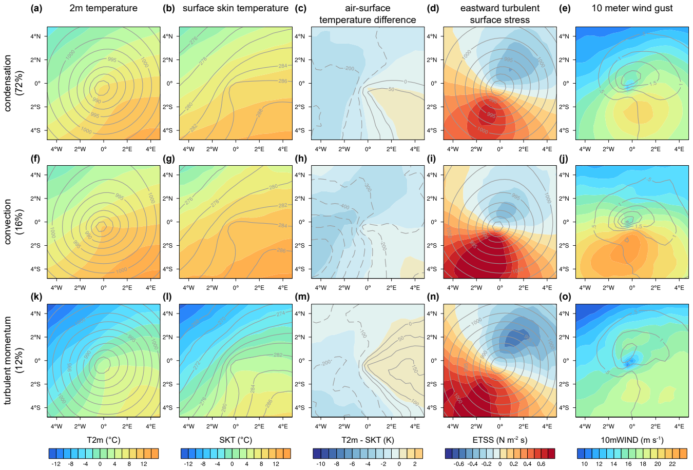
Figure 9. Similar to Fig. 7, but for the positive PV anomaly in the cyclone center in the cold season. Gray contours show sea level pressure (first and fourth column), \theta_{\text{on-at}} 900 hPa (second column), surface sensible heat flux (third column), and total precipitation (last column).
