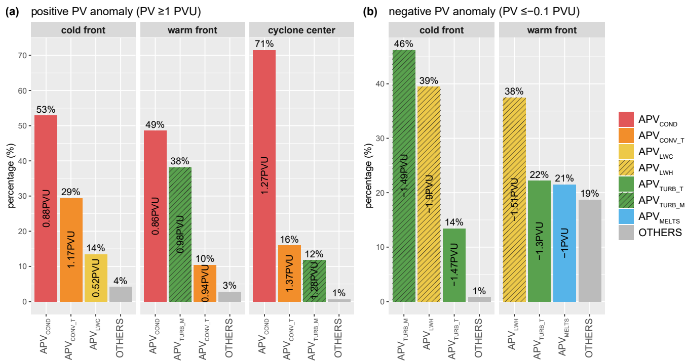
Figure 4. Prevalence of the dominant-most important processes for the generation of (a) the positive PV anomaly ( PV \geq 1 PVU) between the surface and 550 hPa and (b) the negative PV anomaly ( PV \leq -0.1 PVU) between the surface and 850 hPa during the cold season. Ranks are computed from the area-weighted mean APV of each process averaged over the entire 24 h period of most rapid cyclone intensification. Percentages indicate the fraction of cyclones with a specific process as the most important one and numbers . Numbers show the area-weighted mean APV averaged over all cyclones from the respective subset .
