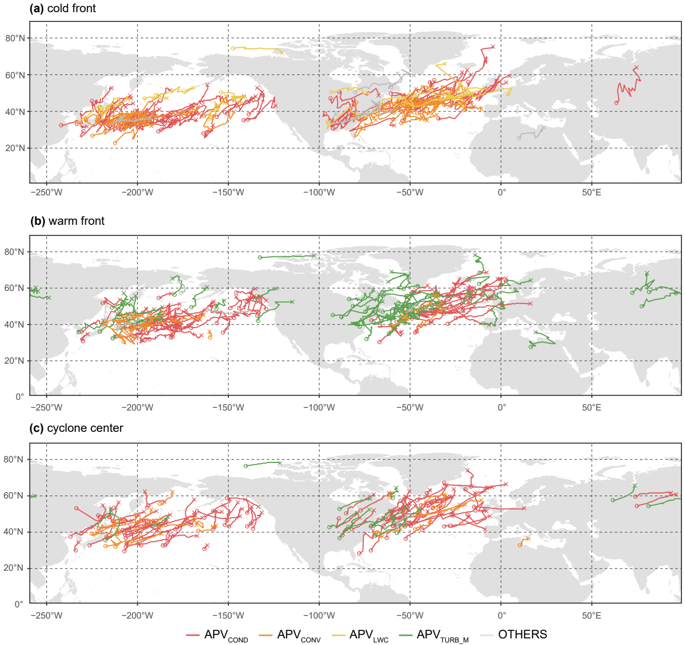
Figure 6. Geographical occurrence of (a) cold fronts, (b) warm fronts, and (c) cyclone centers for all cyclones from the cold season. Colors indicate the dominant primary physical process responsible for the generation of positive PV anomalies along the respective feature. Open circles indicate the beginning and crosses the end of the 24 h period of most rapid cyclone intensification.
