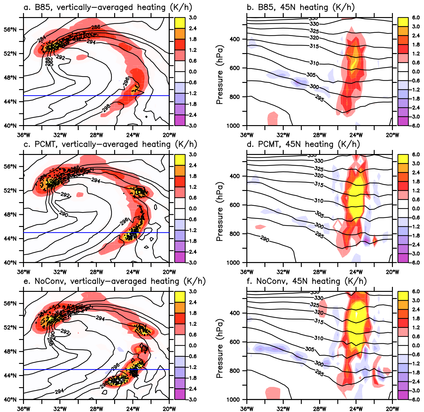
Figure 1. (Left panels) vertically-averaged heating rate between 300 and 800 hPa (shadings; units: \text{K h}^{-1} ), potential temperature at 850 hPa (int: 2 K) and WCB trajectories satisfying 100 hPa ascent in 2 hours at 21 UTC 1 October for (a) B85, (c) PCMT and (e) NoConv simulations. (Right panels) heating rate at 45°N (shadings; units: \text{K h}^{-1} ) and potential temperature (contours; int: 5 K) at 21 UTC 1 October for (b) B85, (d) PCMT and (f) NoConv simulations.
