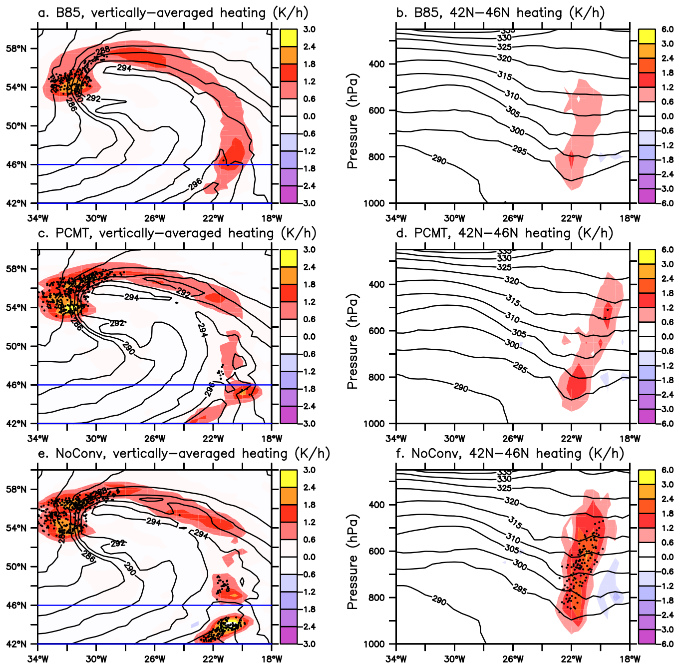
Figure 5. Same as figure 5 of the paper but at 03 UTC 2 October.
