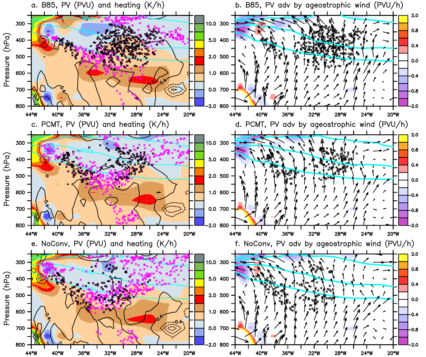
Figure 7. (Left panels) Latitudinally-averaged (63°N-65°N) PV (shadings; units: PVU), heating rate (black contours; int: 0.4 K h -1 ), potential temperature (light blue contours for 310, 315, 320 and 325 K) and WCB trajectories satisfying 25 hPa ascent in 2 hours (black crosses) and the other WCB trajectories (purple crosses) and located in the same latitudinal band at 12 UTC 2 October for (a) B85, (c) PCMT and (e) NoConv simulations. (Right panels) Latitudinally-averaged (63°N-65°N) PV advection by the zonal and vertical components of the ageostrophic wind (shadings; units: PVU h -1 ), and the associated ageostrophic wind vectors (black arrows). The light blue contours represent potential temperature as in left panels. The ageostrophic wind vectors are represented by multiplying respectively the zonal and vertical components by the distances occupied by 1 meter in longitude and 1 Pa in pressure on the diagram.
