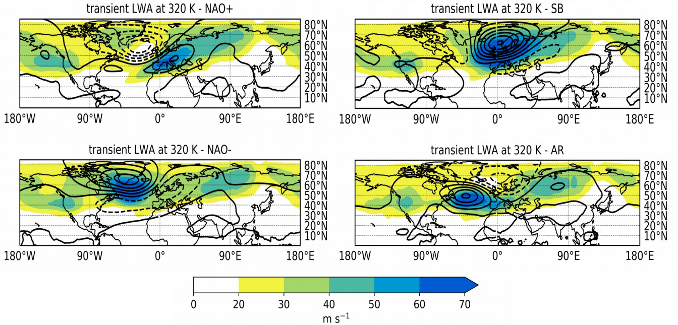
Figure 6. Transient LWA (colour, units \text{m s}^{-1} ) and Montgomery stream function anomalies (black contours every 100 \text{ m}^2 \text{ s}^{-2} , dashed contours represents negative values) at 320 K associated with the four WR over the EAT sector during winter in ERA5.
