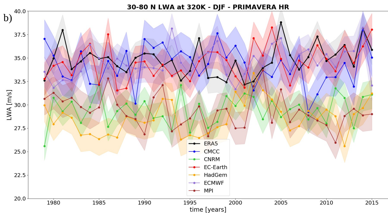
Figure 3. Time series of transient LWA averaged over the NH. Each dot represents the time averaged value for each winter season (DJF). Black line is ERA5, PRIMAVERA are in colour. Shading is the range between two standard deviations from the mean for each time series.
