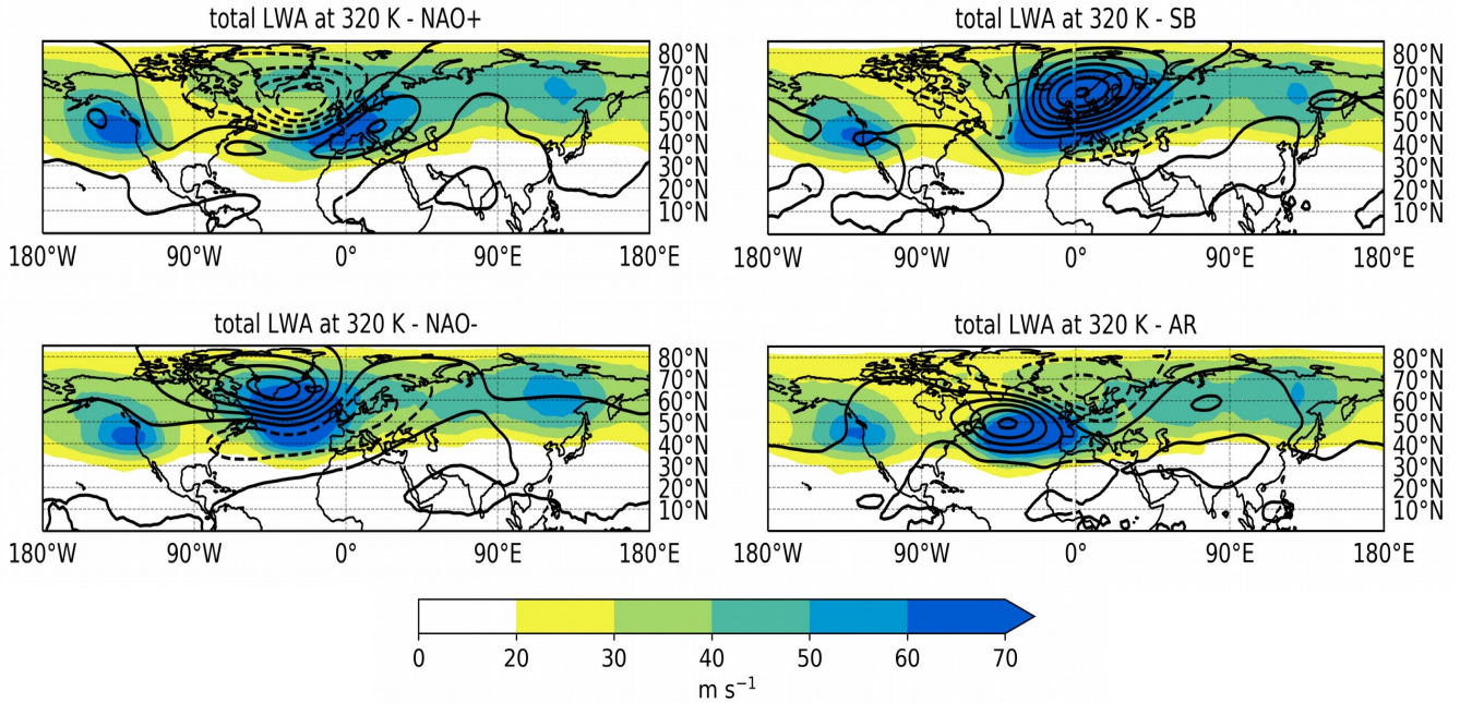
Figure 5. Total (i.e. stationary and transient) LWA (colour, units \text{m s}^{-1} ) and Montgomery stream function anomalies (black contours every 100 \text{ m}^2 \text{ s}^{-2} , dashed contours represents negative values) at 320 K associated with the four WR over the EAT sector during winter in ERA5.
