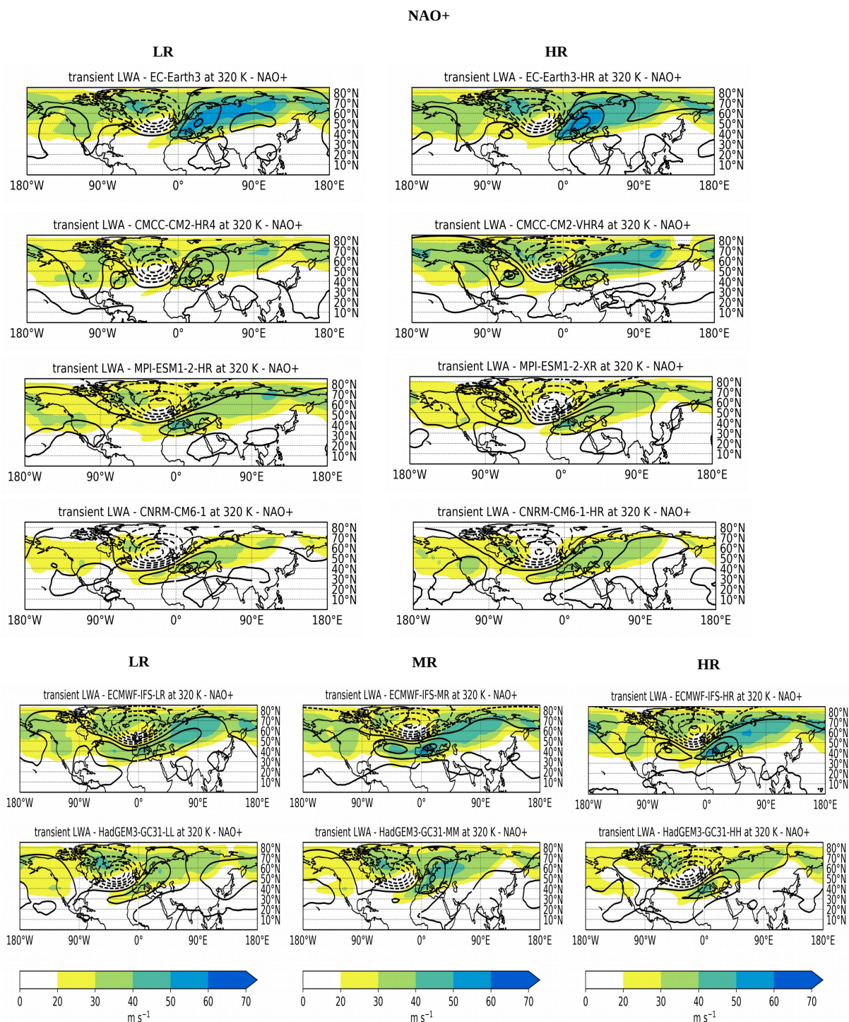
Figure 8. Transient LWA (colour, units \text{m s}^{-1} and Montgomery stream function anomalies (black contours every 100 \text{ m}^2 \text{ s}^{-2} , dashed contours represents negative values) at 320 K associated with NAO+ for PRIMAVERA.
