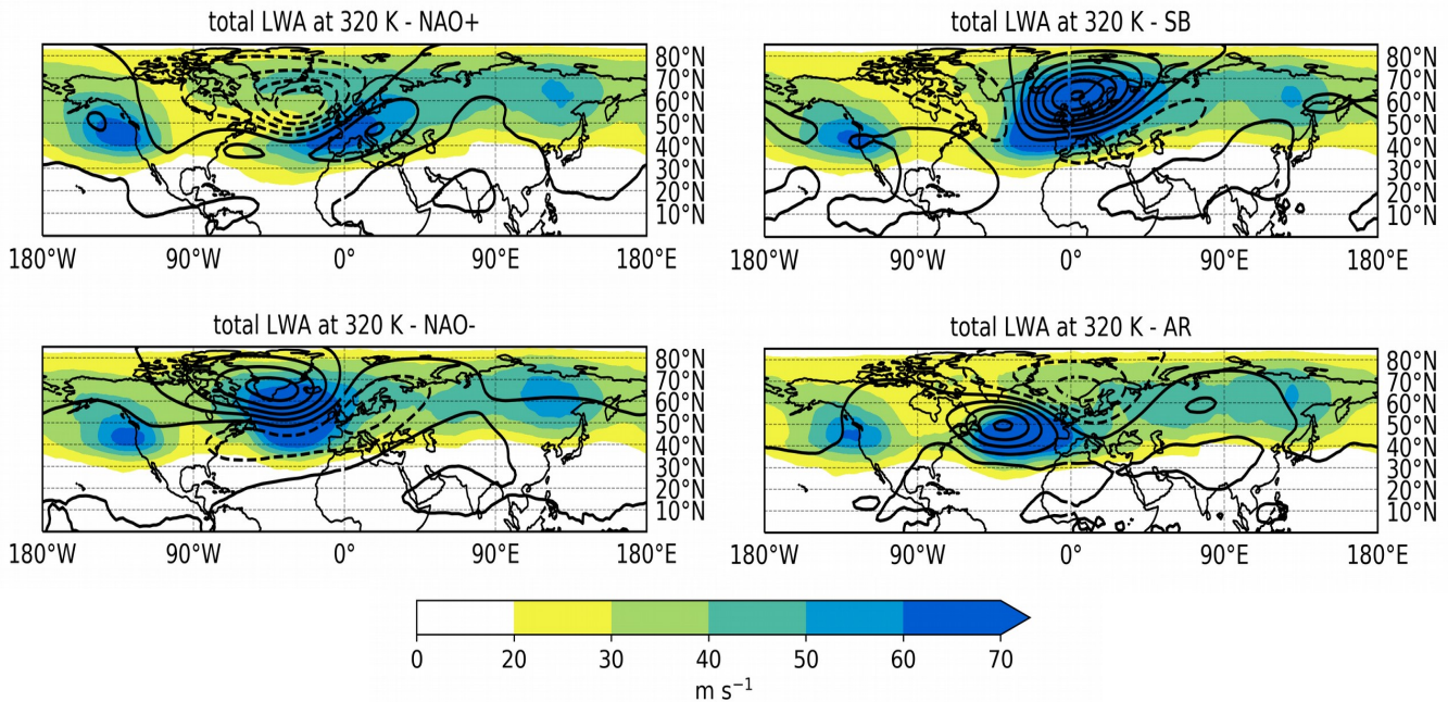
Figure 5. Total (i.e. stationary and transient) LWA (colour, units \text{m s}^{-1} ) and Montgomery stream function anomalies (black contours every 100 \text{ m}^2 \text{ s}^{-2} , dashed contours represents negative values) at 320 K associated with the four WR over the EAT sector during winter in ERA5.
