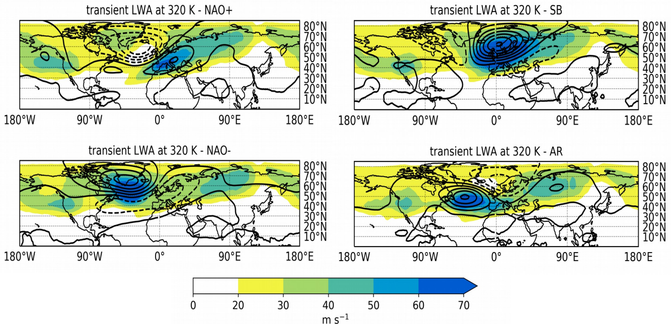
Figure 6. Transient LWA (colour, units \text{ms}^{-1} and Montgomery stream function anomalies (black contours every 100 \text{ m}^2 \text{ s}^{-2} , dashed contours represents negative values) at 320 K associated with the four WR over the EAT sector during winter in ERA5.
