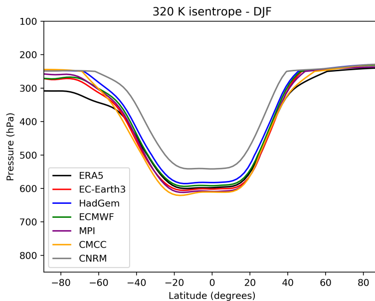
Figure A1. Pressure height (in hPa) of the 320 K isentropic surface (time-zonal mean for DJF). Black line is ERA5, other colours are PRIMAVERA LR simulations.
