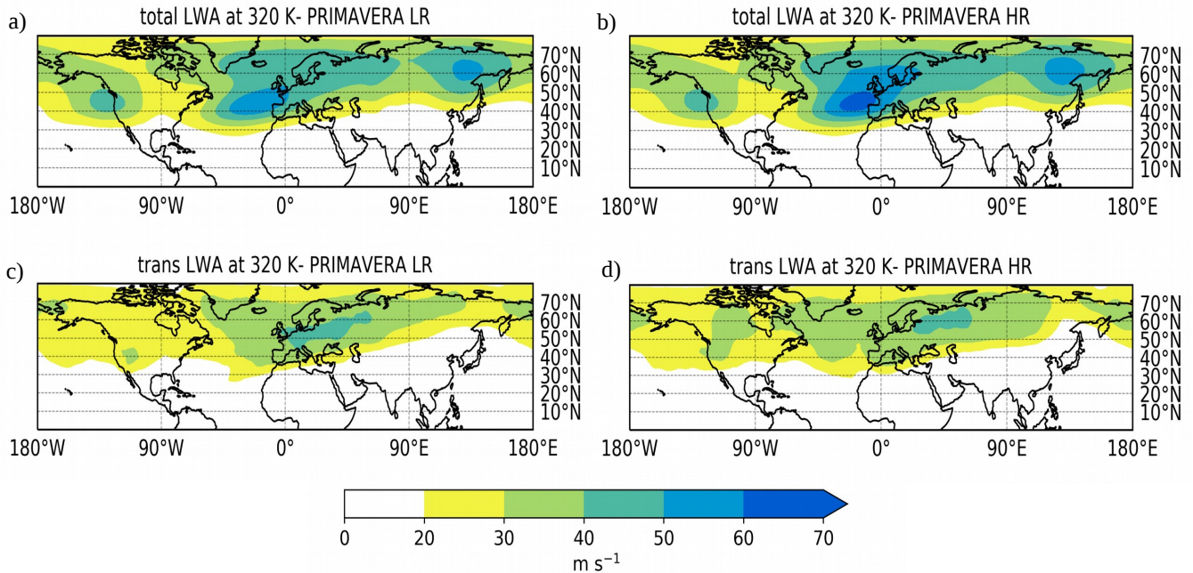
Figure 2. Multimodel mean of total LWA at 320 K for PRIMAVERA LR and HR (panels (a) and (b)) and for transient LWA (panels (c) and (d)).
