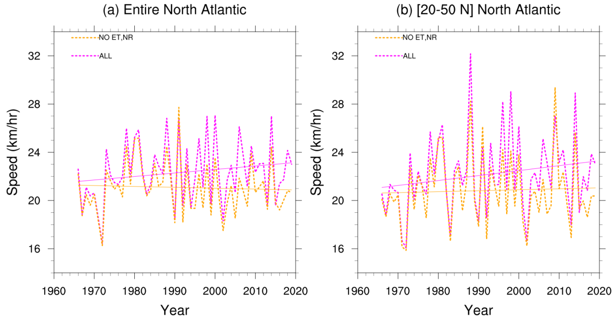
Figure 10. Annual-mean speed and linear trend for (a) The entire Atlantic; and (b) 20–50°N latitude band. The grey-magenta curve is for all storms in the IBTraCS dataset while the orange curve excludes instances when the storm was classified as ET or NR.
