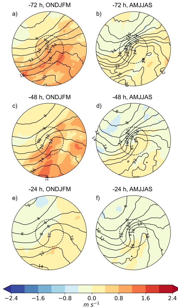
Figure 14. Sensitivity of the maximum 10-m wind gust to the TCWV (colours, \text{m s}^{-1} ), and the composite mean of TCWV (contours, 2 \text{ kg m}^{-2} interval) a,b) 72 h, c,d) 48 h, and e,f) 24 h before the occurrence of maximum 10-m wind gust in Northern Europe. The radius of the plots is 18^\circ and the 6^\circ radius is marked with a dashed circle.
