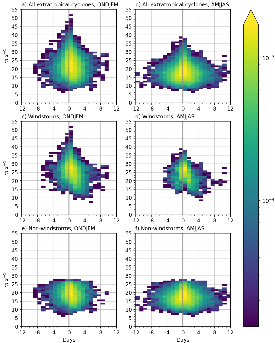
Figure 6. Normalized frequency of maximum 10-m wind gust ( \text{m s}^{-1} ) in Northern Europe (i.e. the maximum 10-m wind gust when the cyclone centre is inside the Northern Europe box) in relation to the time of the minimum mean sea level pressure (MSLP) during the cold season (left panel) and the warm season (right panel): a,b) all extratropical cyclones, c,d) windstorms, and e,f) non-windstorms. Zero on the x-axis indicates the time when the minimum MSLP during the track is obtained and negative/positive values indicate days before/after that time. The frequency is normalized by the total number of the points in the tracks, and the colors are in a logarithmic scale. There are three data points with x-axis values over 12 days which are cut from the figure.
