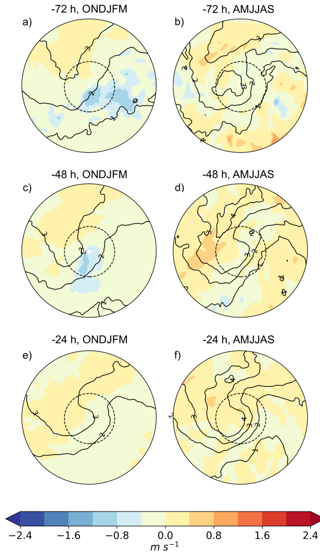
Figure 16. Sensitivity of the maximum 10-m wind gust to the 300-hPa PV (colours, \text{m s}^{-1} ), and the composite mean of 300-hPa PV (contours, 1 PVU interval, 1 PVU = 1.0 \times 10^{-6} \text{ m}^2 \text{ s}^{-1} \text{ K kg}^{-1} ) a,b) 72 h, c,d) 48 h, and e,f) 24 h before the occurrence of maximum 10-m wind gust in Northern Europe. The radius of the plots is 18^\circ and the 6^\circ radius is marked with a dashed circle.
