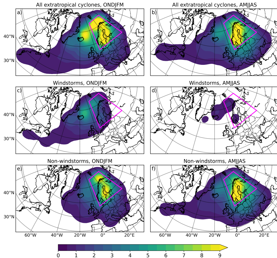
Figure 4. Genesis density (number of cyclones per month per 5^\circ spherical cap \approx 10^6 km 2 ) of a,b) all extratropical cyclones, c,d) windstorms, and e,f) non-windstorms. The magenta box shows the Northern Europe box where the tracks in this study are filtered to occur.
