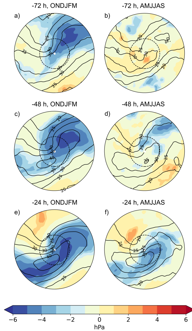
Figure 11. Sensitivity of the minimum MSLP to the 300-hPa wind speed (colours, hPa), and the composite mean of 300-hPa wind speed (contours, 5 \text{ m s}^{-1} interval) a,b) 72 h, c,d) 48 h, and e,f) 24 h before the occurrence of the minimum MSLP. The radius of the plots is 18^\circ and the 6^\circ radius is marked with a dashed circle.
