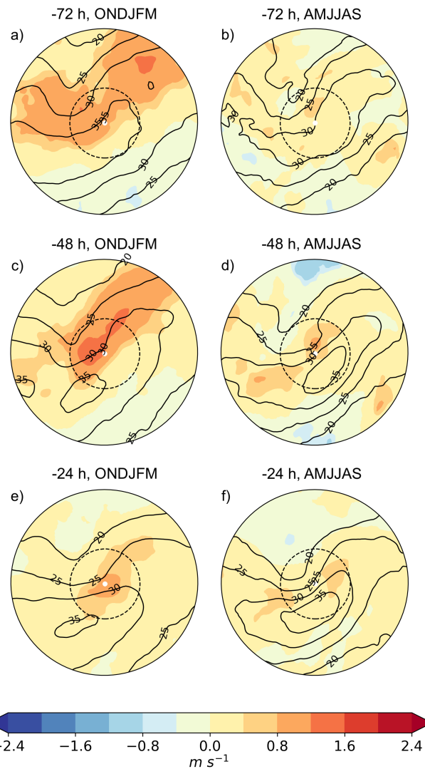
Figure 15. Sensitivity of the maximum 10-m wind gust to the 300-hPa wind speed (colours, m s^{-1} ), and the composite mean of 300-hPa wind speed (contours, 5 m s^{-1} interval) a,b) 72 h, c,d) 48 h, and e,f) 24 h before the occurrence of maximum 10-m wind gust in Northern Europe. The radius of the plots is 18^\circ and the 6^\circ radius is marked with a dashed circle.
