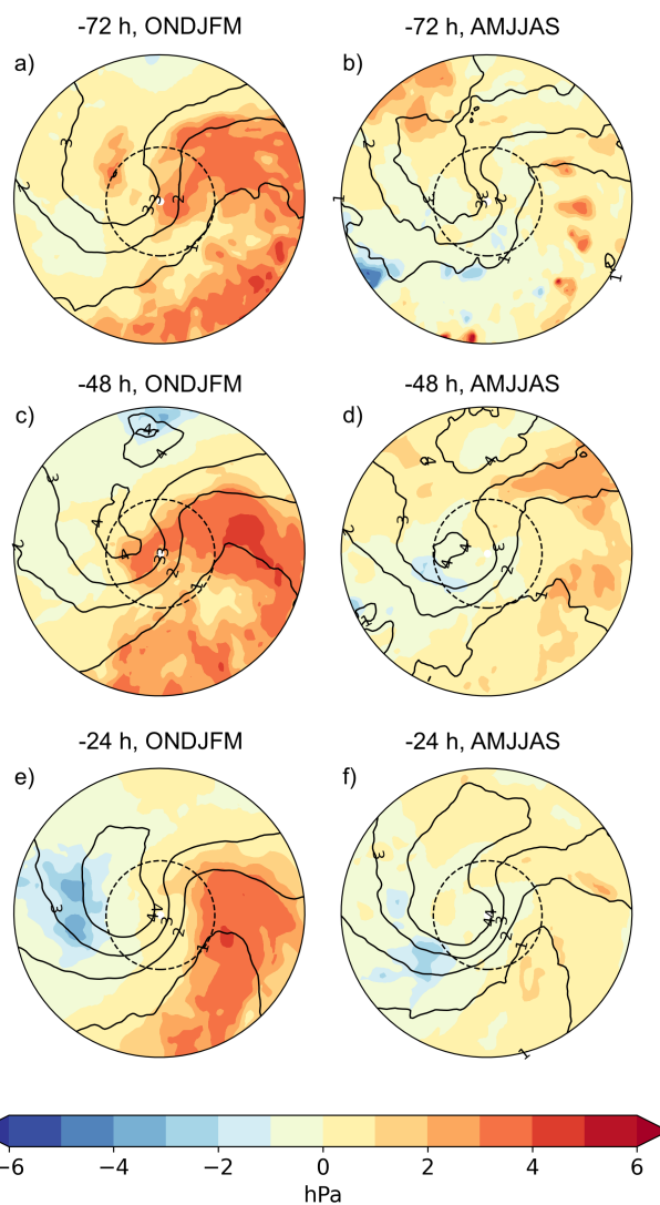
Figure 12. Sensitivity of the minimum MSLP to the 300-hPa PV (colours, hPa), and the composite mean of 300-hPa PV (contours, 1 PVU interval, 1 \text{ PVU} = 1.0 \times 10^{-6} \text{ m}^2 \text{ s}^{-1} \text{ K kg}^{-1} ) a,b) 72 h, c,d) 48 h, and e,f) 24 h before the occurrence of the minimum MSLP. The radius of the plots is 18^\circ and the 6^\circ radius is marked with a dashed circle.
