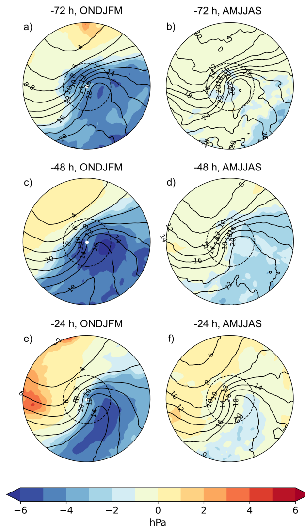
Figure 10. Sensitivity of the minimum MSLP to the TCWV (colours, hPa), and the composite mean of TCWV (contours, 2 kg m -2 interval) a,b) 72 h, c,d) 48 h, and e,f) 24 h before the occurrence of the minimum MSLP. The radius of the plots is 18° and the 6° radius is marked with a dashed circle.
