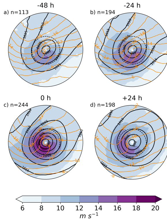
Figure 8. The maximum 10-m wind gust (colours, \text{m s}^{-1} ), mean sea level pressure (black contours, 5 hPa interval) and 850-hPa potential temperature (orange contours, 2 °C interval) composites of windstorms during the warm season (April–September). The offset times are relative to the time of the minimum mean sea level pressure: a) -48 h, b) -24 h, c) 0 h, and d) +24 h. The number in each panel is the number of individual windstorms in each composite. The radius of the plots is 18° and the 6° radius is marked with a dashed circle.
