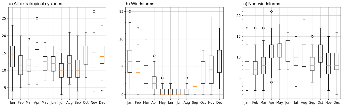
Figure 3. Monthly distribution of cyclones in Northern Europe. Orange lines are medians, boxes show first and third quartiles, and whiskers have first value greater than and last value less than Q1 - 1.5 \cdot IQR and Q3 + 1.5 \cdot IQR , respectively, where Q1 and Q3 are the first and third quartiles and IQR the interquartile range Q3 - Q1 . a) all extratropical cyclones, b) windstorms, and c) non-windstorms.
