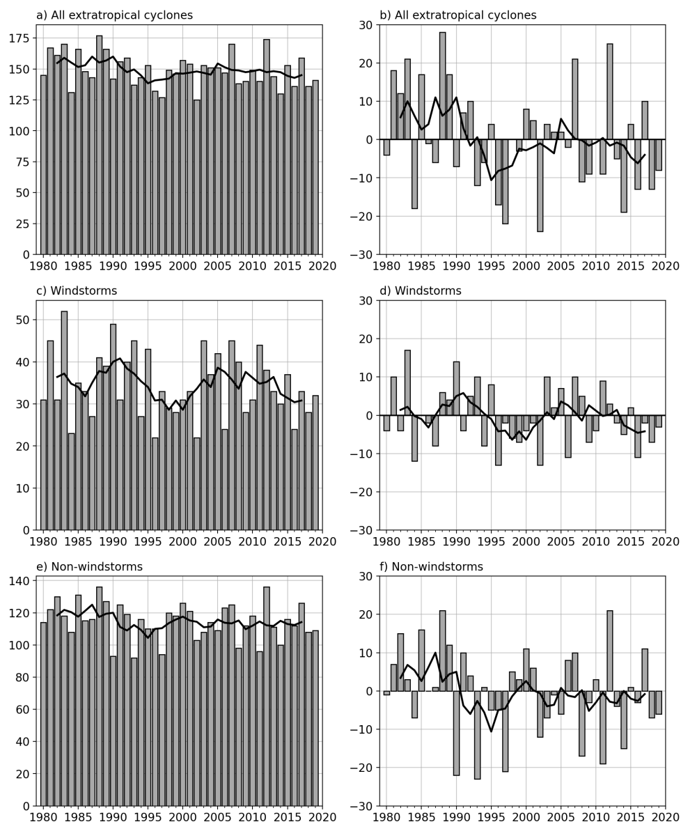
Figure 2. Annual numbers (left column) and absolute anomalies (annual value minus 40-year mean value; right column) of extratropical cyclones in Northern Europe in 1980–2019. Bars show the annual values and lines are 5-year running means. a,b) all extratropical cyclones, c,d) windstorms, and e,f) non-windstorms.
