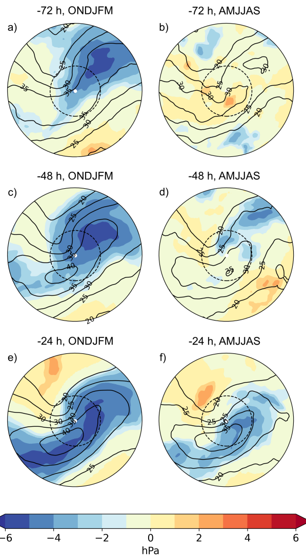
Figure 11. Sensitivity of the minimum MSLP to the 300-hPa wind speed (colours, hPa), and the composite mean of 300-hPa wind speed (contours, 5 \text{ m s}^{-1} interval) a,b) 72 h, c,d) 48 h, and e,f) 24 h before the occurrence of the minimum MSLP. The radius of the plots is 18^\circ and the 6^\circ radius is marked with a dashed circle.
