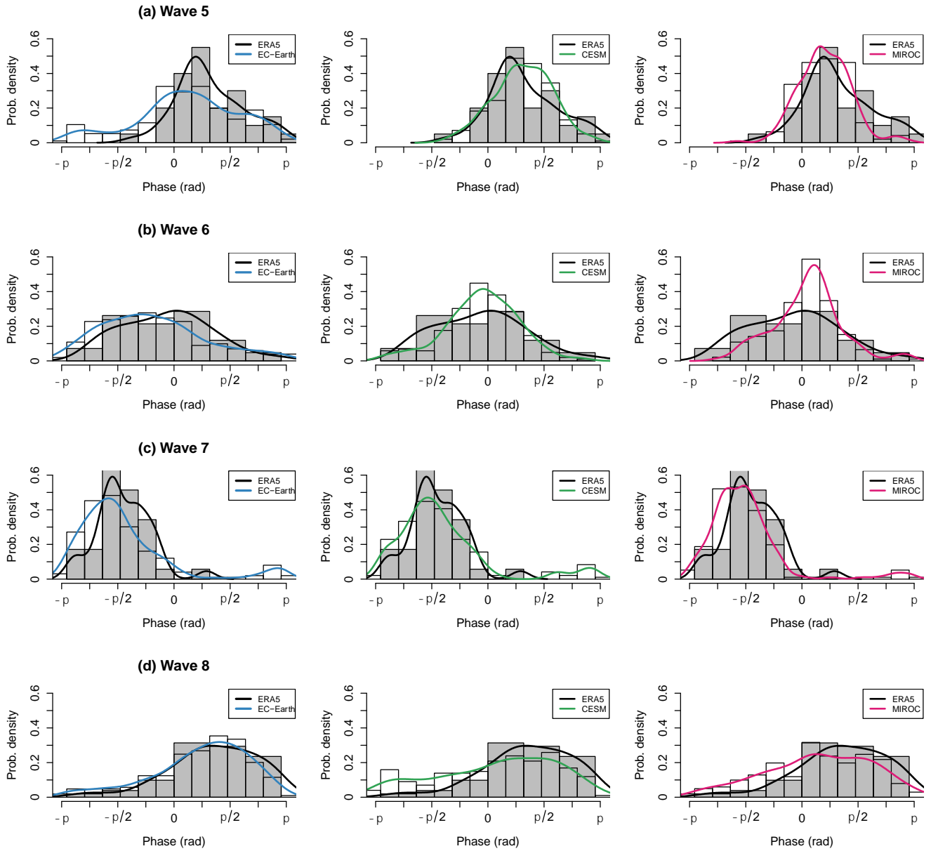
705 Figure B2. Same as Fig.2 but with histogram added.
