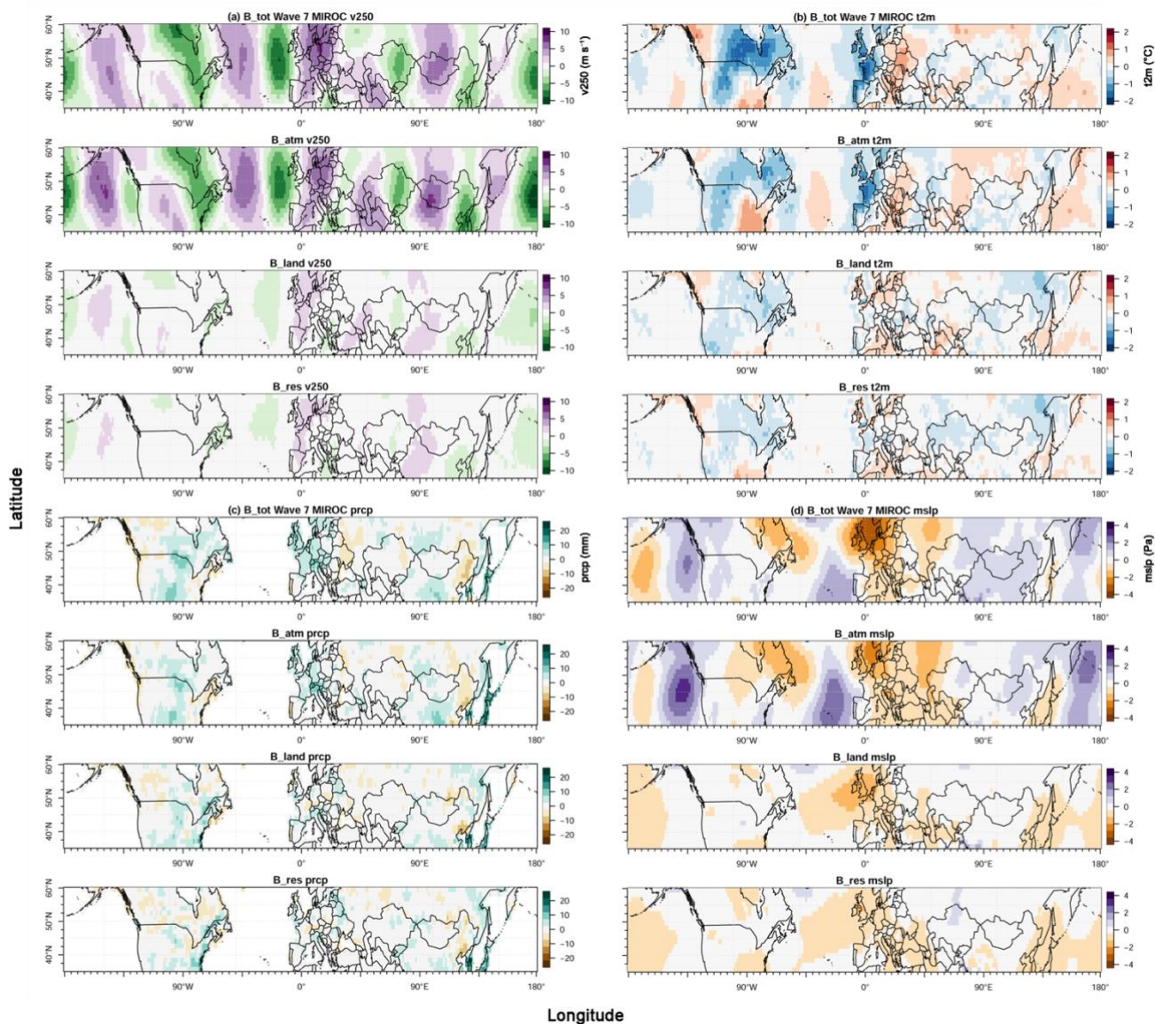
745 Figure B9: Bias plots for high-amplitude wave-7 events and episodes in different experiments for MIROC. Total bias( B_{tot} ), Atmospheric bias( B_{atm} ), Land-Atm interaction bias( B_{land} ) and residual bias( B_{res} ) for meridional wind velocity at 250hPa (a), surface temperature (b), precipitation (c), and sea level pressure (d).
