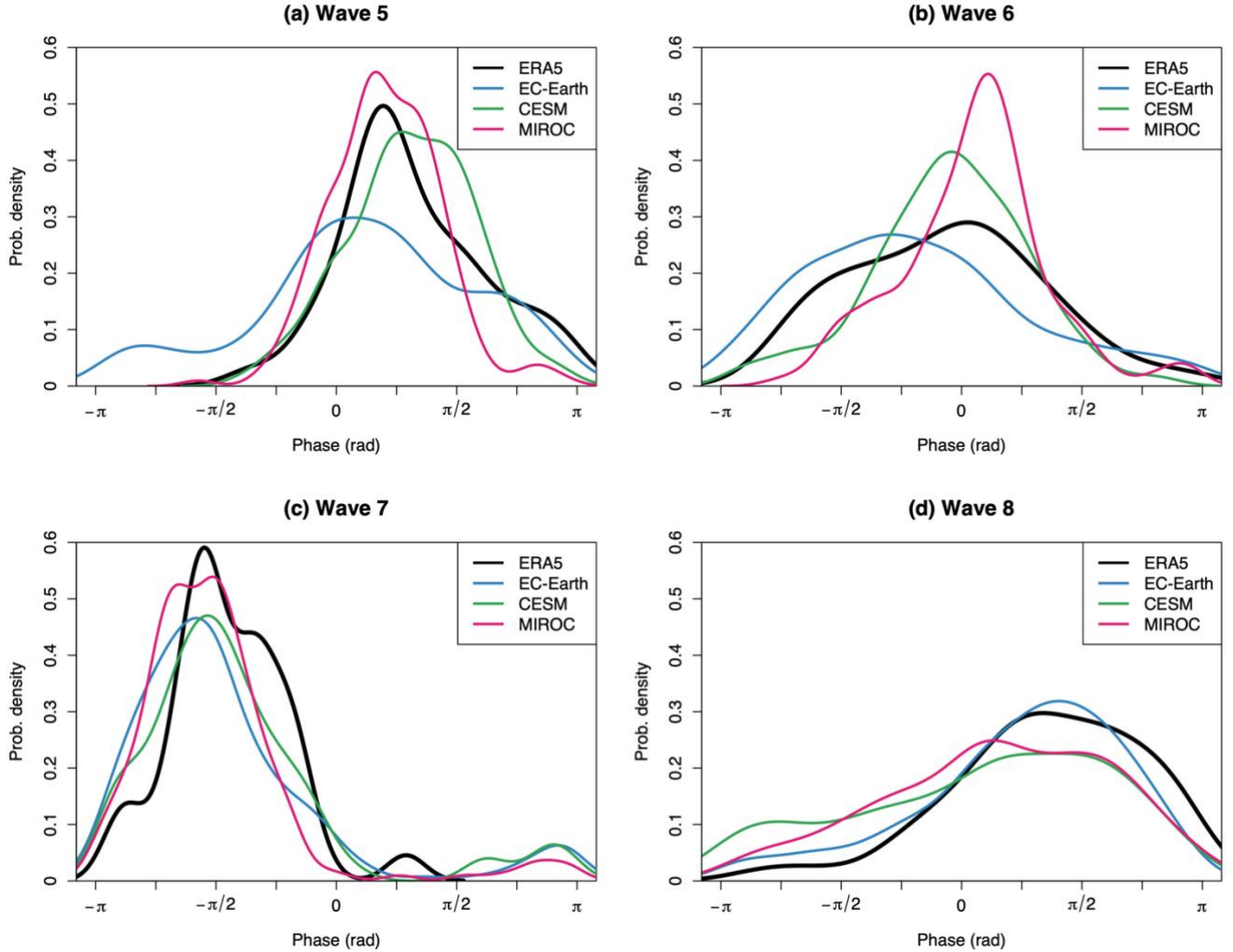
615 Figure 2: Phase-locking of Rossby waves for JJA ERA5 and model waves 5-8 in control run AISI for high wave amplitude episodes (> 1.5 s.d.): (a)-(d), Probability density functions of the phase positions of waves 5-8 in ERA5, EC-Earth, CESM, and MIROC during JJA for the period of 1979-2015/2016 (wave 5 (a), wave 6 (b), wave 7 (c), wave 8 (d)). The bandwidth for ERA5 and models are as follows: (a) Wave 5: 0.35(ERA5), 0.40(EC-Earth), 0.25(CESM), 0.22(MIROC), (b) Wave 6: 0.53(ERA5), 0.45(EC-Earth), 0.30(CESM), 0.25(MIROC), (c) Wave 7: 0.25(ERA5), 0.29(EC-Earth), 0.27(CESM), 0.22(MIROC), (d) Wave 8: 0.49(ERA5), 620 0.39(EC-Earth), 0.52(CESM), 0.46(MIROC).
