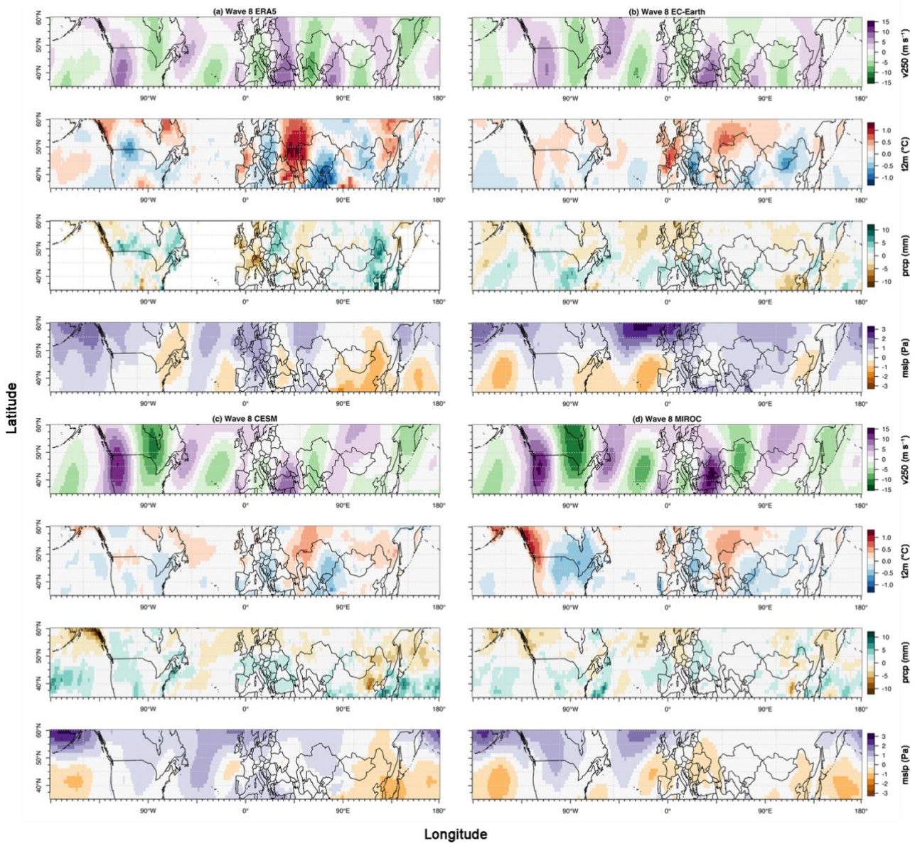
720 Figure B5: Composite anomaly plots of weeks with high-amplitude wave-8 episodes for meridional wind velocity at 250hPa (v250, absolute field), near-surface temperature (t2m, anomaly), precipitation (prcp, anomaly), and sea level pressure (mslp, anomaly) in ERA5 (a), EC-Earth (b), CESM (c) and MIROC (d) based on control runs AISI.
