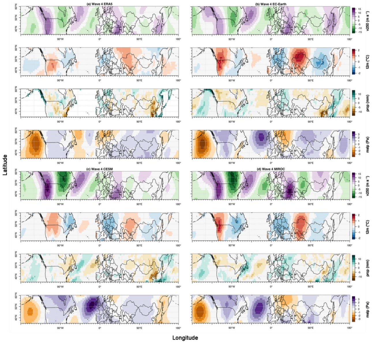
710 Figure B3: Composite anomaly plots of weeks with high-amplitude wave-4 episodes for meridional wind velocity at 250hPa ( v_{250} , absolute field), near-surface temperature ( t_{2m} , anomaly), precipitation ( prcp , anomaly), and sea level pressure ( mslp , anomaly) in ERA5 (a), EC-Earth (b), CESM (c) and MIROC (d) based on control runs AISI.
