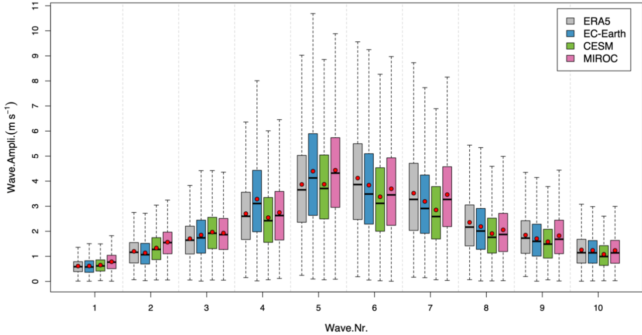
610 Figure 1: Boxplot for wave amplitudes in AISI climatology runs for climate models EC-Earth, CESM, and MIROC, as well as reanalysis data ERA5 for the period of June, July, and August in 1979-2015/2016. Red dots indicate the mean, and thick black lines represent the median. The lower hinge of each box is Q1 quartile (25th), and the upper hinge for Q3 quartile (75th). The upper and lower bars are based on the 1.5 times interquartile range (IQR) value. The outliers are not shown in the plot.
