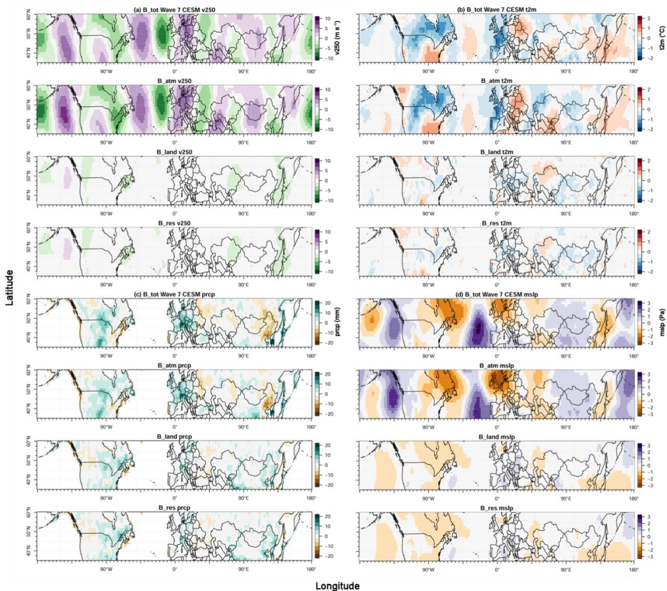
Figure B7: Bias plots for high-amplitude wave-7 events and episodes in different experiments for CESM. Total bias( B_{tot} ), Atmospheric bias( B_{atm} ), Land-Atm interaction bias( B_{land} ) and residual bias( B_{res} ) for meridional wind velocity at 250hPa (a), surface temperature (b), precipitation (c), and sea level pressure (d).
