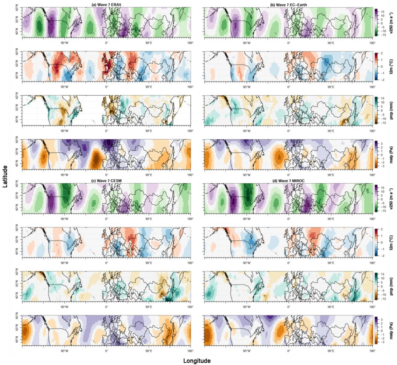
Figure 4: Composite anomaly plots of weeks with high-amplitude waves-7 episodes for meridional wind velocity at 250hPa (v250, absolute field), near-surface temperature (t2m, anomaly), precipitation (prcp, anomaly), and sea level pressure (mslp, anomaly) in ERA5 (a), EC-Earth (b), CESM (c) and MIROC (d) based on control runs AISI.
