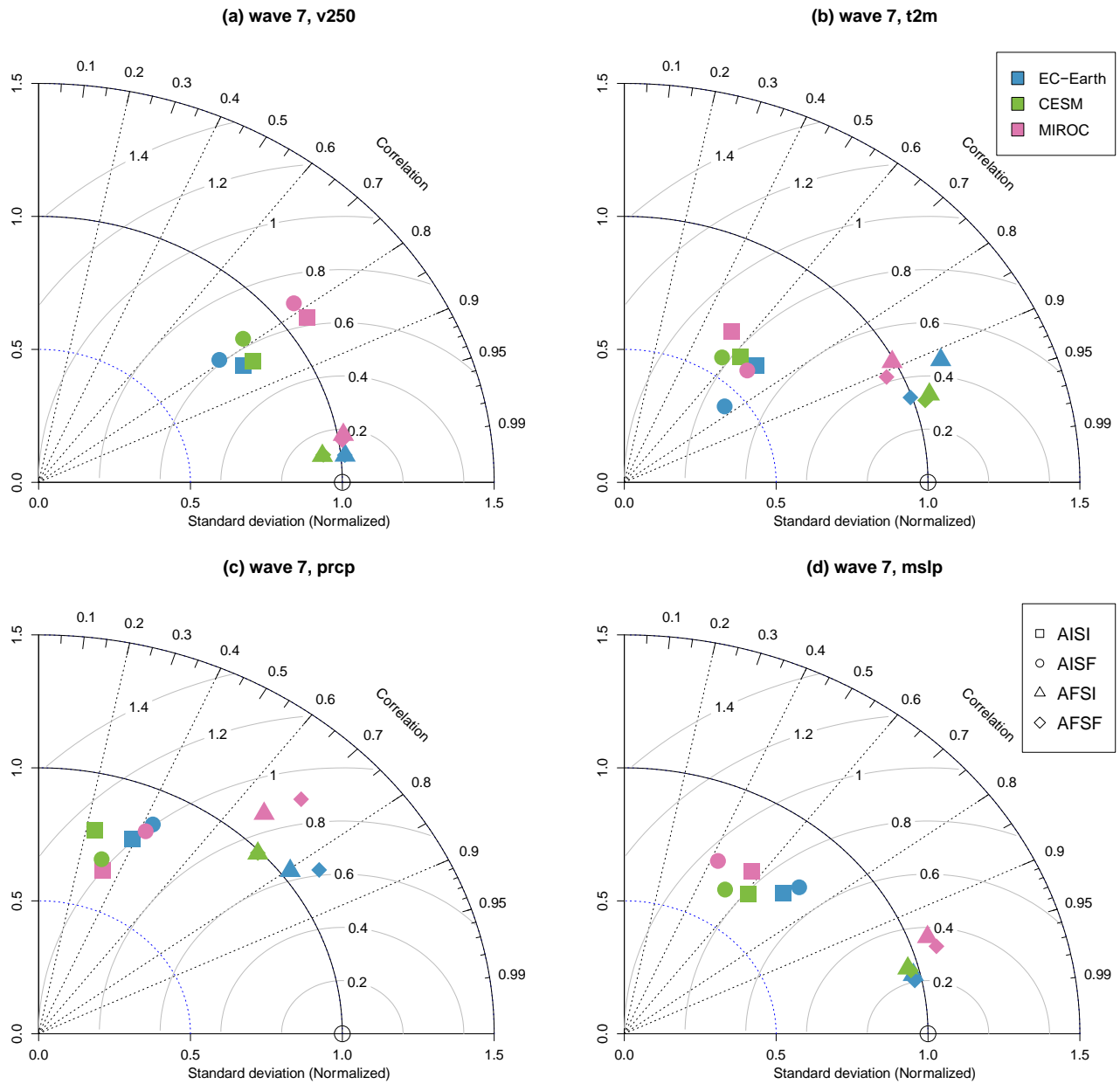
640 Figure 6: Taylor Diagram for all experiments in models compared to ERA5 for wave-7 events and episodes. For a) v250, b) t2m, c) prcp, and d) mslp, the Taylor diagram presents for each model and each experiment, three statistics: the Pearson correlation (dashed lines); the RMS error (grey contours); and the normalized spatial standard deviation (solid black contours).
