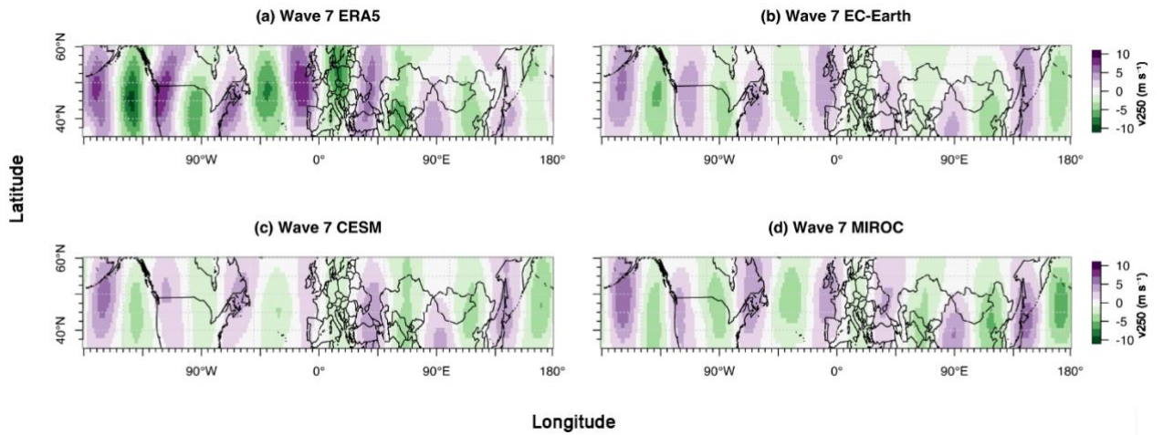
760 Figure B11: Composite anomaly plots of weeks with high-amplitude wave-7 episodes for meridional wind velocity at 250hPa (v250, anomaly) in ERA5 (a), EC-Earth (b), CESM (c) and MIROC (d) based on control runs AISI.
