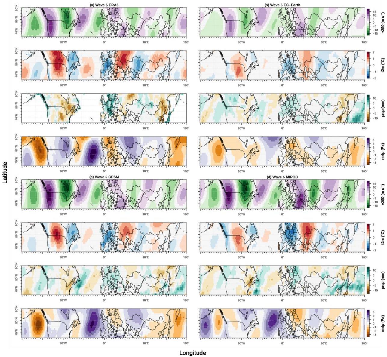
625 Figure 3: Composite anomaly plots of weeks with high-amplitude waves-5 episodes for meridional wind velocity at 250hPa (v250, absolute field), near-surface temperature (t2m, anomaly), precipitation (prcp, anomaly), and sea level pressure (mslp, anomaly) in ERA5 (a), EC-Earth (b), CESM (c) and MIROC (d) based on control runs AISI.
