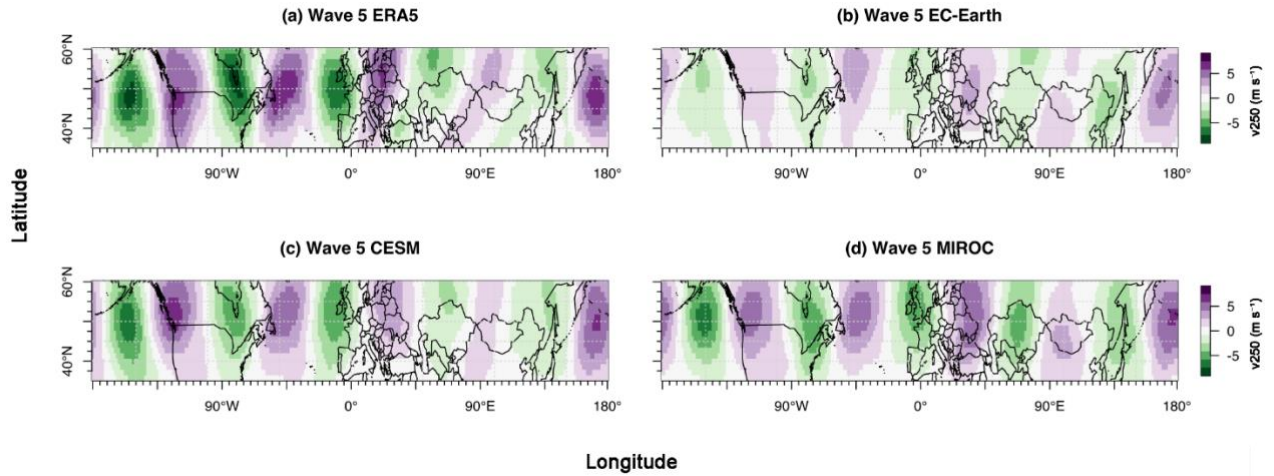
755 Figure B10: Composite anomaly plots of weeks with high-amplitude wave-5 episodes for meridional wind velocity at 250hPa (v250, anomaly) in ERA5 (a), EC-Earth (b), CESM (c) and MIROC (d) based on control runs AISI.
