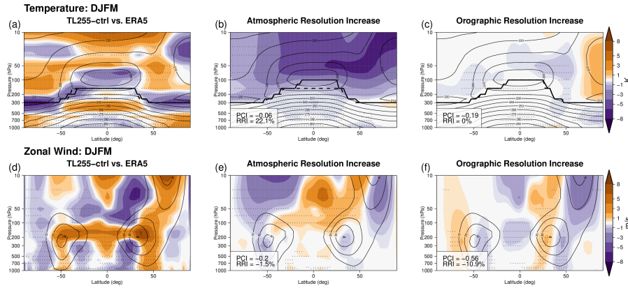
Figure 1. DJFM zonal mean temperature (upper row) and zonal wind (lower row): (a,d) EC-Earth3 TL255-ctrl bias with respect to ERA5, (b,e) changes induced by the atmospheric resolution increase and (c,f) changes induced by the orographic resolution increase. Shading shows differences, contours the TL255-ctrl field. Please note the irregular colorbar spacing. In (a,b,c) black lines show the tropopause height for reference (dashed) and changes (solid). Stippling indicates significance with a Welch t-test at the 1% level. In (b,c,e,f) the PCI and RRI (see text for details) are reported at the bottom left of each panel: large negative values implies reduced bias.
