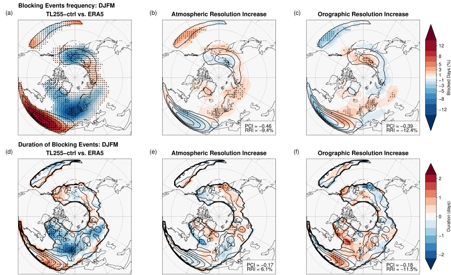
Figure 4. DJFM blocking events frequency (top row) and blocking events duration (bottom row) for (a,d) EC-Earth3 TL255-ctrl bias with respect to to ERA5 (b,e) changes induced by the atmospheric resolution increase and (c,f) changes induced by the orographic resolution increase. Shading shows differences, contours the TL255-ctrl field. For Blocking Events frequency, please note the irregular colorbar spacing. For blocking frequency, contours are drawn every 5%. For blocking duration, contours are drawn every 0.5 days. Stippling indicates significance with a Welch t-test at the 5% level. In (b,c,e,f) the PCI and RRI (see text for details) are reported at the bottom left of each panel: large negative values implies reduced bias.
