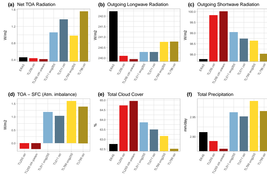
Figure 7. Global yearly-averaged mean (a) net TOA radiation (b) Outgoing Longwave radiation at TOA (c) Outgoing Shortwave radiation at TOA (d) Atmosphere imbalance (e) Total cloud cover (f) Total precipitation in the EC-Earth3 runs. TL511 is shown in blue and TL799 in yellow, with lighter colours indicating orog255 experiments
