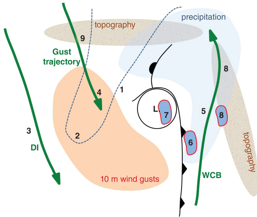
2050 Figure 3: Schematic illustration of possible features related to combined precipitation and wind impact of a cyclone in the Mediterranean, based on the five events studied in Raveh-Rubin and Wernli (2016). Note that this schematic does not represent any individual event, but rather summarizes the variable possible features of importance. The cyclone centre is denoted by the letter 'L', accompanied by a cold and a warm front. Shading shows areas with precipitation impact (light blue), and with 10 m gust impact (light red). Areas with convection (and thus co-located precipitation and wind gust impact) are shaded blue and 2055 encircled by a red line. High topography is represented by grey regions. The 320 K 2-PVU contour is shown as a dashed line and typical WCB, DI and gust trajectories are denoted as green arrows. The numbers mark the location of: (1) a prominent upper- level feature (PV streamer/trough/ridge), (2) tropopause fold and downward momentum transfer, (3) DI trajectories around high gusts, (4) low-level gust trajectory, (5) WCB slantwise ascent associated with precipitation, (6) convective precipitation at cold front, (7) convective precipitation in cyclone centre, (8) orography enhancing precipitation (and/or convection), (9) orography 2060 accelerating gust trajectories. Reprinted from Raveh-Rubin and Wernli (2016) with permission.
