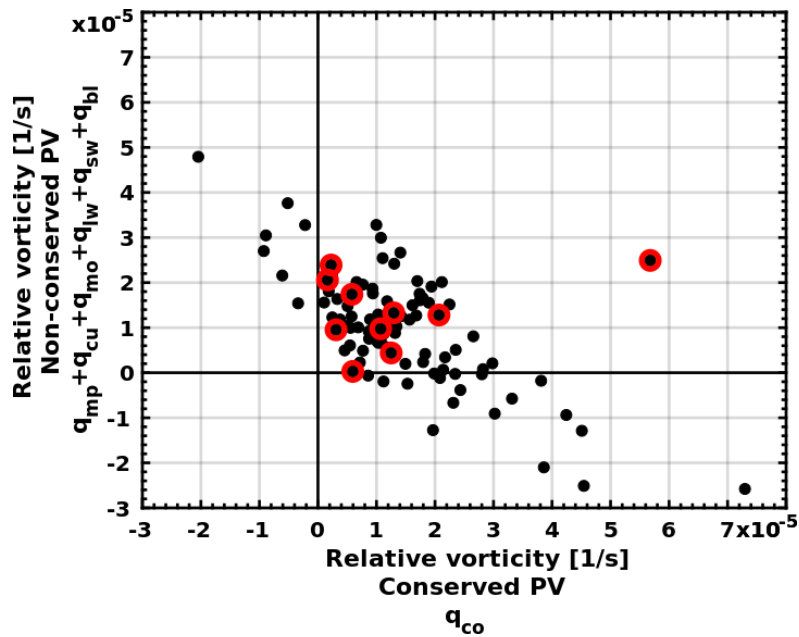
Figure 4: Scatterplot relating the contribution of different PV sources to the relative vorticity at 850 hPa, in the centre of 100 intense cyclones: Contributions of conserved, adiabatically transported PV is shown in the x-axis and non-conserved, diabatically-produced PV is shown in the y-axis. Red circles depict ten medicane cases. Reprinted from Flaounas et al. (2021).
