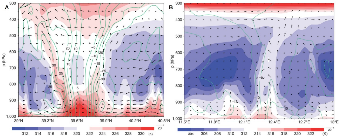
Figure 5: (a) The October 1996 case: Vertical cross-section of \theta_e (colours), storm-relative winds (vectors), absolute momentum (lines, contour interval=5m/s; zero not shown) near the cyclone centre (longitude=12.45°E) (WRF-model run, 3 km grid spacing), at 1000 UTC 9 October 1996; (b) as in (a), but for the December 2005 case (latitude = 34.1°N; 0600 UTC 15 December 2005.. The wind vectors are drawn every five grid points in the horizontal. Typical TC features can be identified, such as upward motion along isosurfaces of absolute momentum, large-scale moisture convergence in low levels, and near moist-neutrality for ascending particles. Reprinted from Miglietta and Rotunno (2019) with permission.
