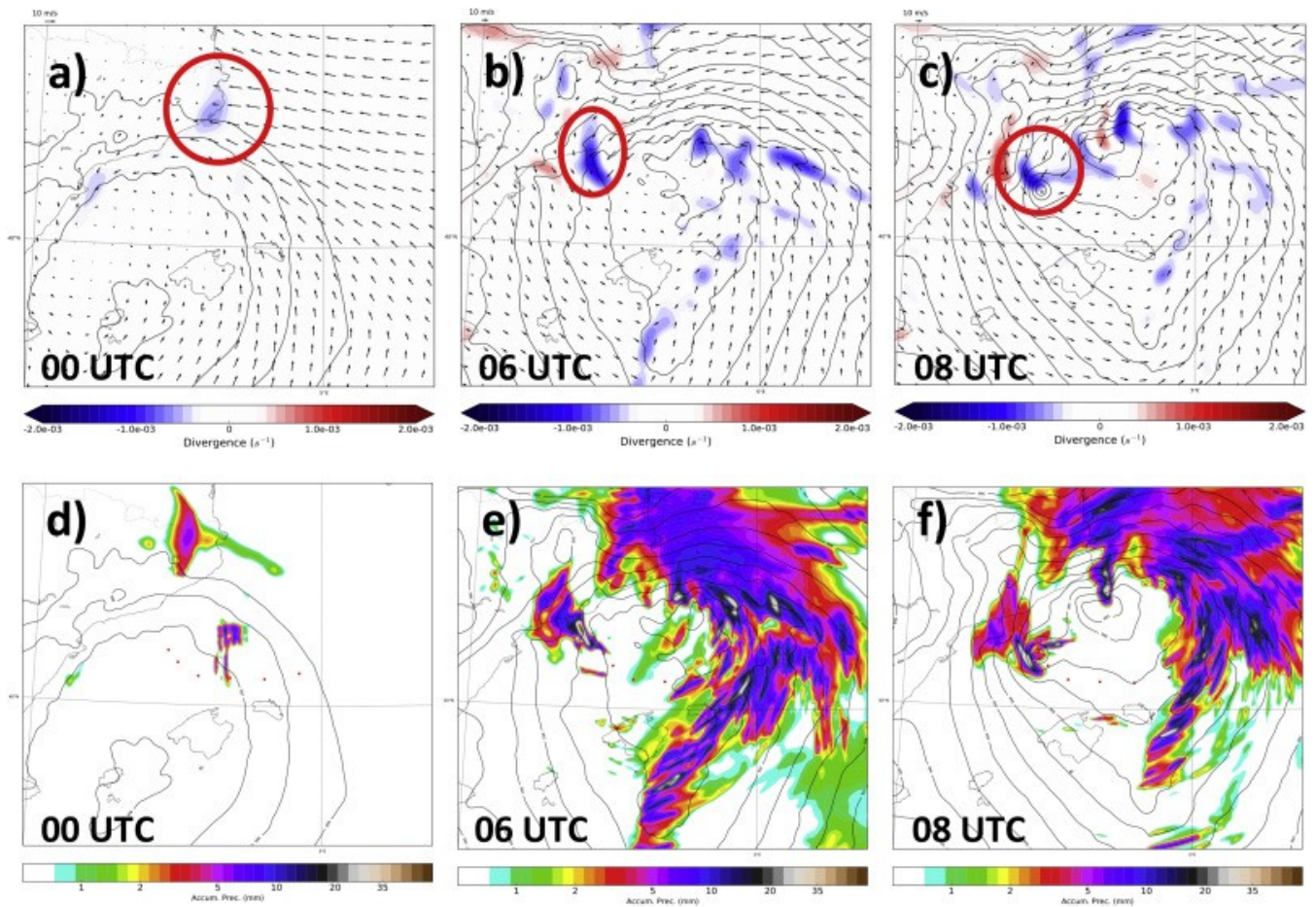
2090 Figure 7: Control surface divergence, horizontal winds and mean sea level pressure (a-c) and hourly accumulated precipitation together with mean sea level pressure (d-f) depicted at a-d) 00, b-e) 06 and c-f) 08 UTC on 31 October 2012. Red circle highlights locations of low-level convergence associated with triggering of the secondary cyclone. Reprinted from Carrio et al. (2020).
