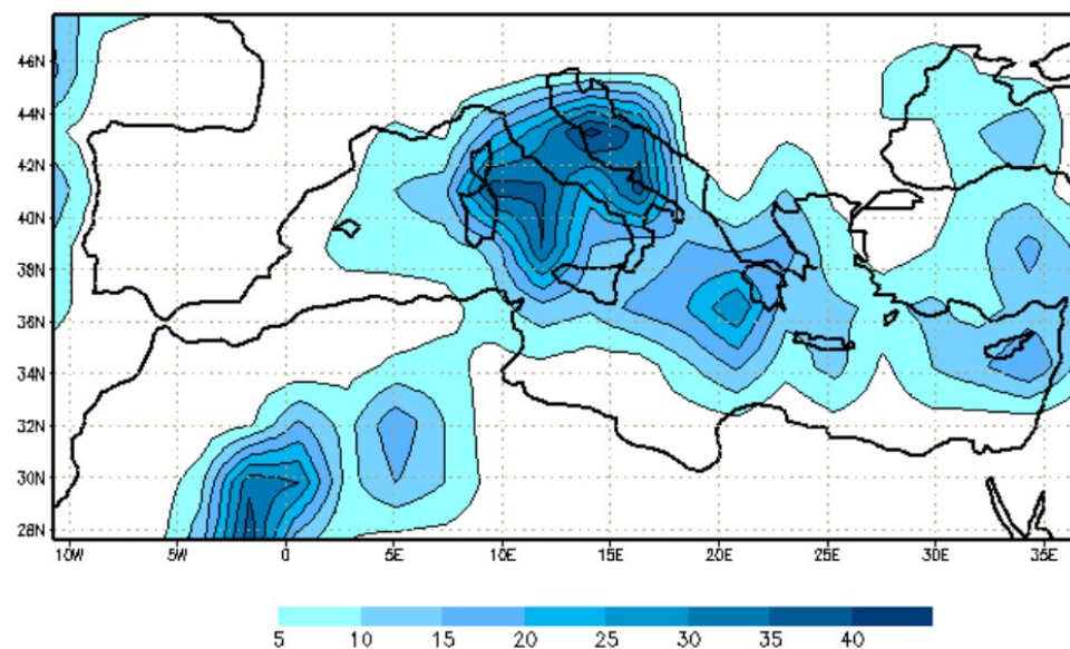
2040 Figure 1: Number of intense cyclones over the 45 years ERA-40 period at mature stage per squares of 2.25^\circ \times 2.25^\circ . Reprinted from Homar et al. (2007).
