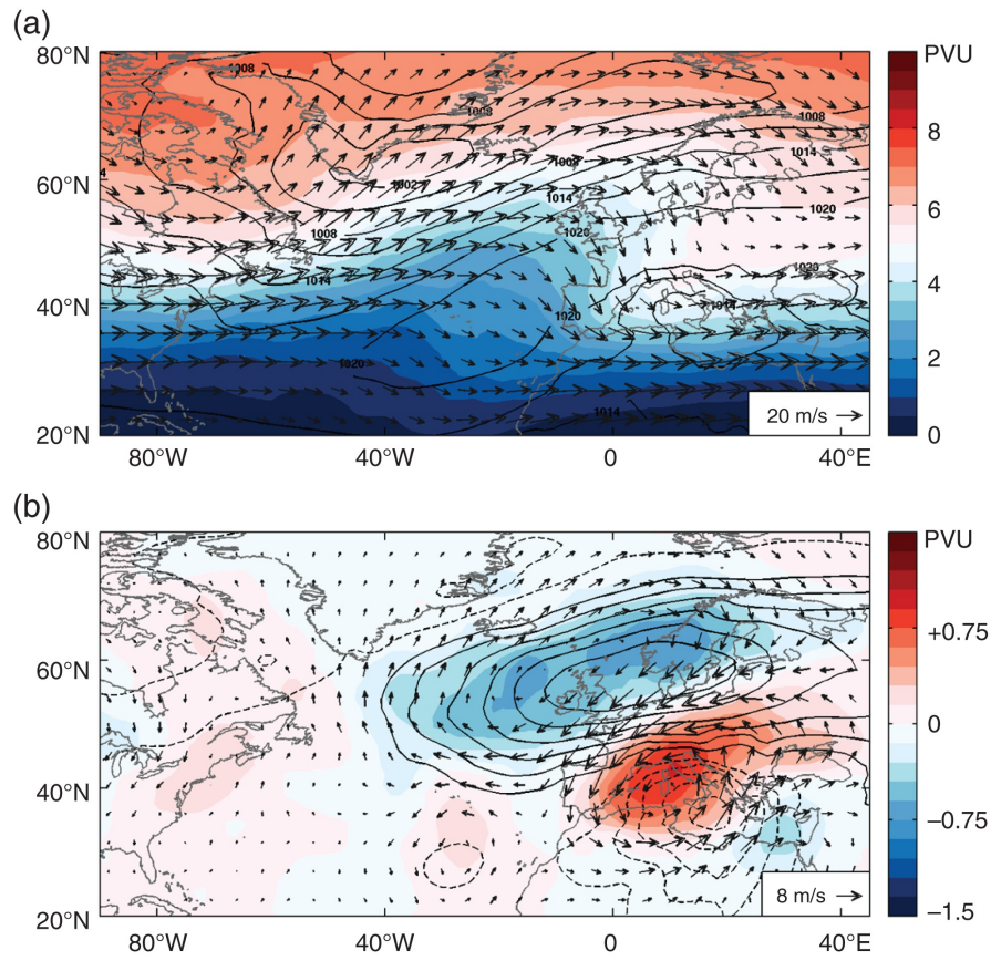
Figure 2: (a) ERA-Interim average fields of sea-level pressure (black contours), PV (shaded), and wind (arrows) on the 330-K isentropic surface, centred at the time of maximum intensity of the 200 Mediterranean cyclones. (b) as (a) but for monthly anomalies (contours every 1 hPa, dashed for negative and solid for positive values). Reprinted from Raveh-Rubin and Flaounas (2017).
