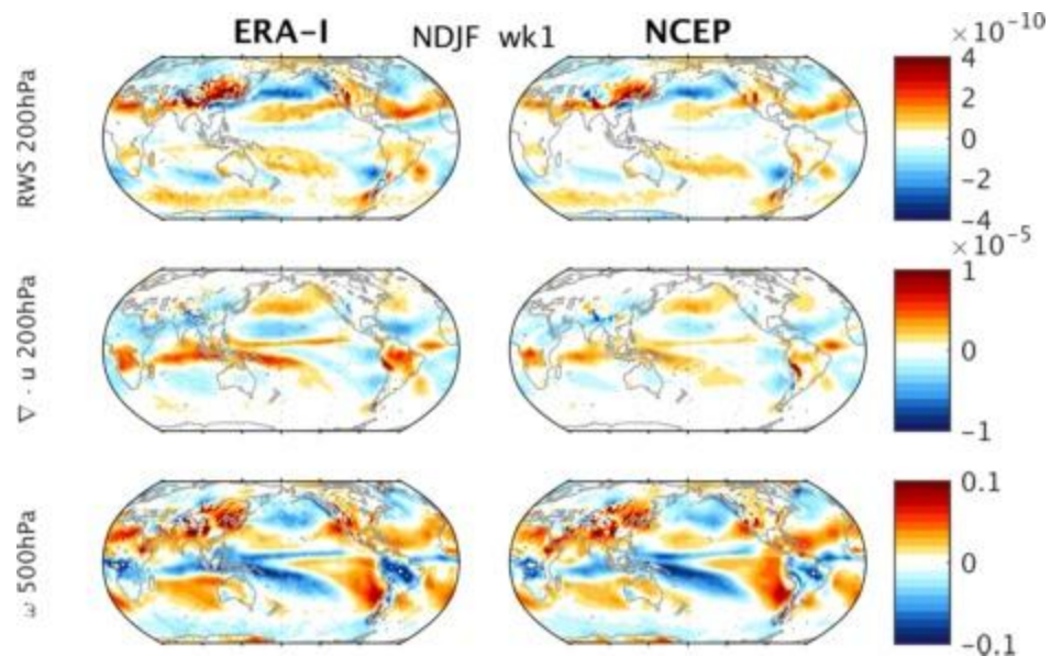
Figure R1. Left column, from top to bottom: week 1 200 hPa Rossby wave source, 200 hPa wind divergence, 500 hPa \omega during NDJF; right column: same as left column but for the NCEP model
