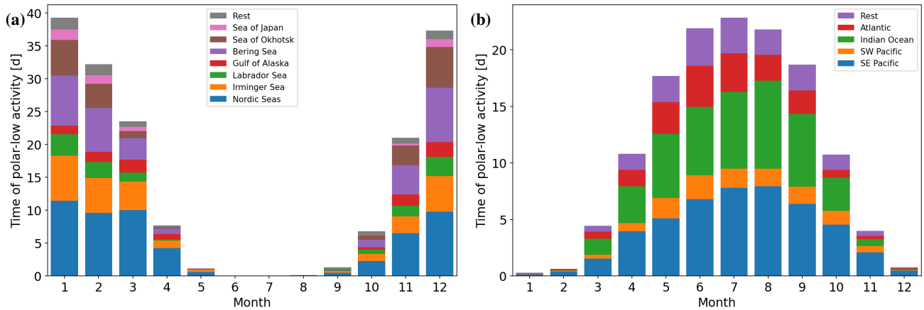
Figure 4. The average monthly time of polar-low activity normalised to months with a duration of 30 days for (a) the Northern and (b) the Southern Hemisphere. Note that two polar-lows occurring simultaneously are counted twice to Given the typical polar-low lifetime of around 24 h, one day of activity represents approximately one polar low. Colours denote the contribution of specific regions marked by boxes in Figure 3.
