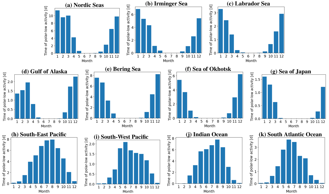
Figure 5. The average monthly time of polar-low activity normalised to months with a duration of 30 days for the specific regions marked by boxes in Figure 3.
