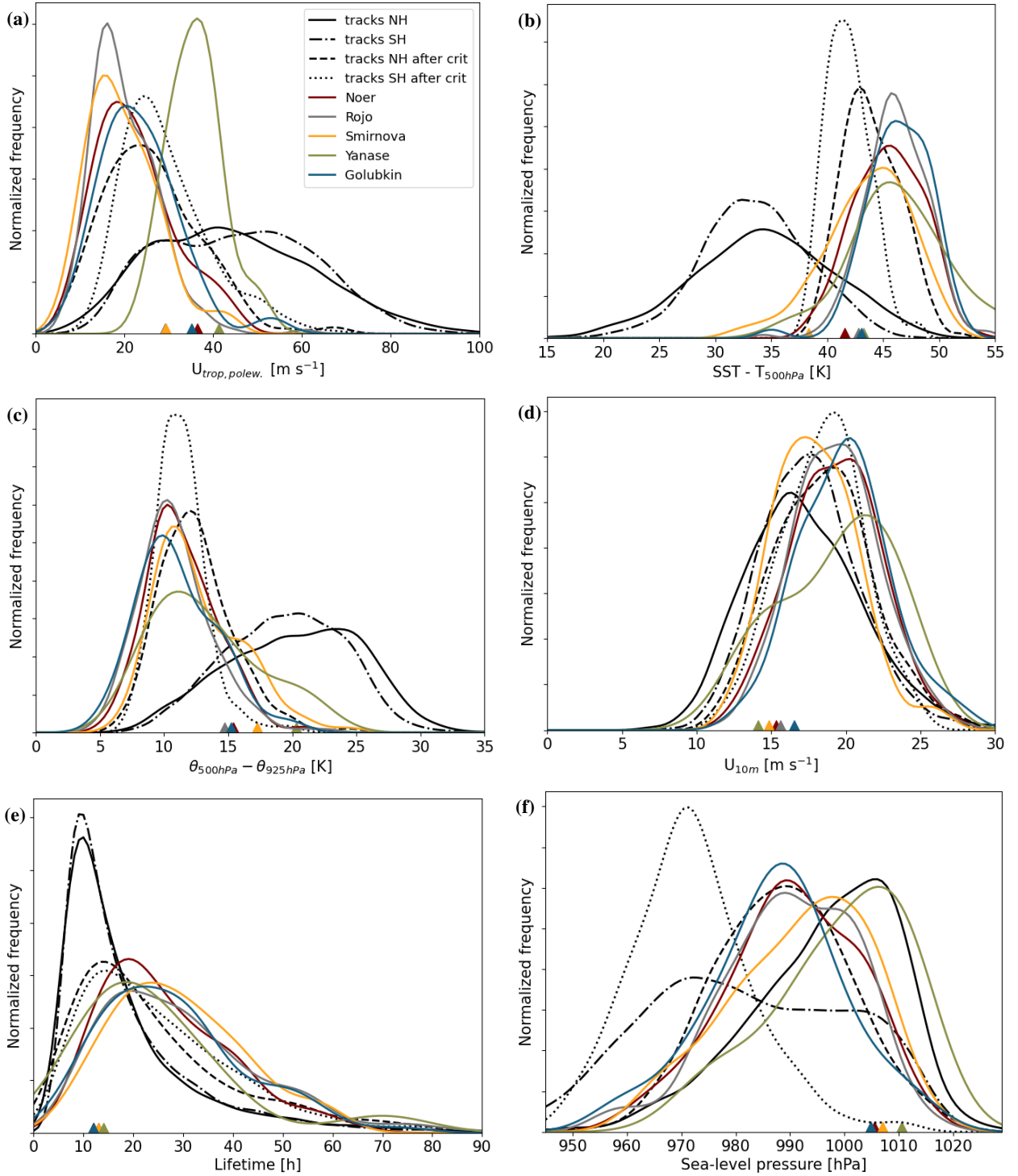
Figure 2. As Figure 1, the distribution in different parameters parameter distributions for polar lows from the lists (colours), all cyclone tracks of the Northern and Southern Hemisphere (black), different polar-low lists (colours) and in the cyclone tracks that remain after application of the four polar-low criteria for the two hemispheres (black dotted and dash-dotted dashed).
