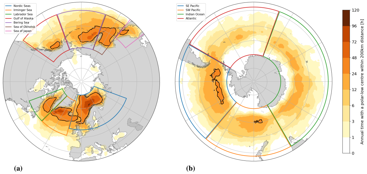
Figure 3. Annual mean density of polar-low activity, measured by the amount of polar-low time steps within a 200 km distance, which is a typical radius of a polar low, for (a) the Northern and (b) the Southern Hemisphere. Note the logarithmic colour scale towards low densities. A black contour encircles regions with an activity of more than 24 h per year, which means that a given location is affected by a polar low with a typical duration of one day approximately once per year.
