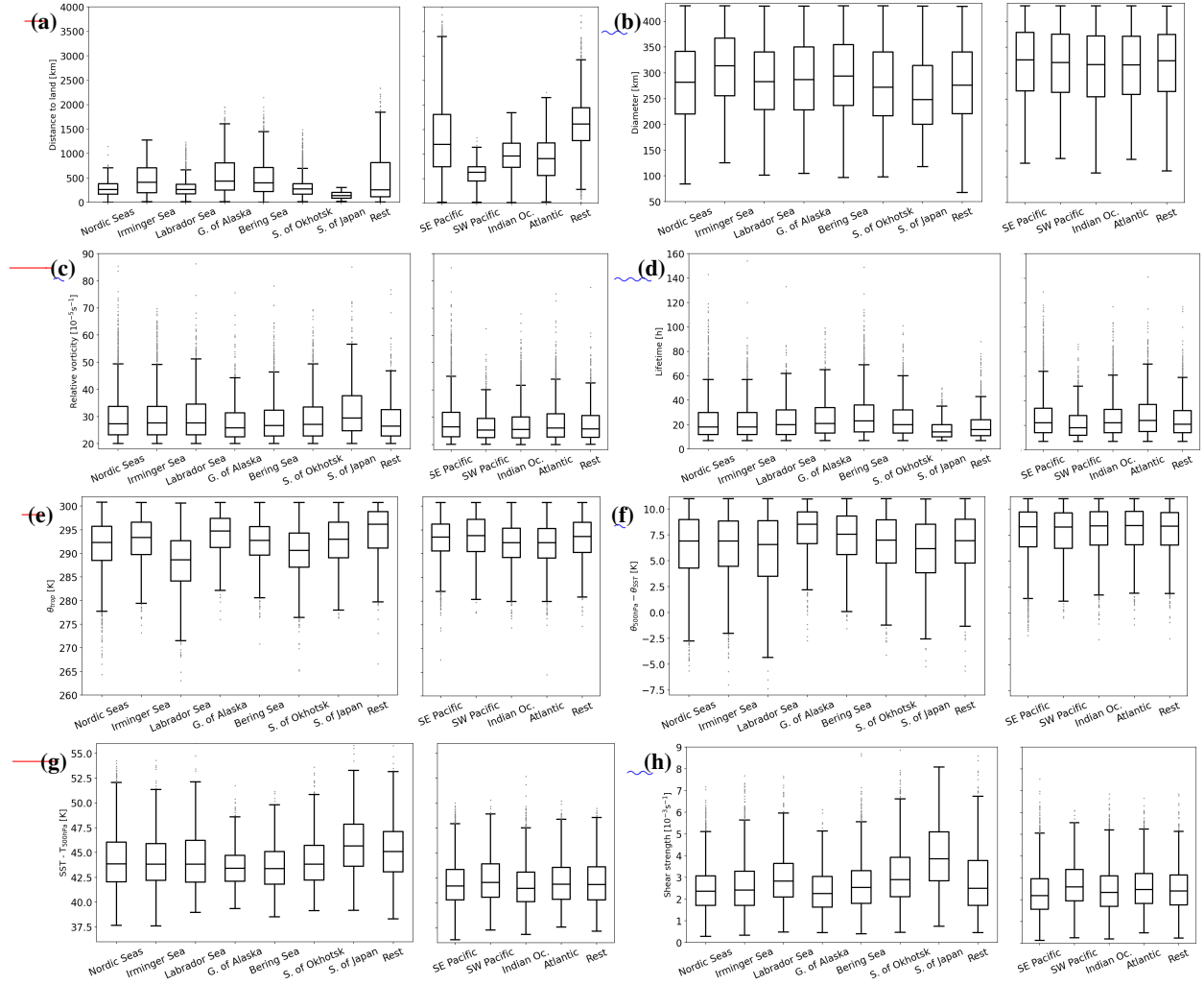
Figure 7. Parameter distributions of polar lows for the different regions. For The lifetime-maximum of the polar-low tracks is used for computation of (a) the distance to land, (b) the vortex diameter, (c) the relative vorticity, (g) SST - T_{500hPa} , and (h) the shear strength the lifetime-maximum of the polar-low tracks is computed . For (e) \theta_{trop} the lifetime-mean, and for (f) \theta_{500hPa} - \theta_{SST} the lifetime-minimum is calculated. (d) The lifetime is the duration of the polar low.
