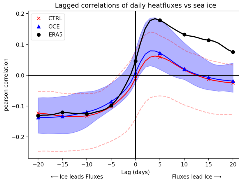
Figure 10. Lagged correlations of the daily BKS heat fluxes against daily BKS sea ice for ERA5, black dotted (resp. CTRL, red crosses, and OCE, blue triangles). Negative lags correspond to the ice forcing heat fluxes, and vice versa for positive lags. Note that positive heat flux values correspond to an upwards flux. redCorrelations are computed using all days in November through February, 1980-2015. Blue shading indicates the ensemble spread of OCE; the CTRL spread is indicated by red stipled lines. Note that only every 5th point has been marked by a symbol for visual clarity.
