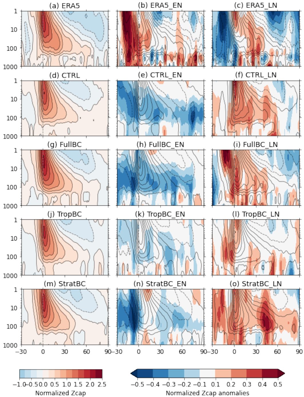
Figure 6: SSW response of normalized polar cap (60°N-90°N) geopotential height, composited around SSW day zero (shown as dashed vertical grey line). Left column shows neutral years for the experiments and all years for ERA5. Middle column shows SSW response in El Niño years with contours (negative values dashed) and the El Niño anomalous SSW response in colours (normalized polar cap geopotential height in El Niño years minus neutral years). Right column is the same for La Niña. ERA5 data from 1979-2019, 100 years for each model run (neutral, El Niño, and La Niña).
