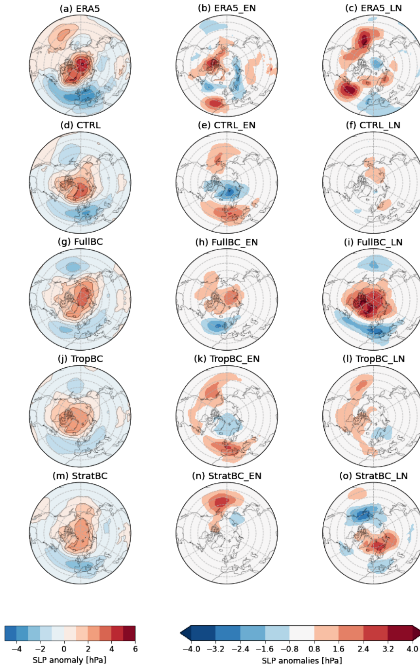
Figure 8: Left column: Composites of absolute SLP anomalies averaged over 30 days after the central dates of SSWs, for neutral ENSO conditions for the models and all years for ERA5. Middle and right column show difference between SLP anomalies during El Niño (middle) and La Niña (right), minus neutral condition anomalies. ERA5 data from 1979-2019, 100 years for each model run (neutral, El Niño, and La Niña).
