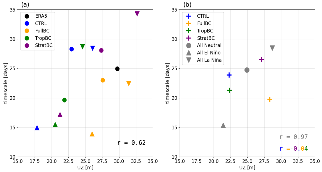
DJF UZ and 150-50hPa mean timescales of variability
