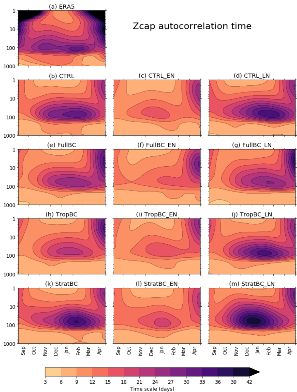
Figure 2: Time-scales of polar cap (60°N-90°N area average with cosine weighting) geopotential height (Zcap) variability. The timescales are defined as days when the autocorrelation function drop to 1/e. The timeseries are smoothed in time with a Gaussian filter ( \sigma = 26 days), following Fig. 1 from Baldwin et al. 2003. ERA5 data from 1979-2019, 100 years for each model run (neutral, El Niño, and La Niña).
