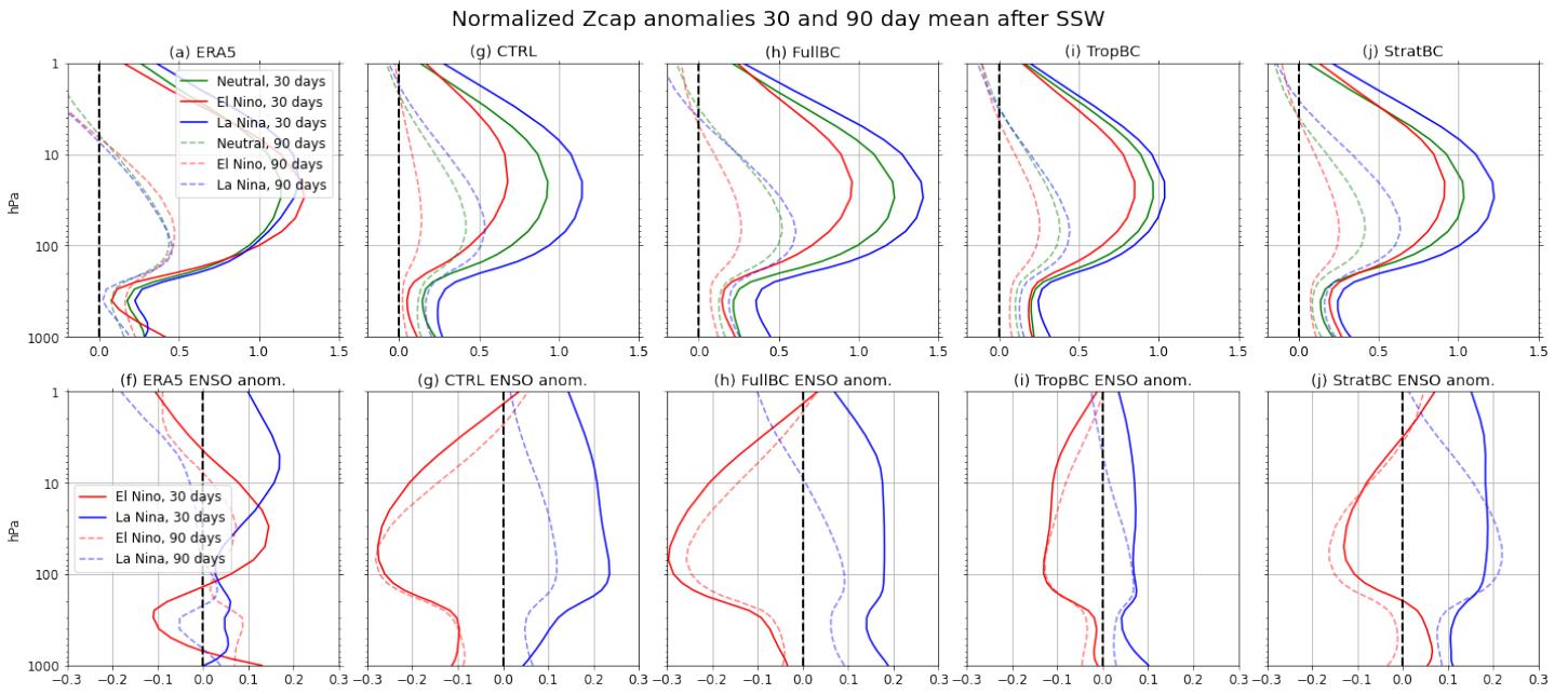
Figure 7: Top row; Normalized polar cap (60°N-90°N) geopotential height, composited around day zero of and time-averaged for 30 and 90 days after SSWs, for neutral years (green), El Niño years (red) and La Niña years (blue). Bottom row shows the change in the mean Zcap SSW difference from neutral years due to El Niño (red) and La Niña (blue)
