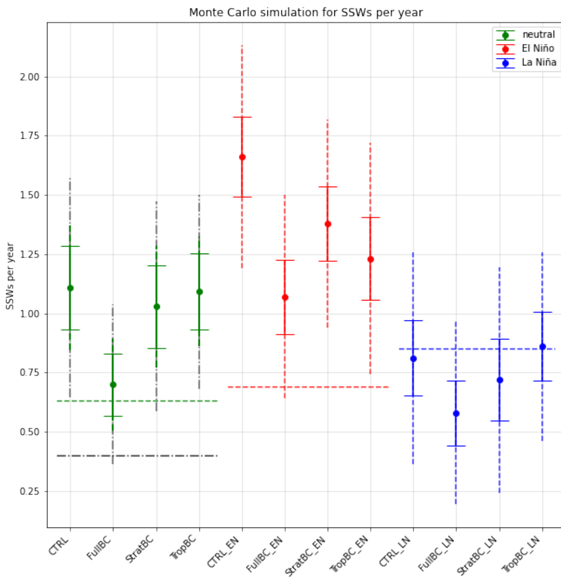
Figure 4: Estimates of variability for number of SSWs per year using Monte Carlo simulations (N=10000). The horizontal dashed lines show the ERA5 SSWs per year (green is all 41 years, black dot-dashed is 15 neutral years, red is 13 El Niño years, blue is 13 La Niña years). Solid error bars show the 5th-95th percentile for Monte Carlo simulation choosing 100 random years from each 100 year simulation. Dashed error bars show the 5th-95th percentile for Monte Carlo simulations where the number of years chosen matches the number of years in ERA5 (green: all 41 years, black dot-dashed: 15 neutral years, red: 13 El Niño years, blue: 13 La Niña years).
